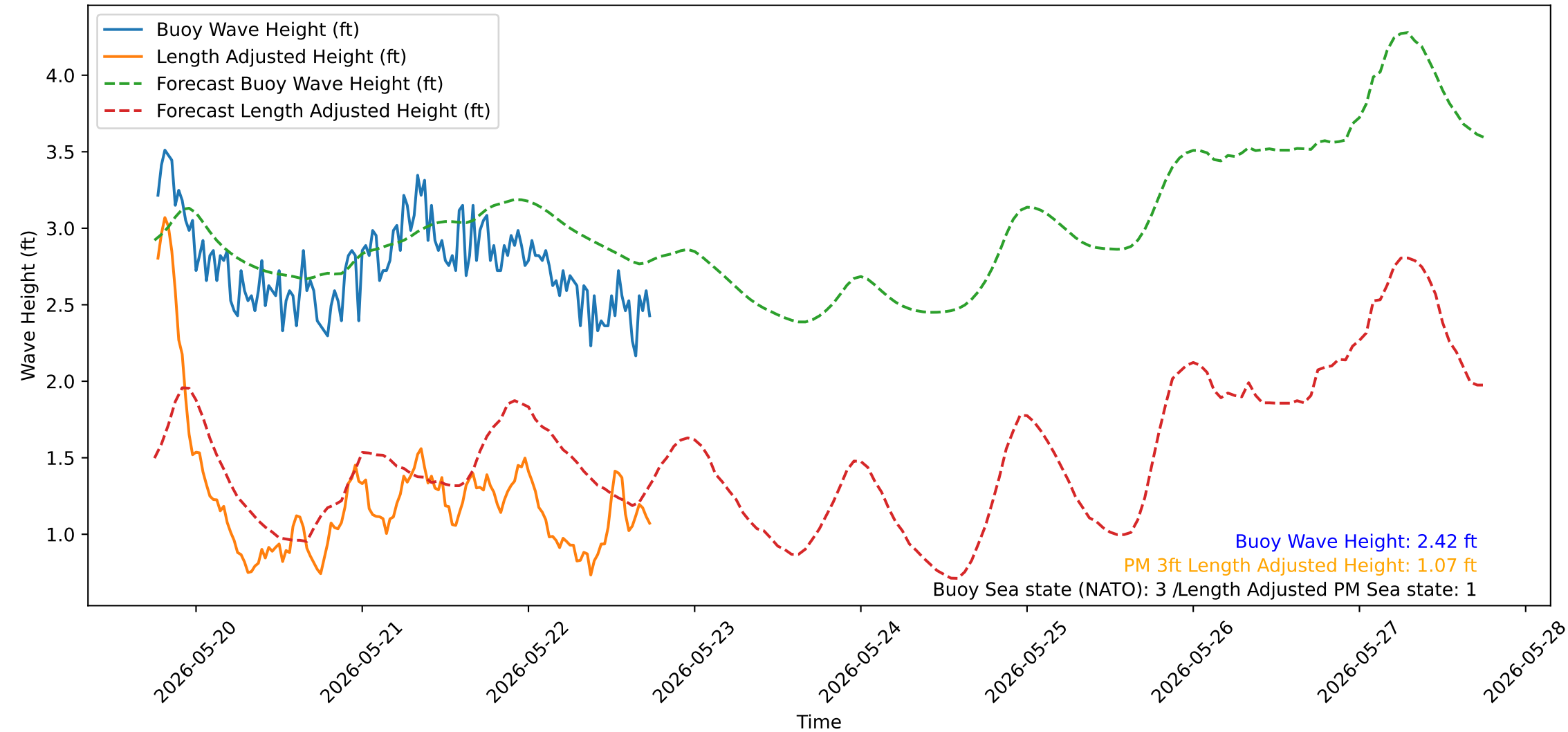
Wave Heights over Time for Red Beach at 2026-05-22 18:20:53
