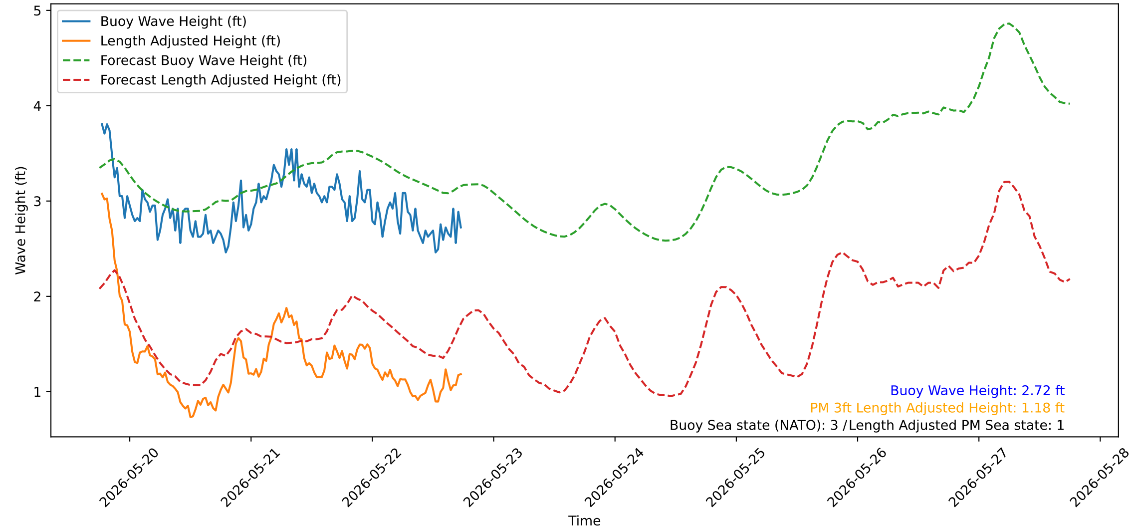
Wave Heights over Time for Green Beach at 2026-05-22 18:21:15
