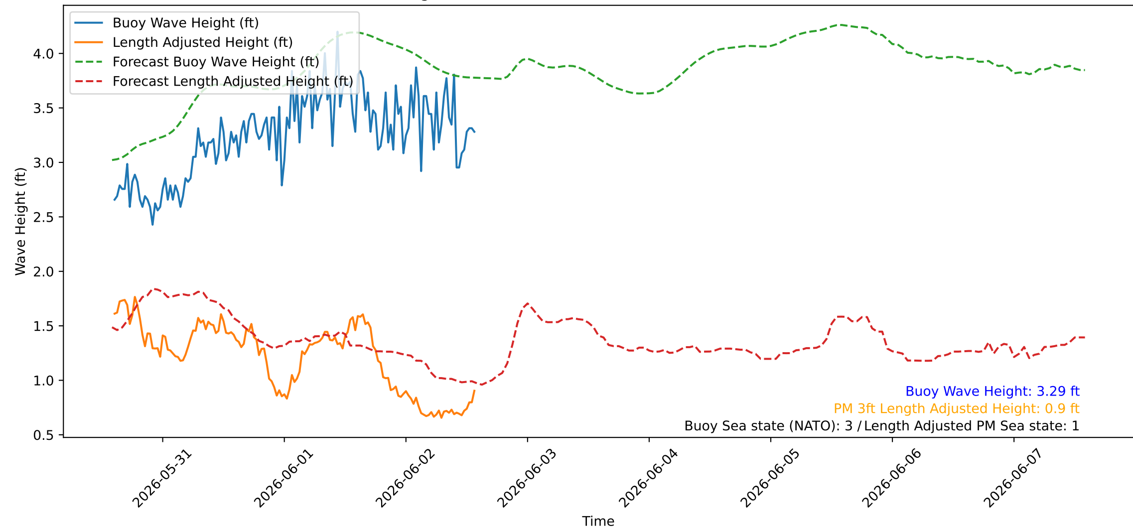
Wave Heights over Time for Red Beach at 2026-06-02 14:20:46
