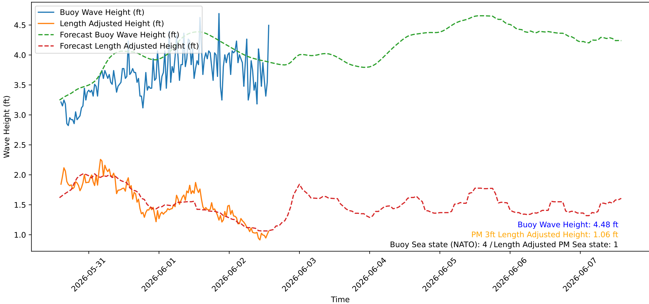
Wave Heights over Time for Oceanside Harbor at 2026-06-02 14:20:26
