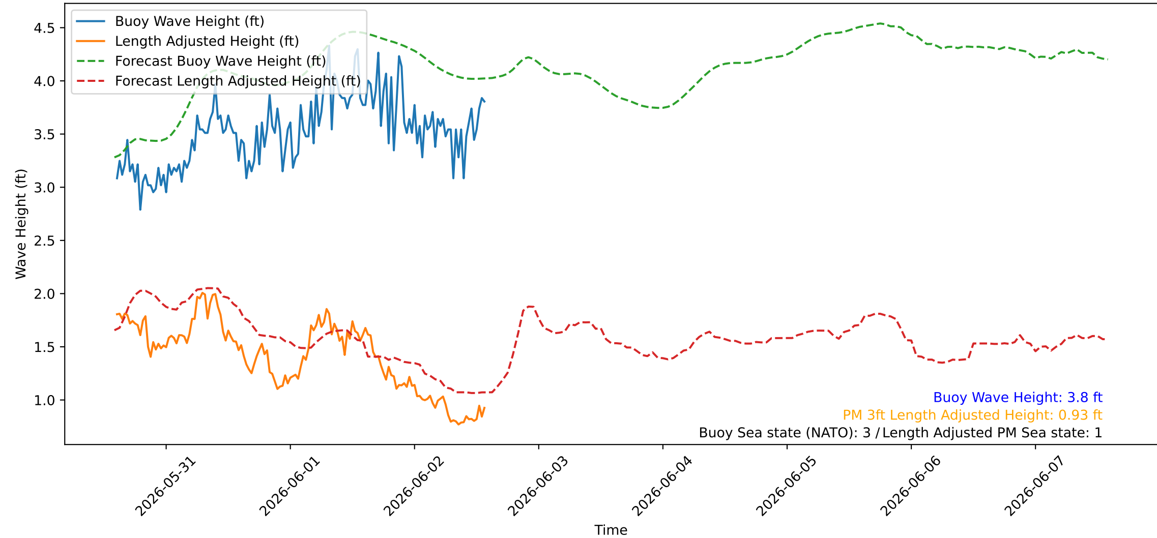
Wave Heights over Time for Green Beach at 2026-06-02 14:21:09
