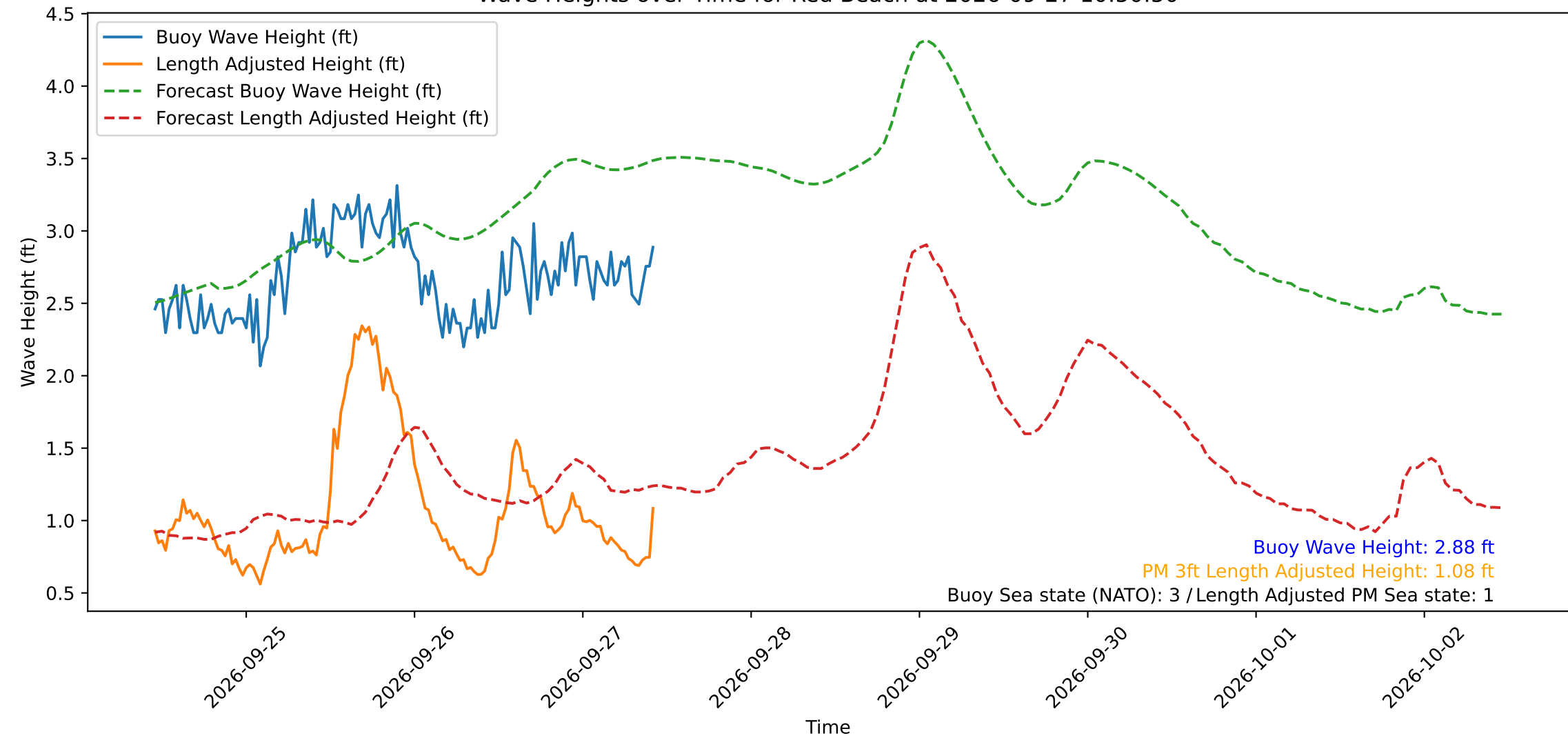
Wave Heights over Time for Red Beach at 2026-09-27 10:50:50
