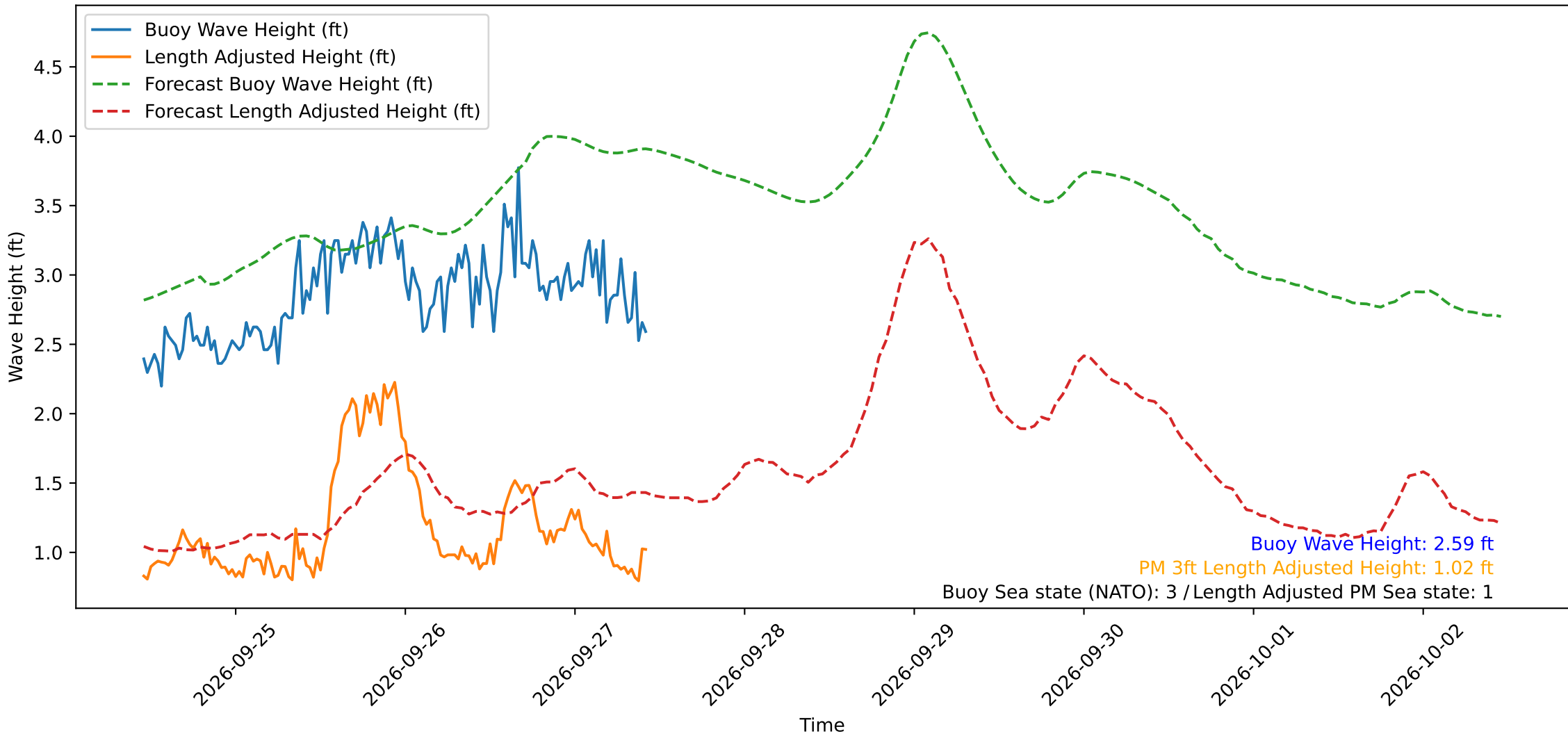
Wave Heights over Time for Oceanside Harbor at 2026-09-27 10:50:29
