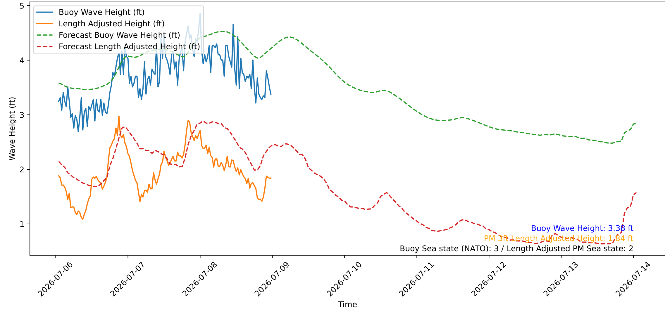
Wave Heights over Time for Red Beach at 2026-07-09 00:30:46
