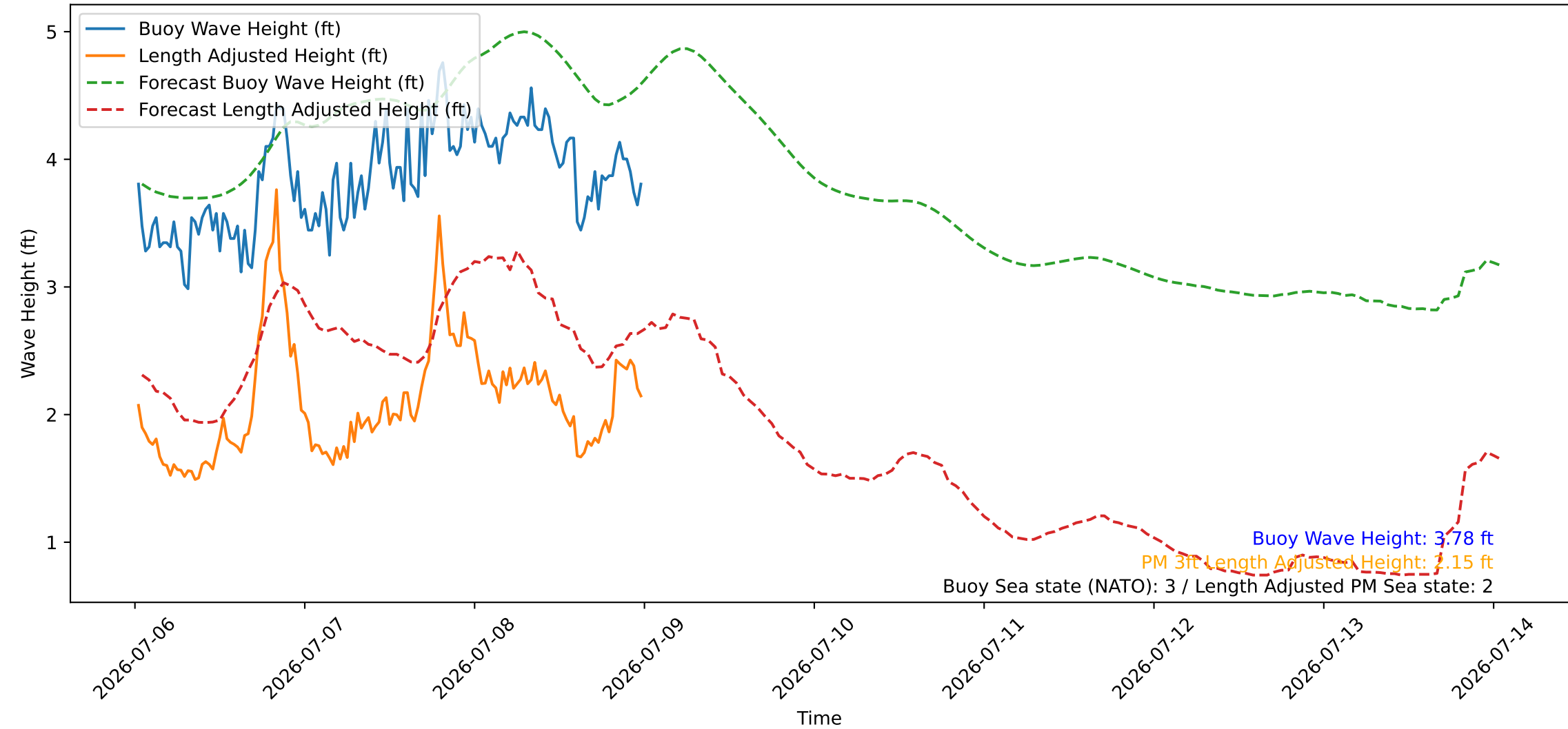
Wave Heights over Time for Green Beach at 2026-07-09 00:31:09
