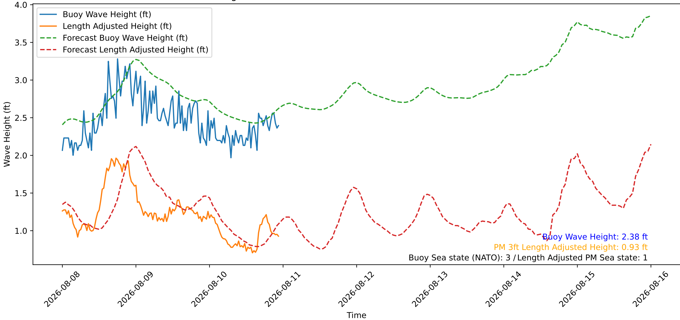
Wave Heights over Time for Oceanside Harbor at 2026-08-10 23:50:26
