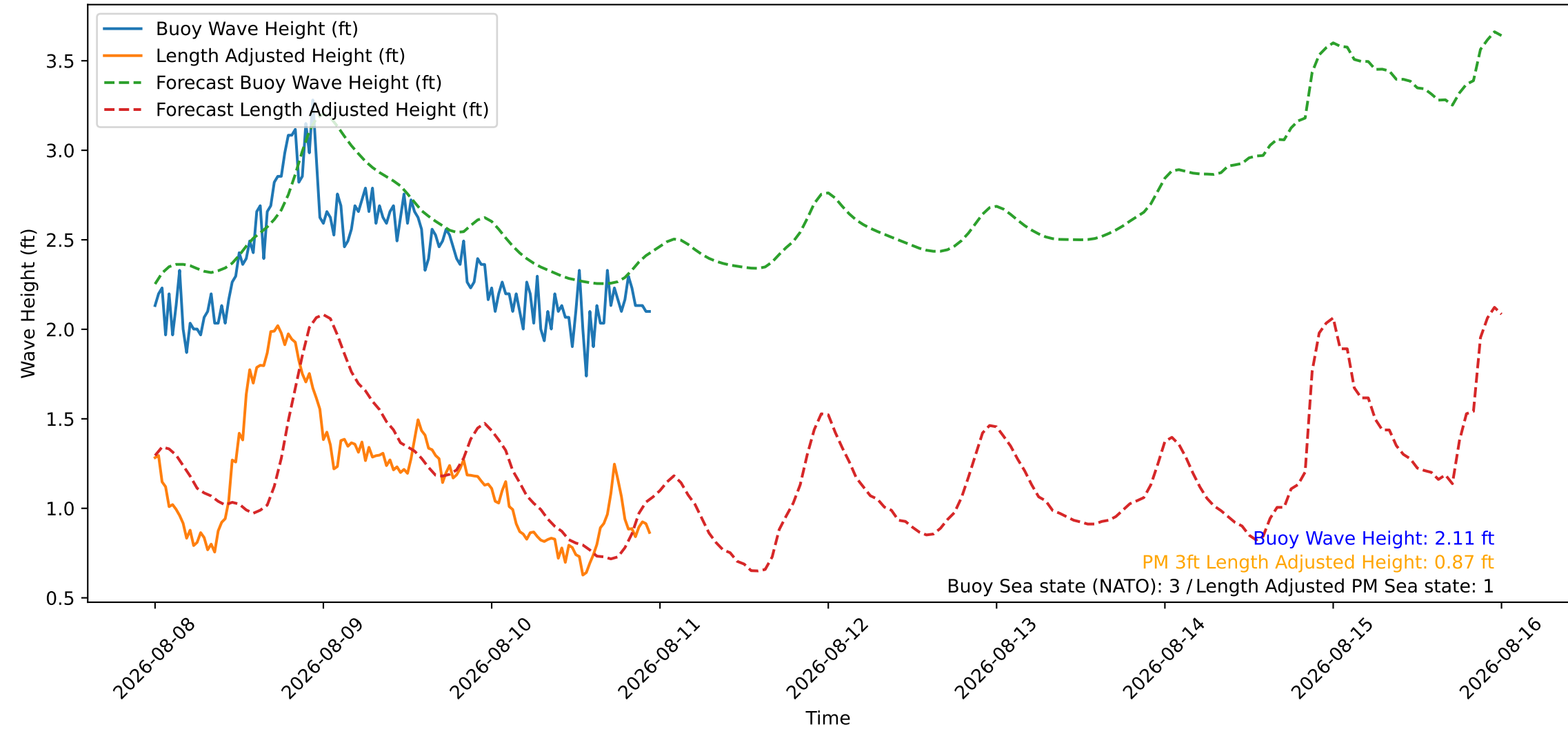
Wave Heights over Time for Red Beach at 2026-08-10 23:50:47
