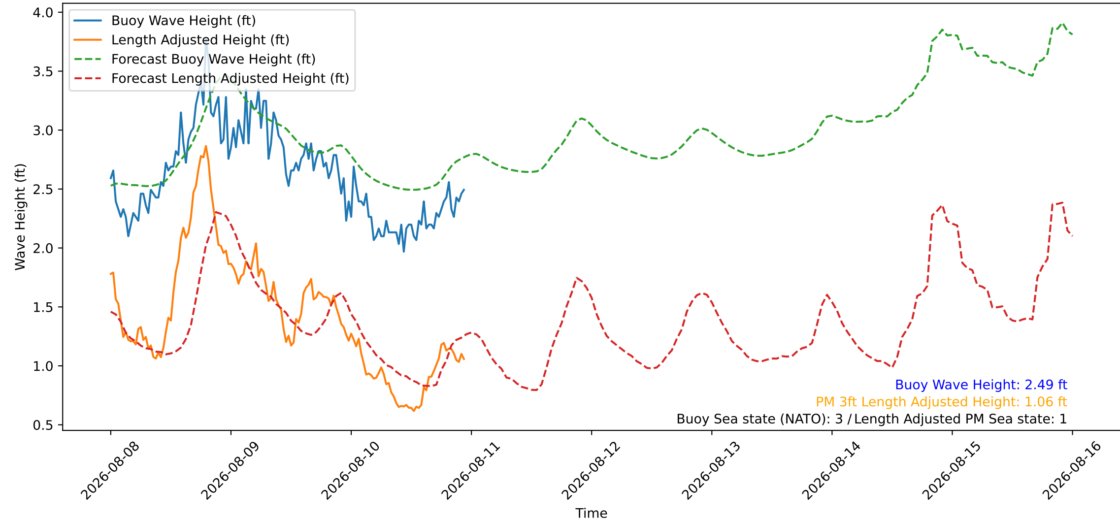
Wave Heights over Time for Green Beach at 2026-08-10 23:51:09
