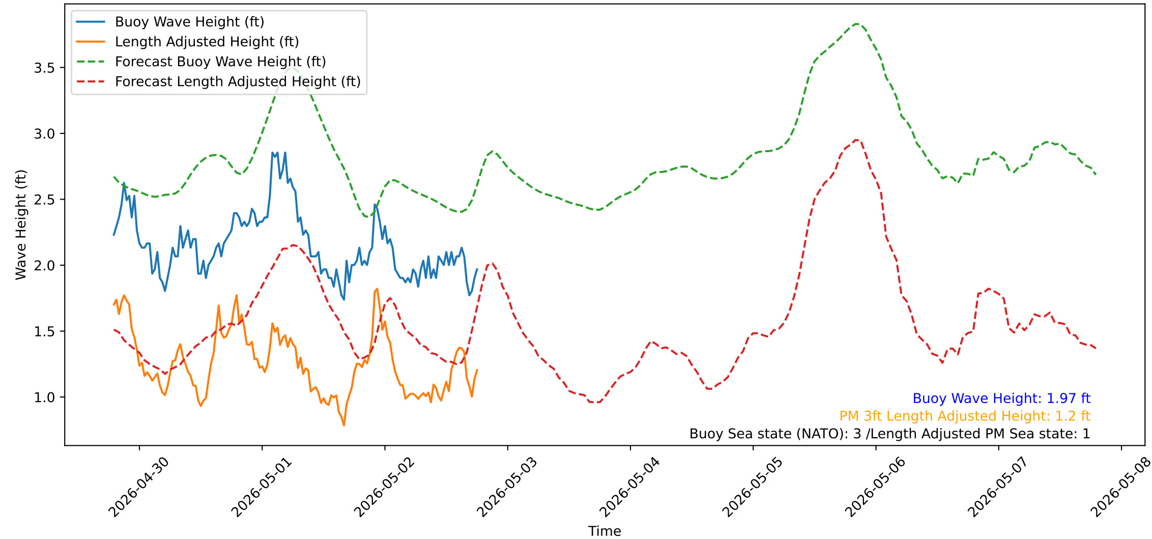
Wave Heights over Time for Green Beach at 2026-05-02 18:51:14
