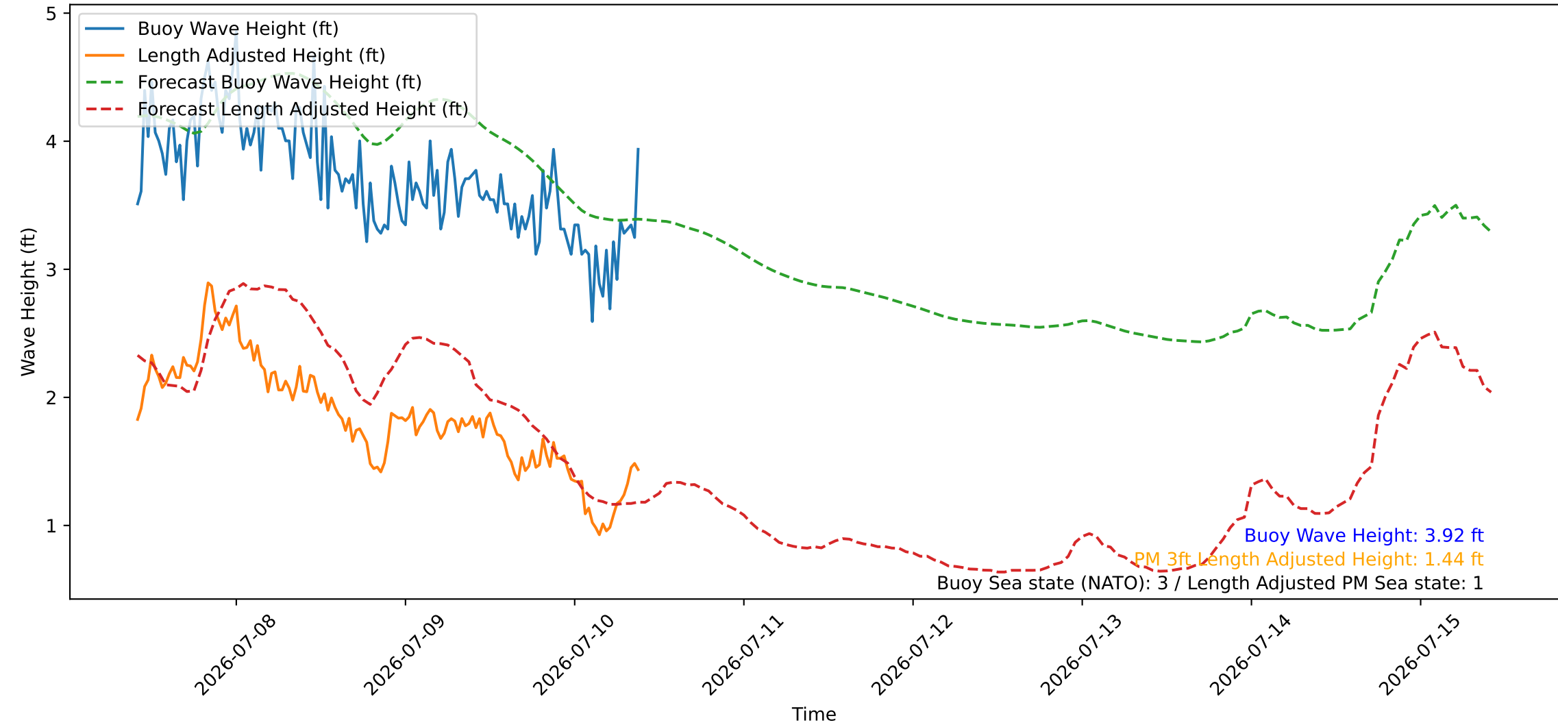
Wave Heights over Time for Red Beach at 2026-07-10 09:40:46
