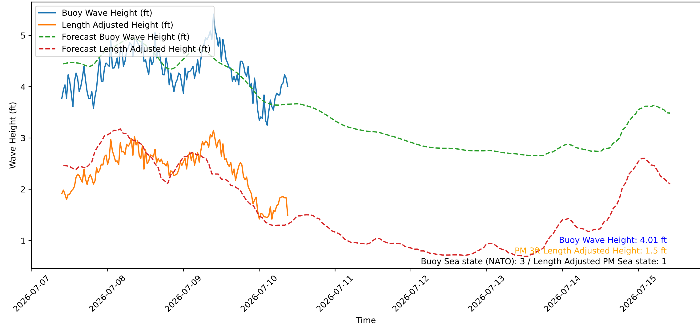
Wave Heights over Time for Oceanside Harbor at 2026-07-10 09:40:26
