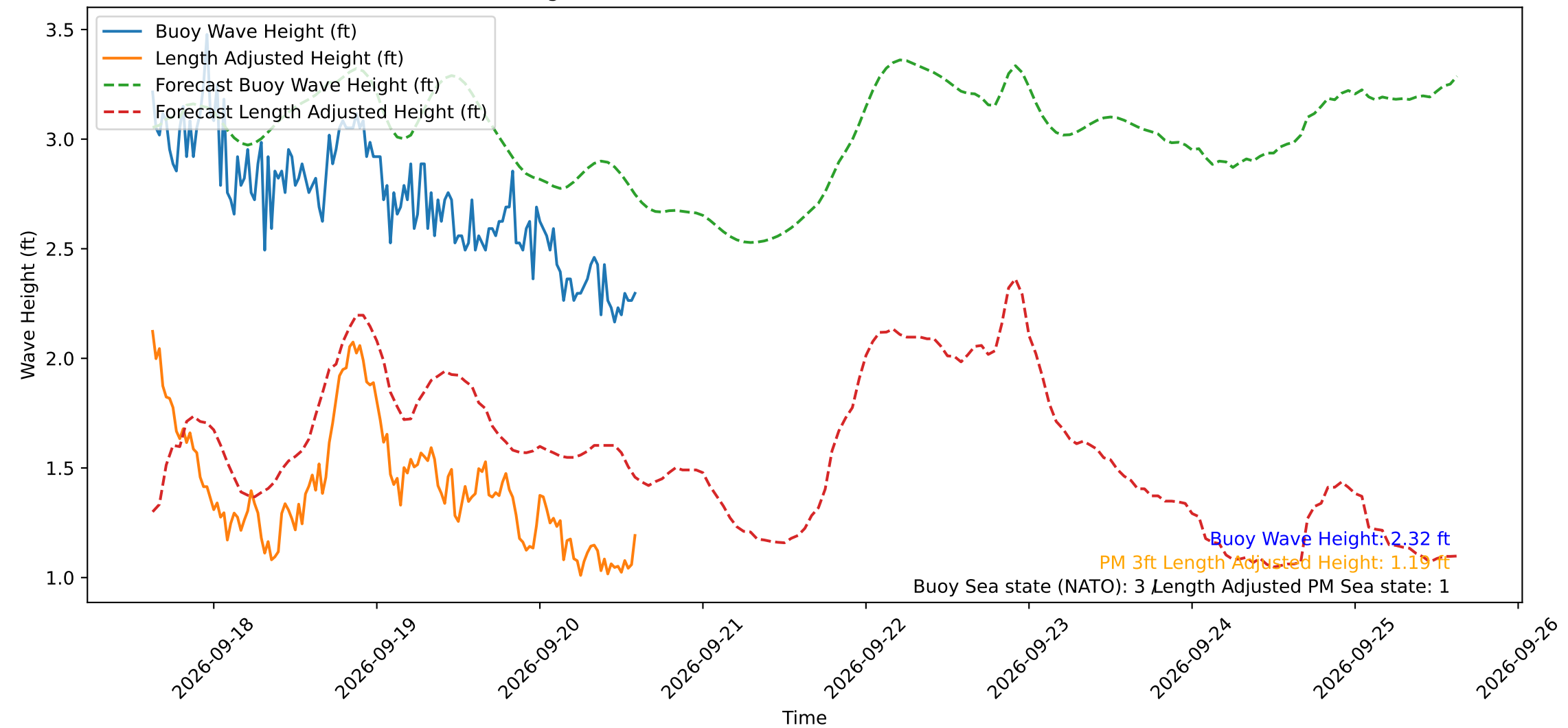
Wave Heights over Time for Green Beach at 2026-09-20 14:51:13
