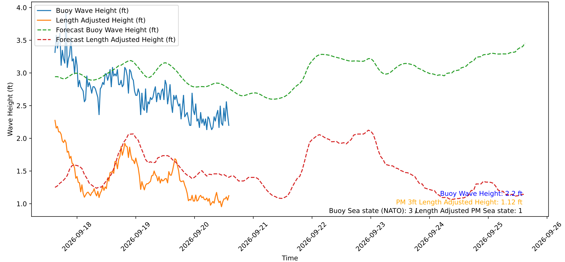
Wave Heights over Time for Oceanside Harbor at 2026-09-20 14:50:29
