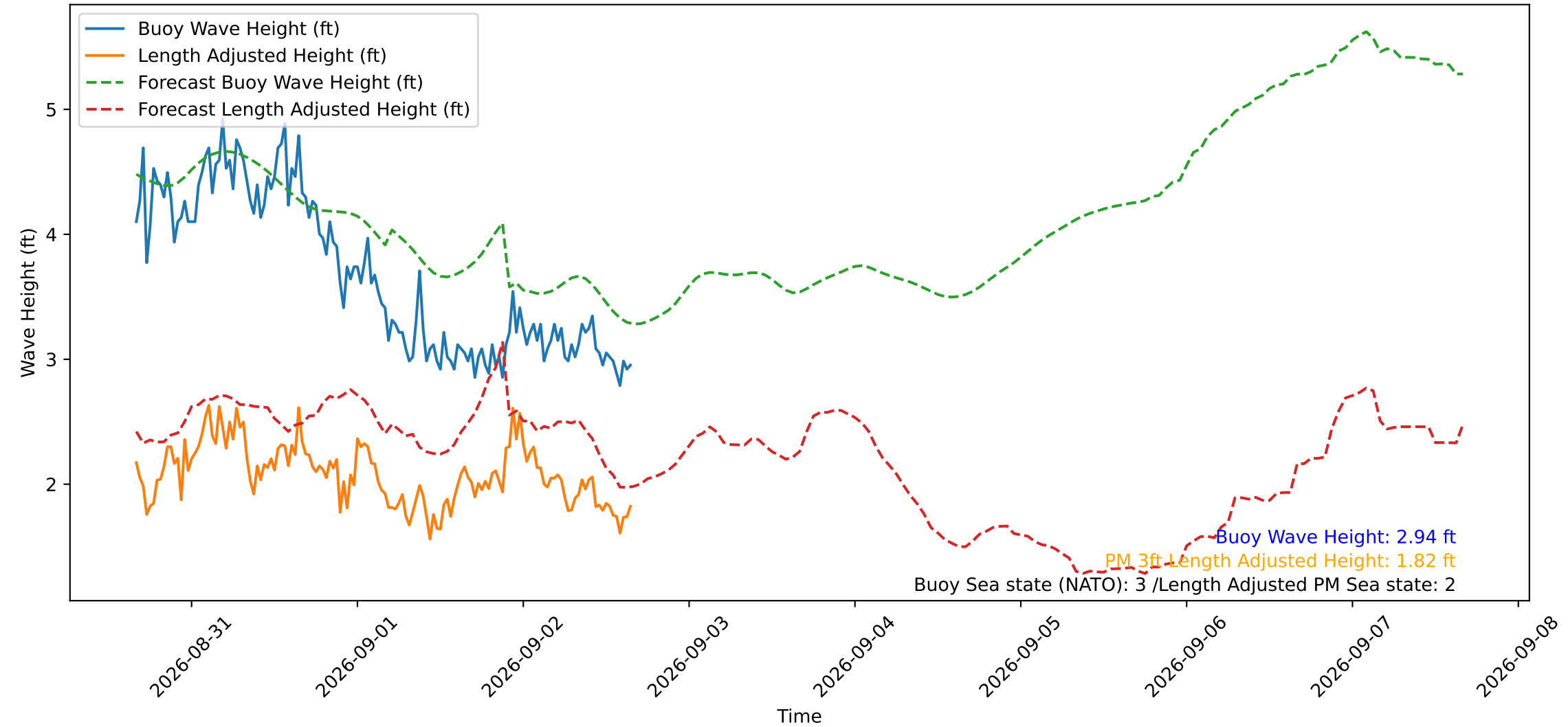
Wave Heights over Time for Oceanside Harbor at 2026-09-02 16:10:29
