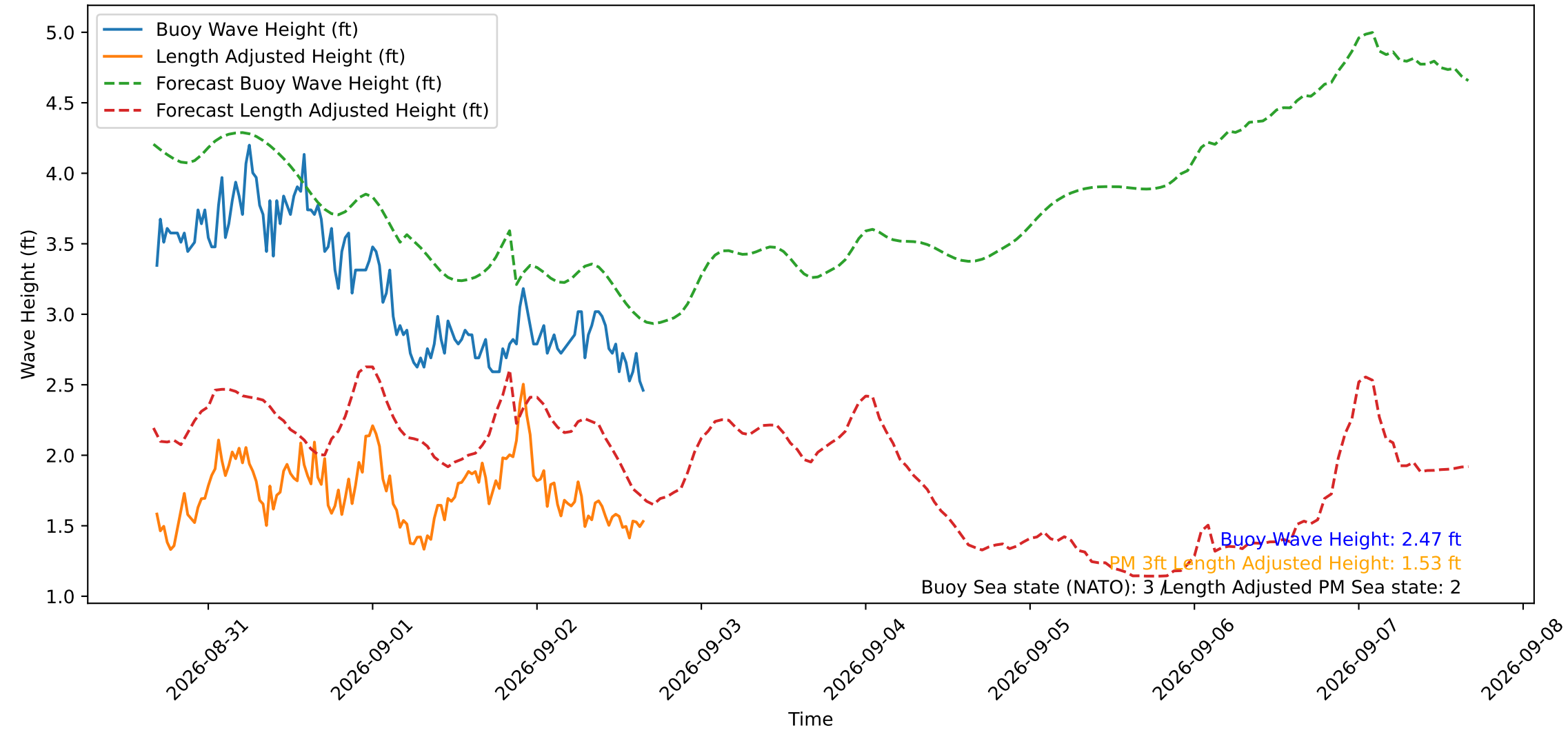
Wave Heights over Time for Red Beach at 2026-09-02 16:10:49
