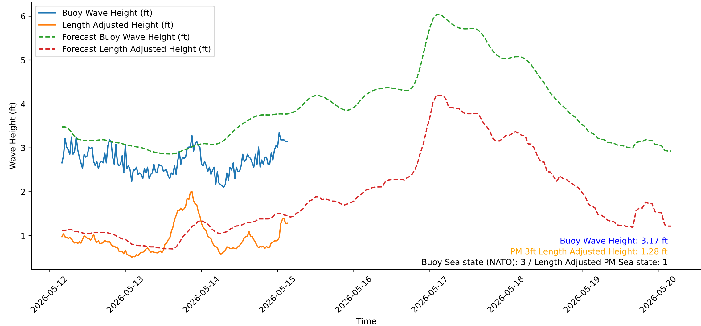
Wave Heights over Time for Green Beach at 2026-05-15 03:51:15
