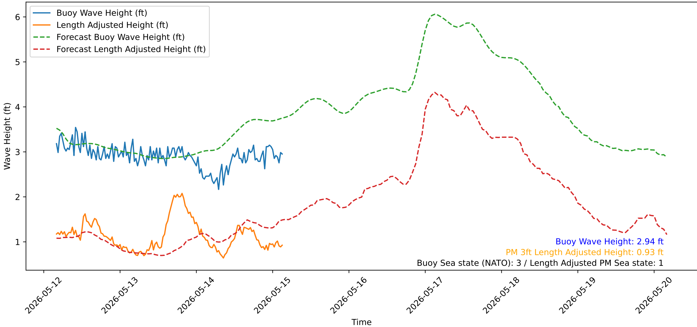
Wave Heights over Time for Oceanside Harbor at 2026-05-15 03:50:31
