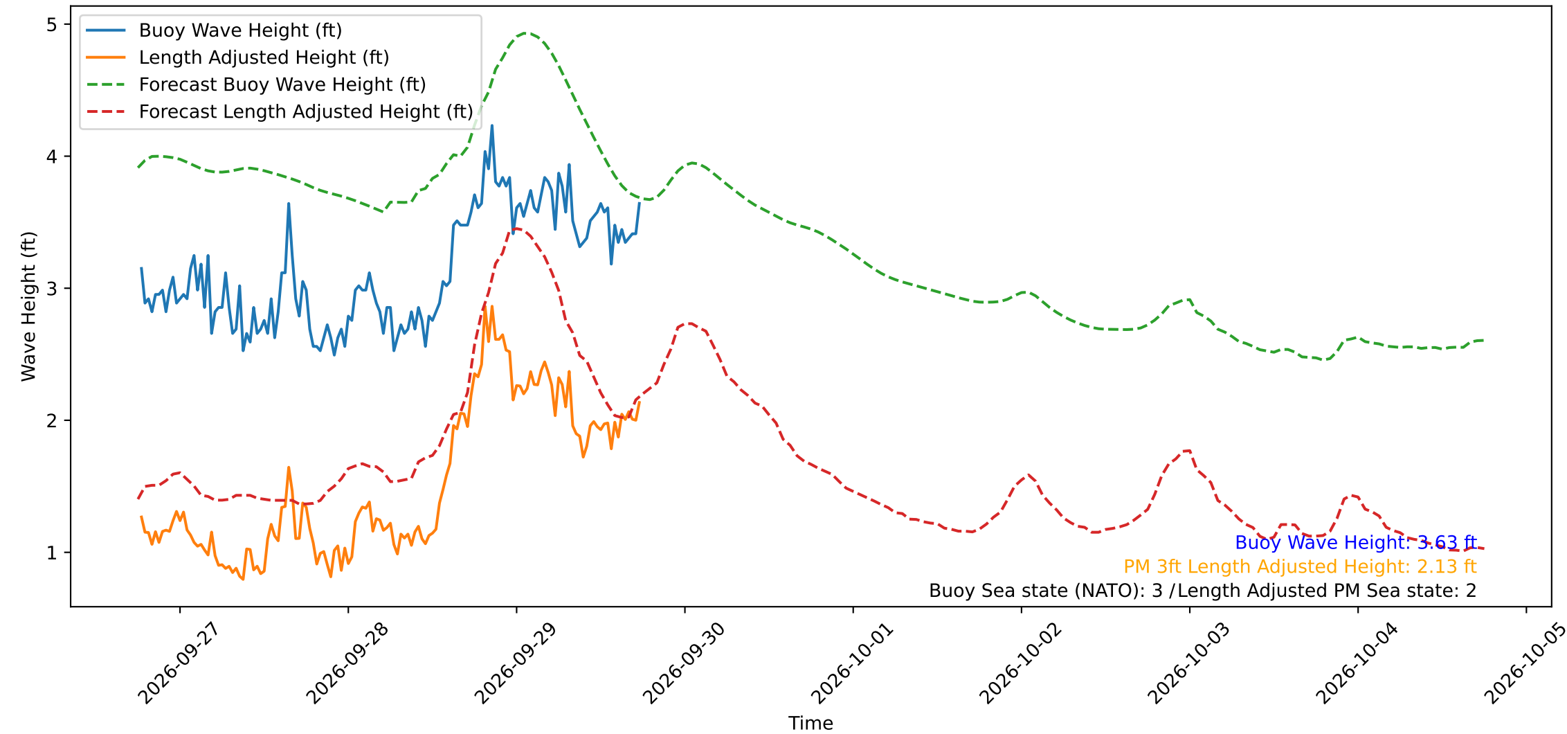
Wave Heights over Time for Oceanside Harbor at 2026-09-29 18:20:29
