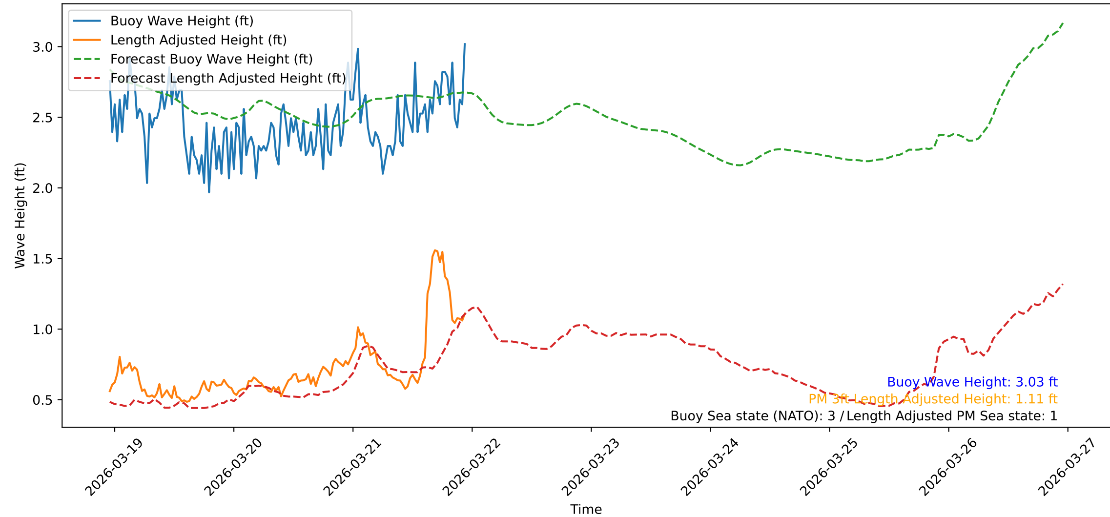
Wave Heights over Time for Oceanside Harbor at 2026-03-21 23:00:31
