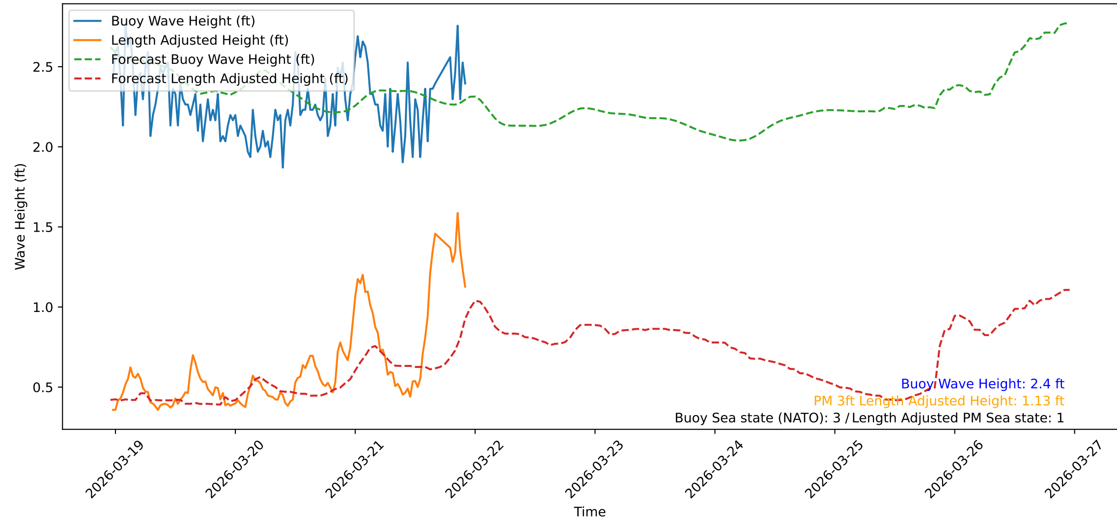
Wave Heights over Time for Red Beach at 2026-03-21 23:00:47
