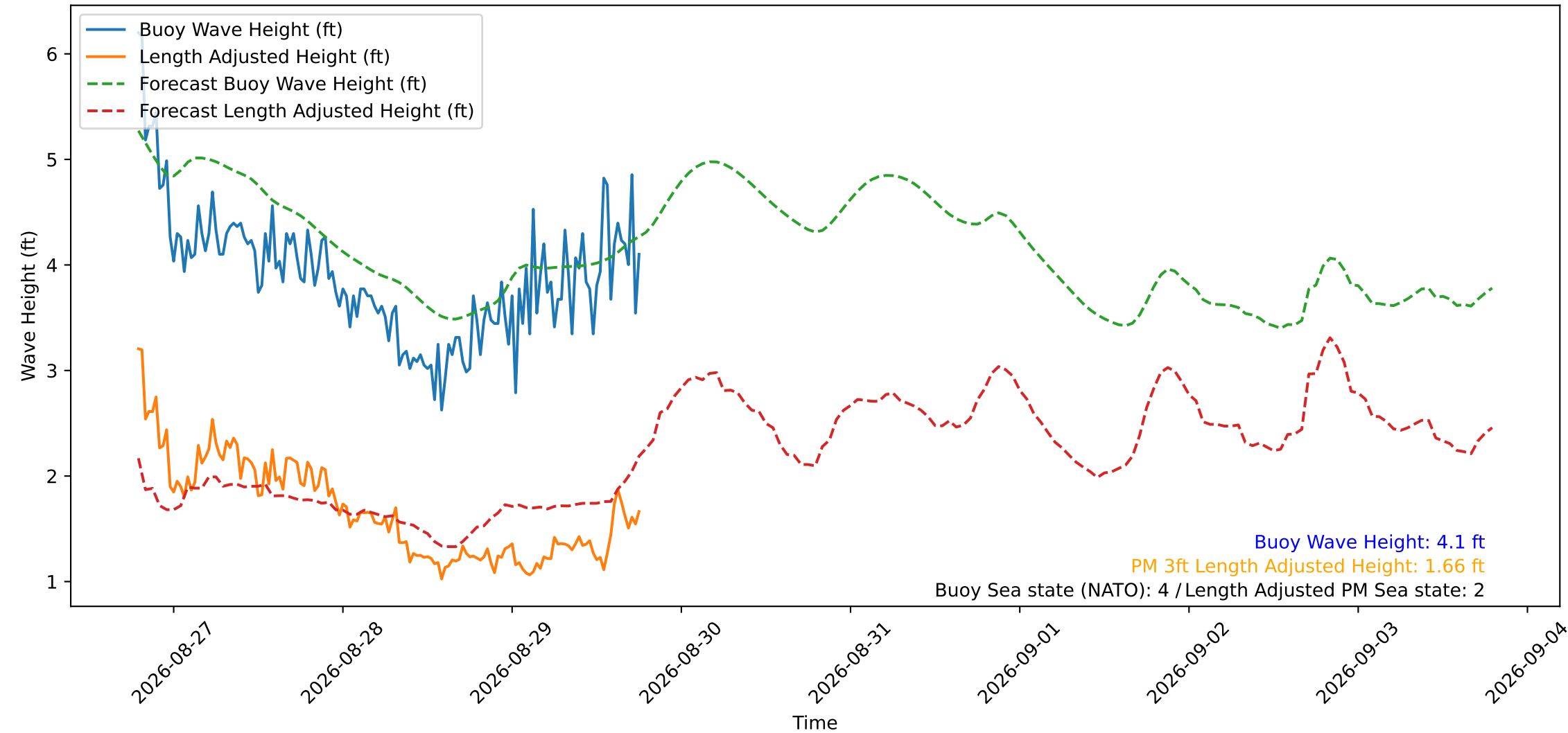
Wave Heights over Time for Green Beach at 2026-08-29 18:51:15
