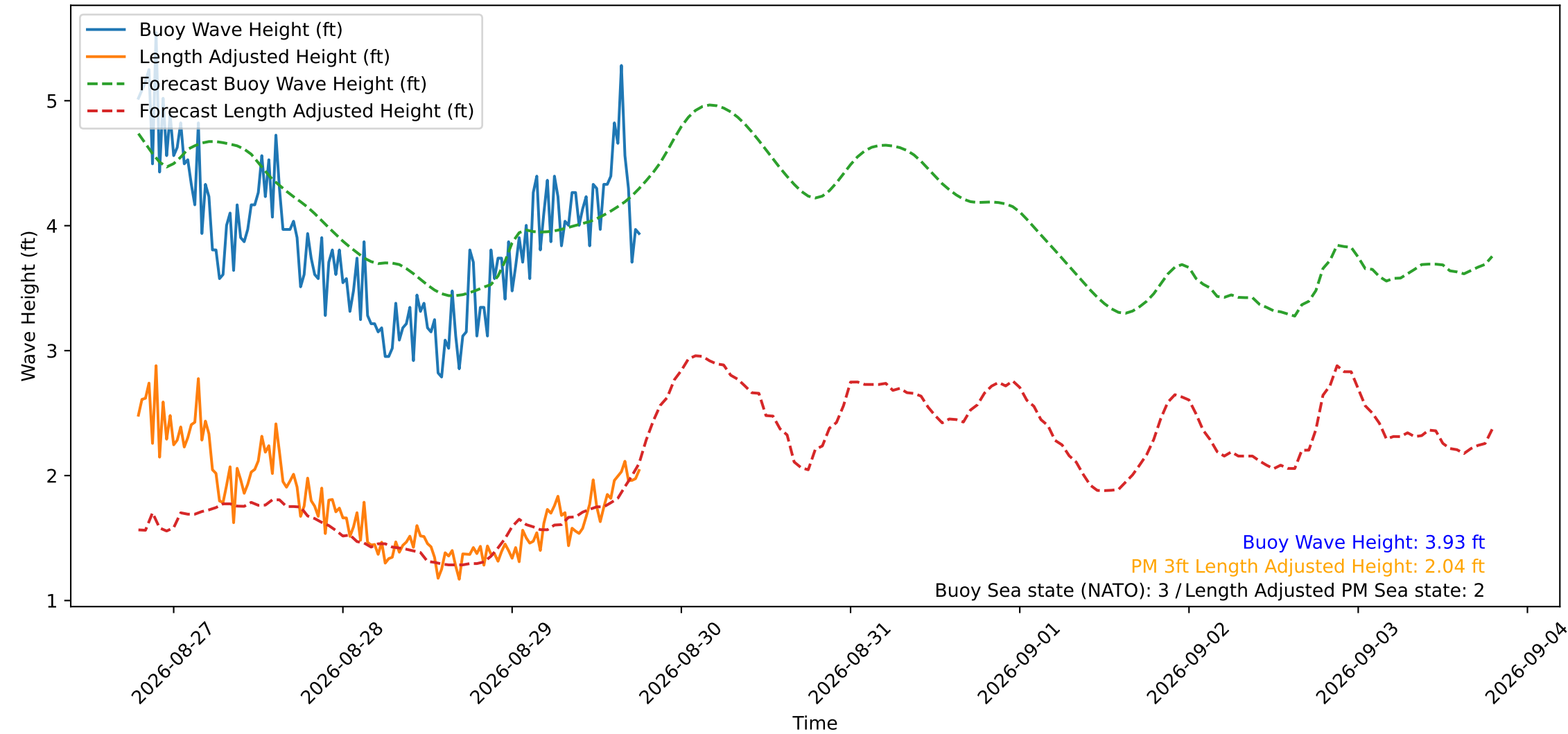
Wave Heights over Time for Oceanside Harbor at 2026-08-29 18:50:29
