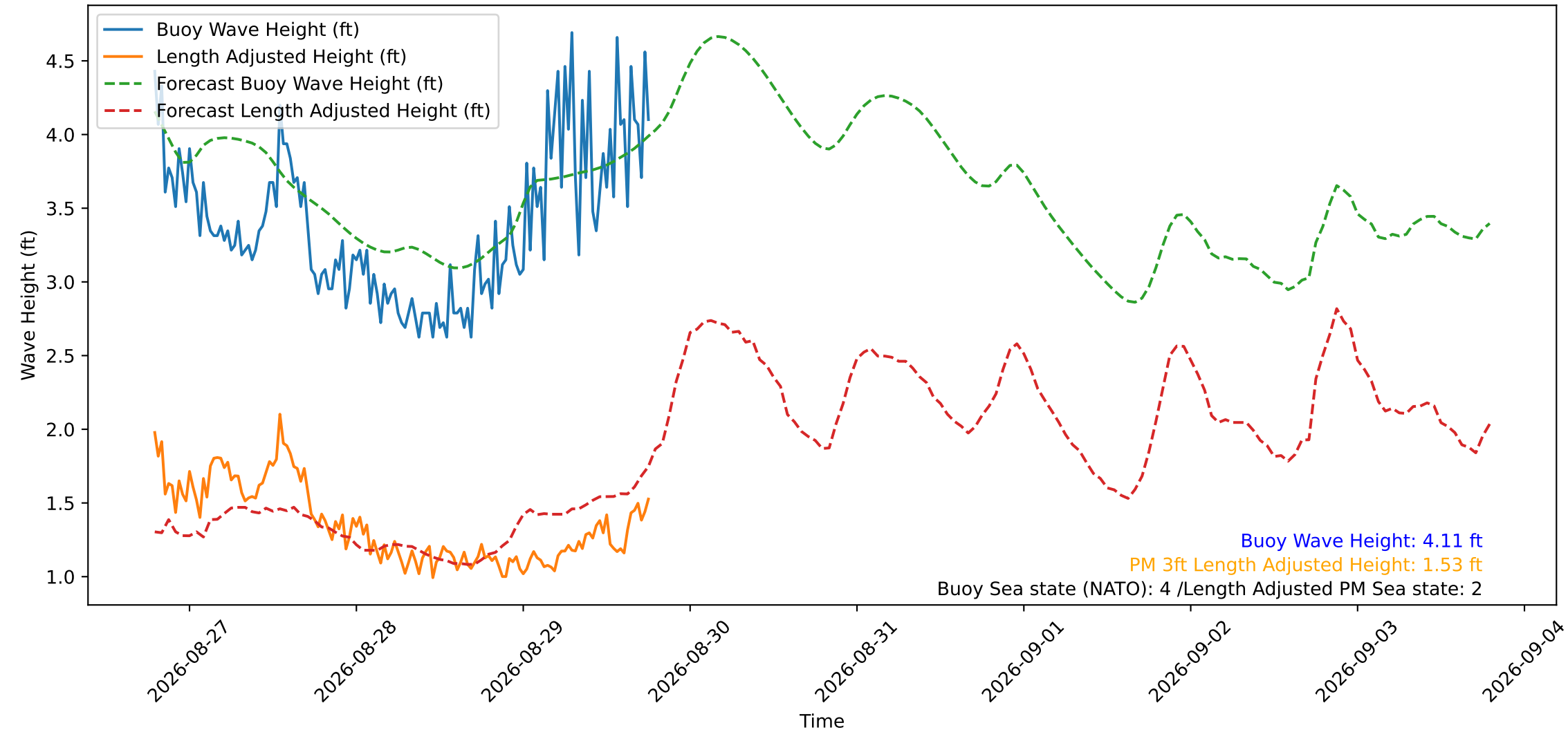
Wave Heights over Time for Red Beach at 2026-08-29 18:50:51
