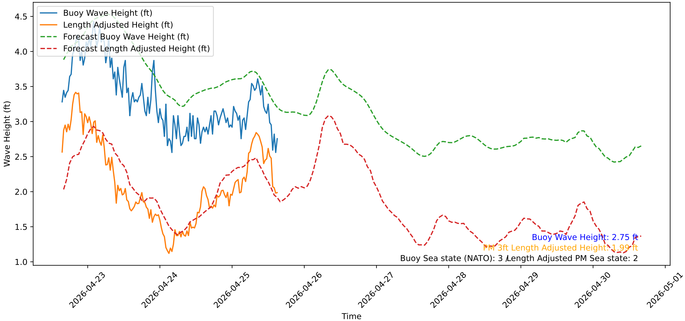
Wave Heights over Time for Oceanside Harbor at 2026-04-25 15:40:32
