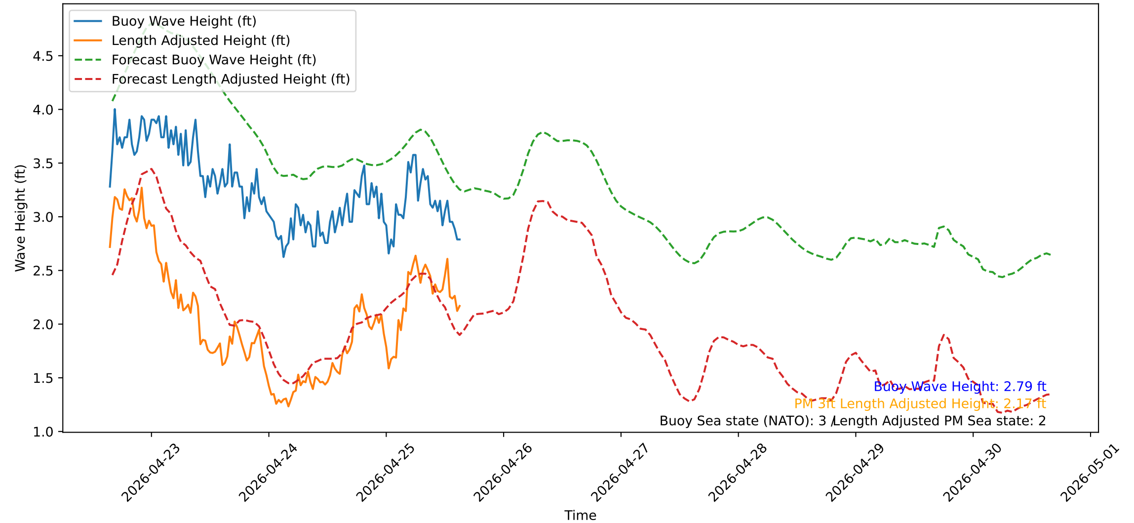
Wave Heights over Time for Green Beach at 2026-04-25 15:41:13
