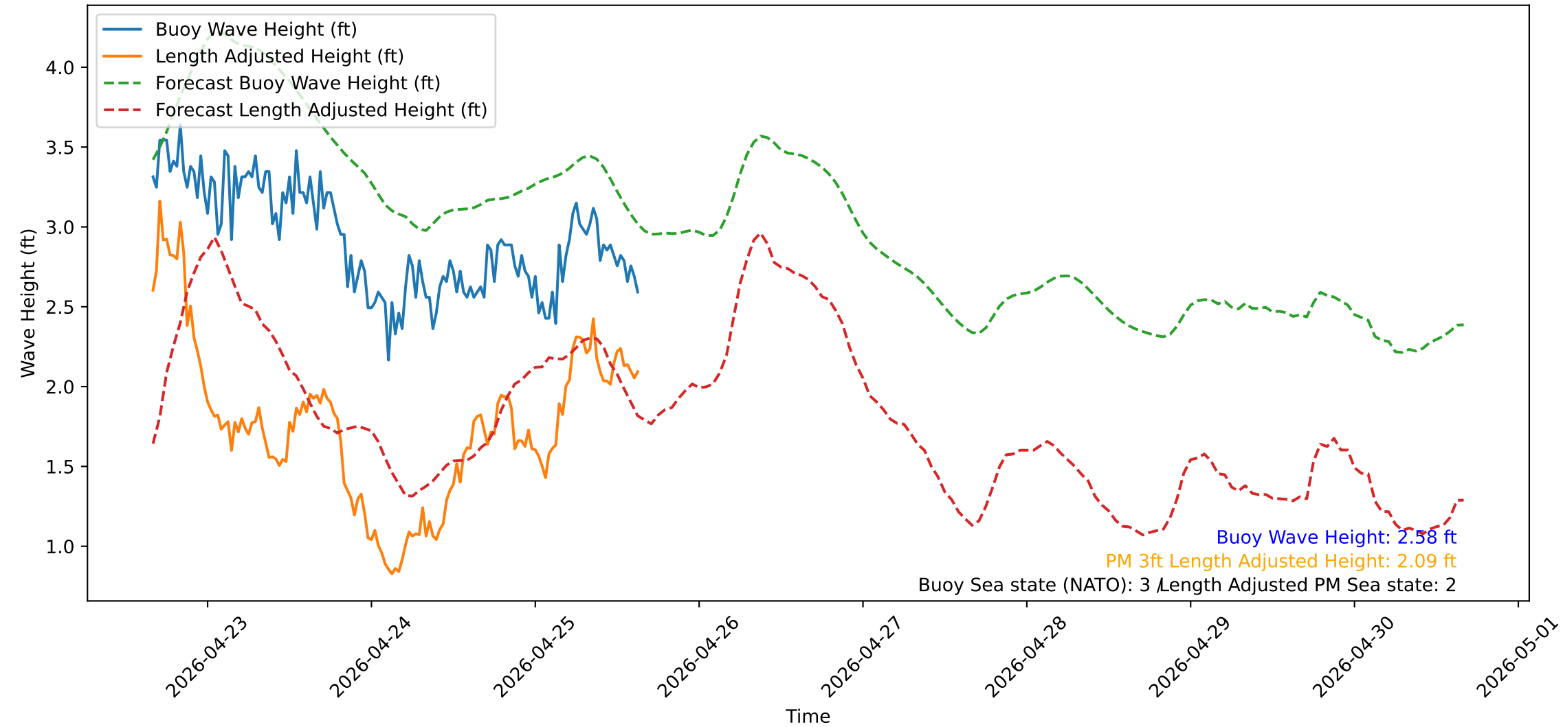
Wave Heights over Time for Red Beach at 2026-04-25 15:40:51
