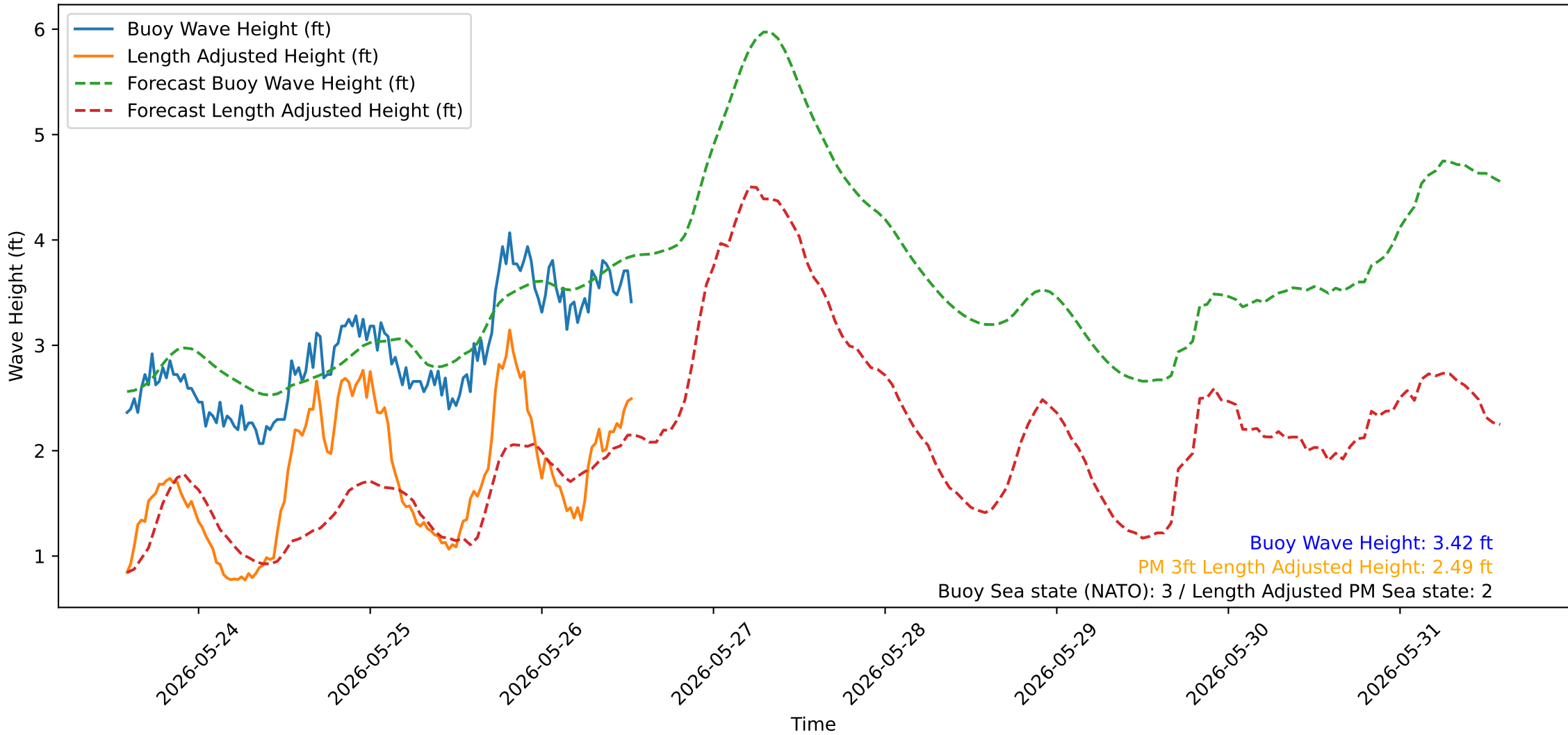
Wave Heights over Time for Green Beach at 2026-05-26 13:51:11
