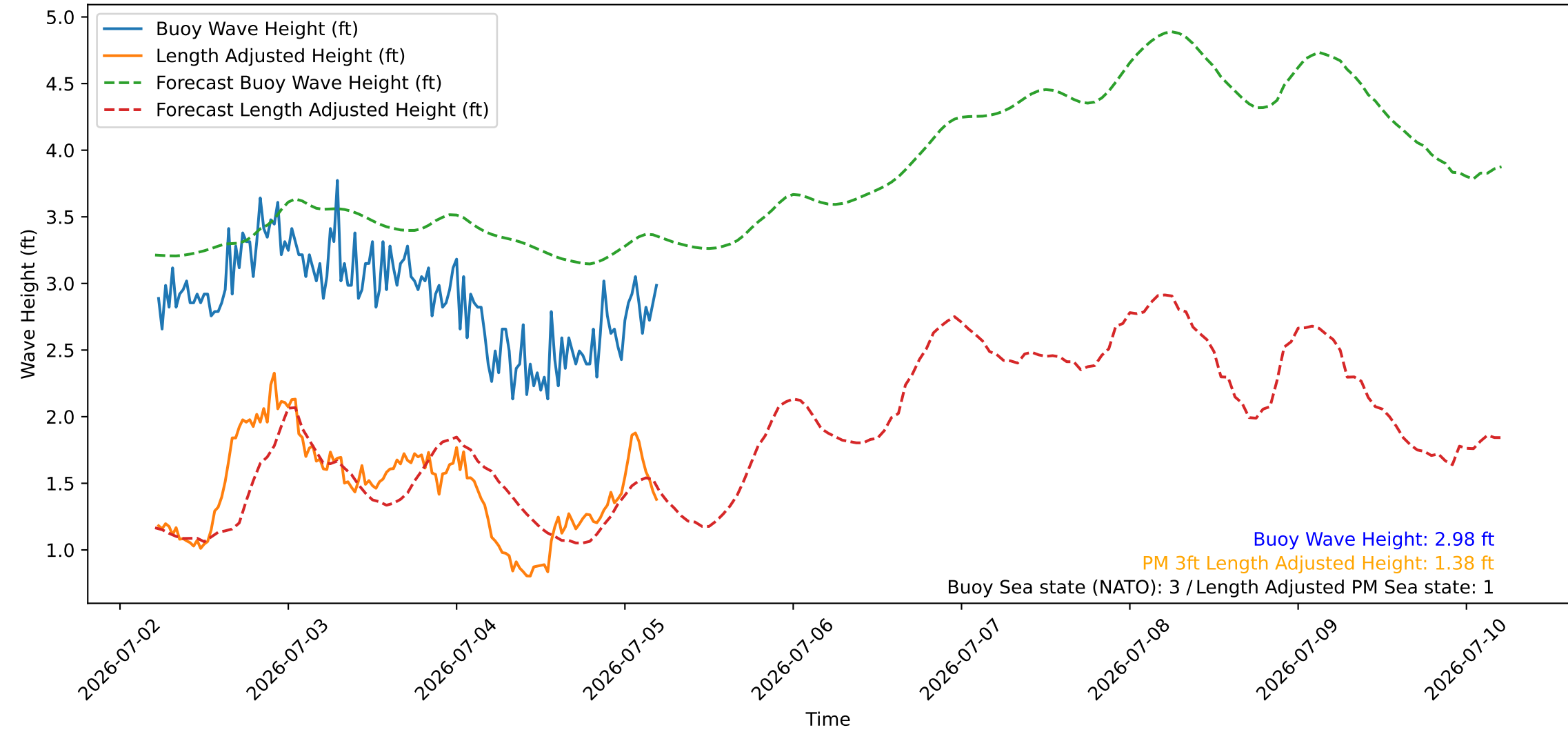
Wave Heights over Time for Oceanside Harbor at 2026-07-05 05:20:26
