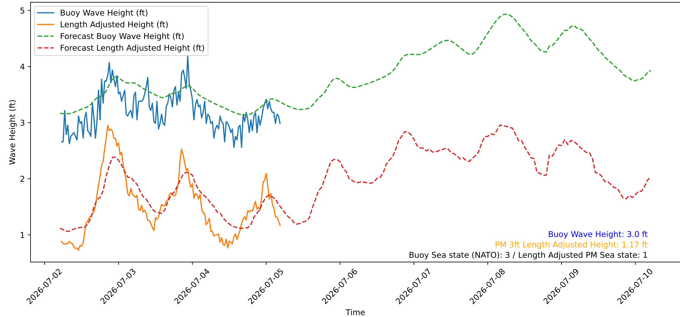
Wave Heights over Time for Green Beach at 2026-07-05 05:21:10
