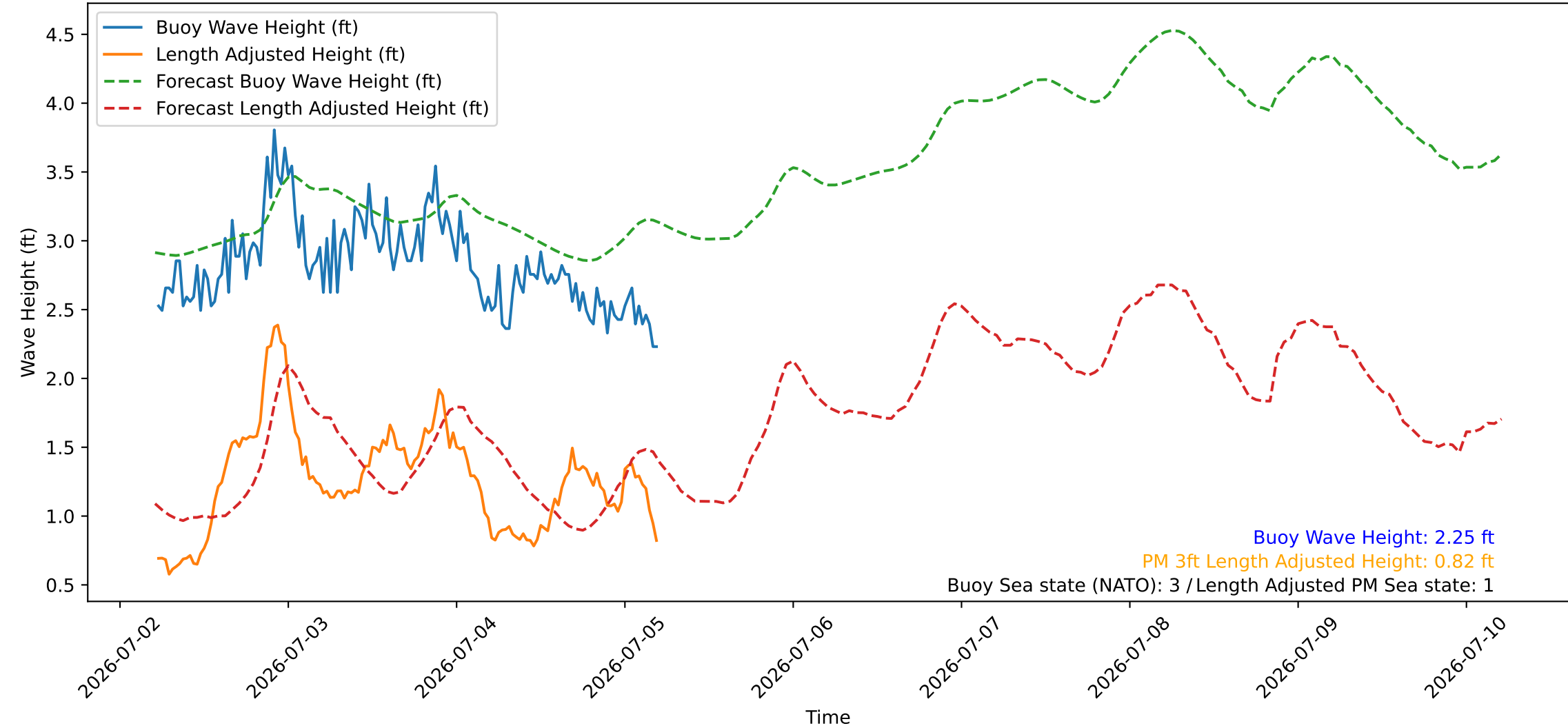
Wave Heights over Time for Red Beach at 2026-07-05 05:20:47
