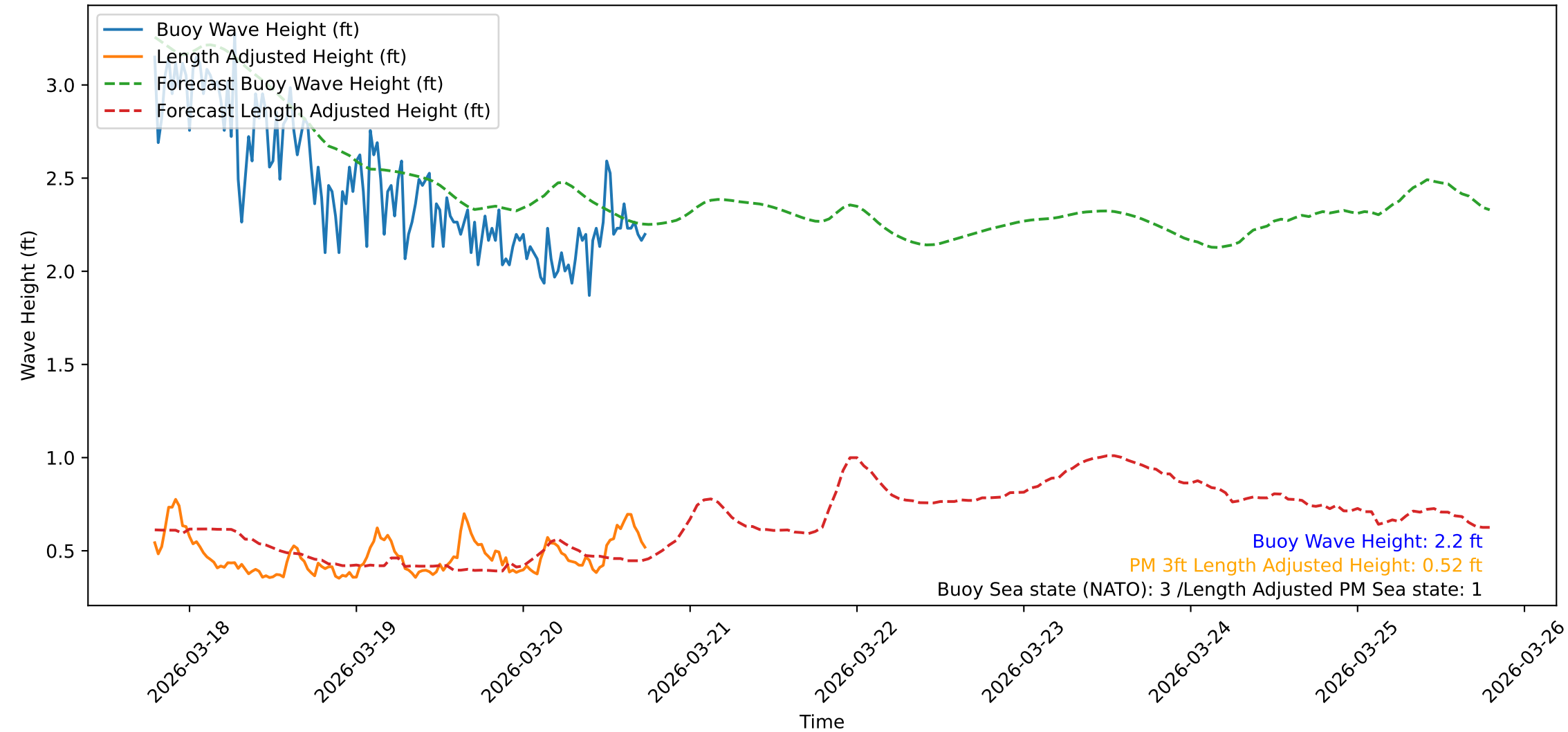
Wave Heights over Time for Red Beach at 2026-03-20 18:40:47
