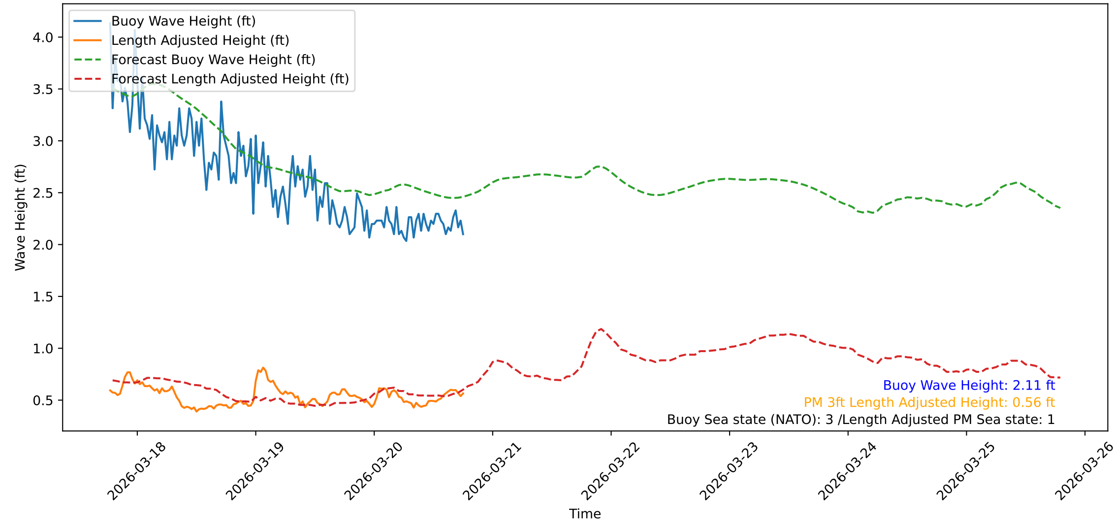
Wave Heights over Time for Green Beach at 2026-03-20 18:41:10
