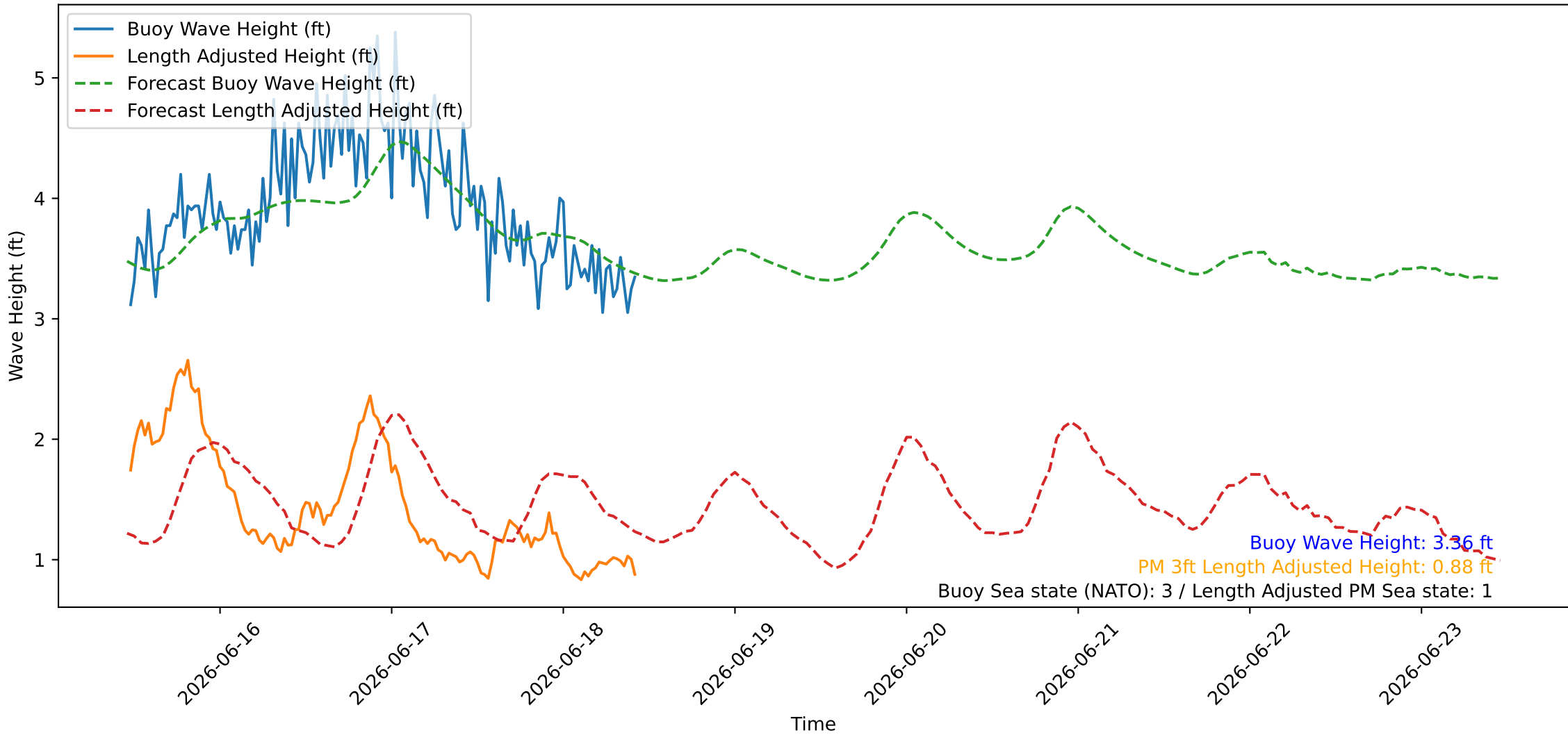
Wave Heights over Time for Red Beach at 2026-06-18 11:00:45
