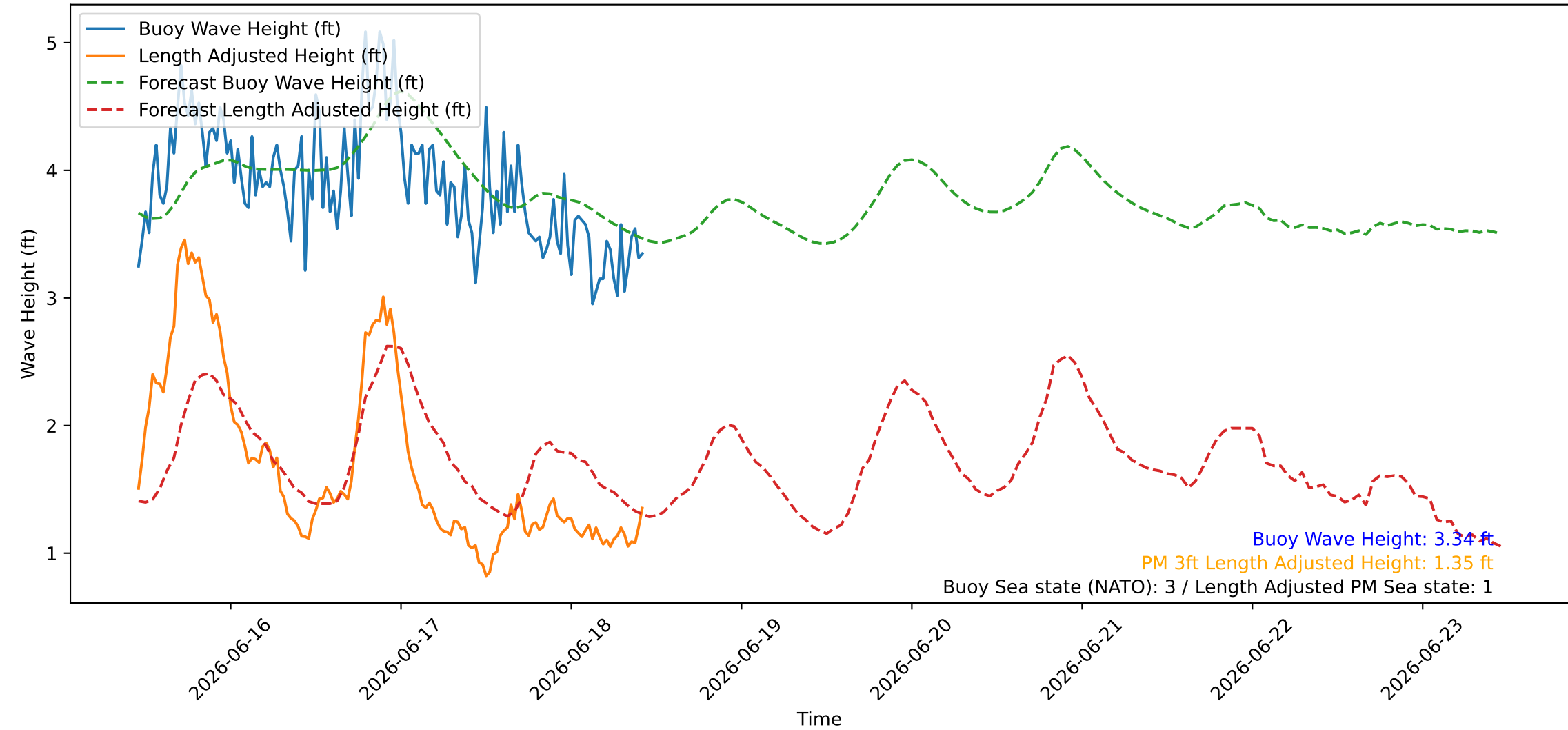
Wave Heights over Time for Green Beach at 2026-06-18 11:01:08
