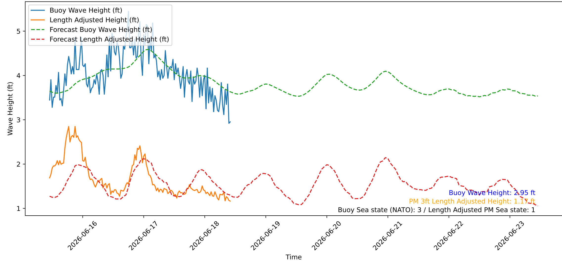
Wave Heights over Time for Oceanside Harbor at 2026-06-18 11:00:26
