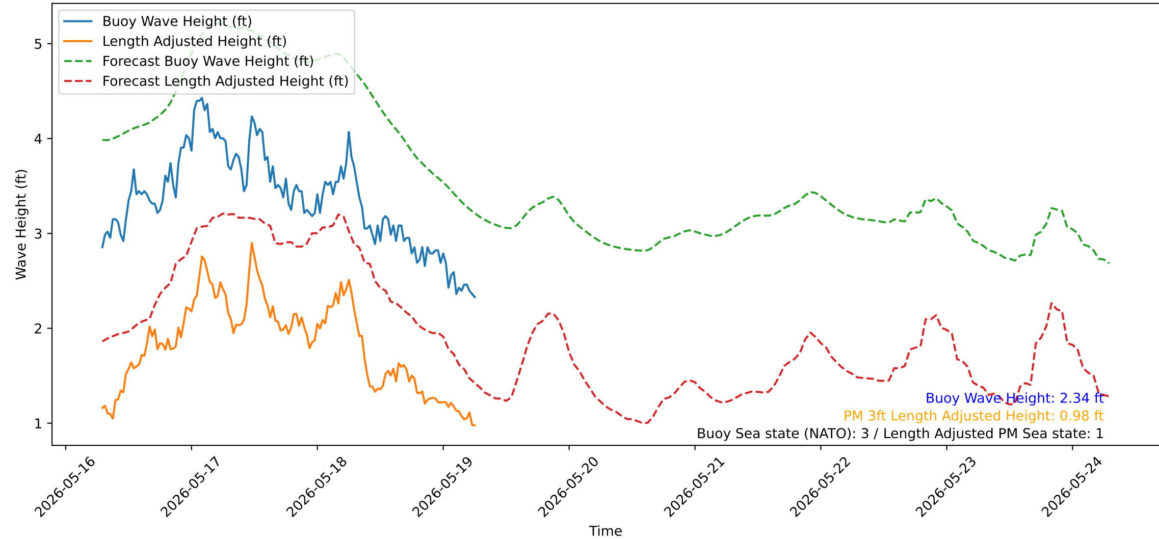
Wave Heights over Time for Green Beach at 2026-05-19 06:51:15
