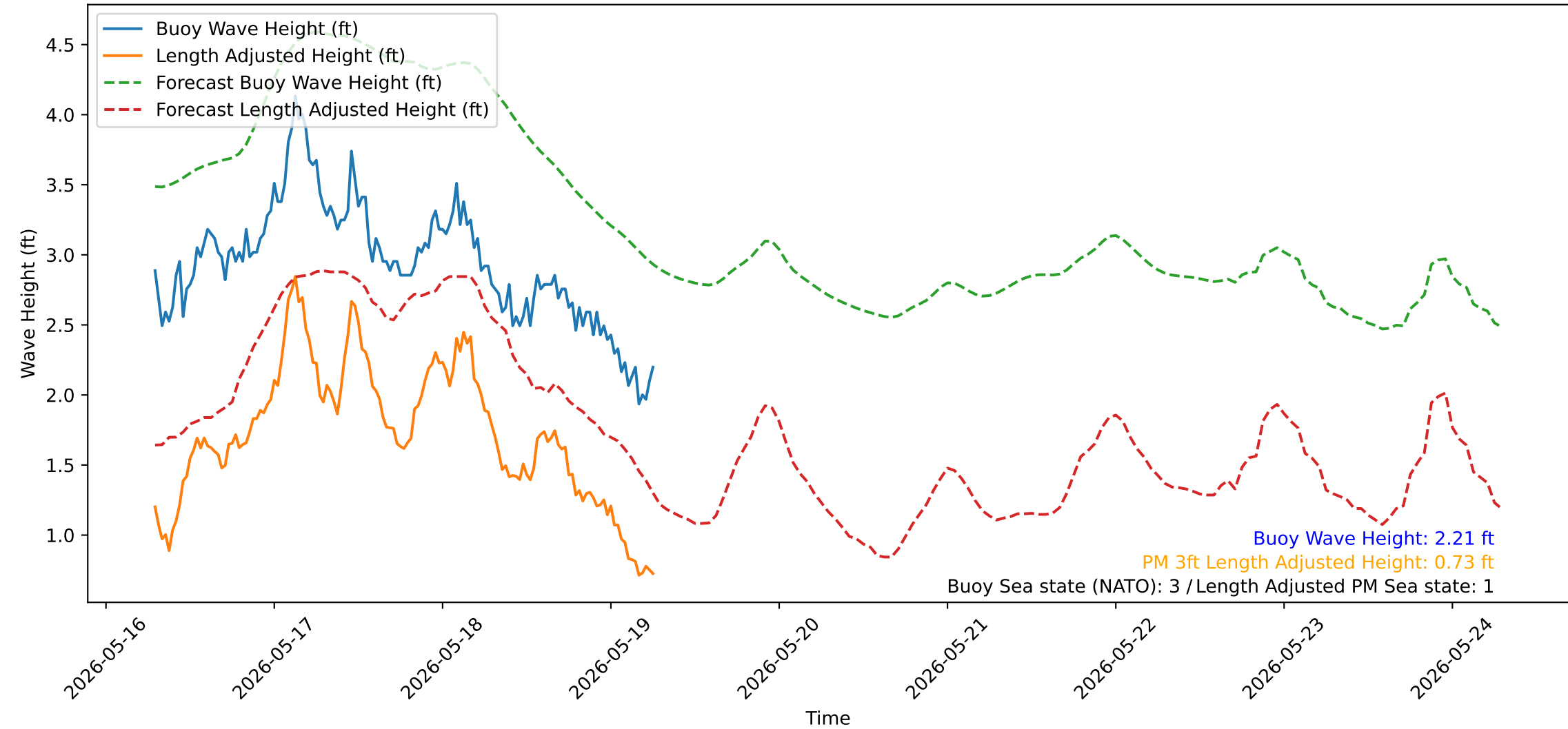
Wave Heights over Time for Red Beach at 2026-05-19 06:50:52
