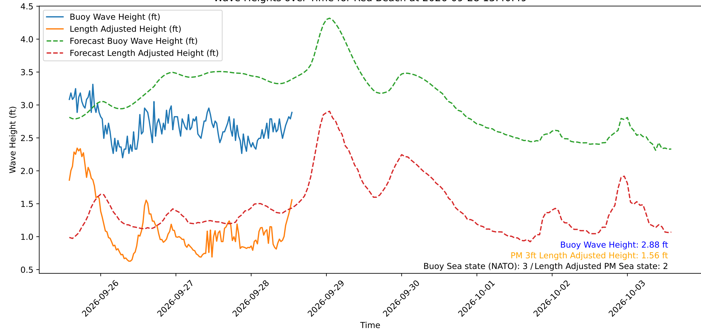
Wave Heights over Time for Red Beach at 2026-09-28 13:40:49
