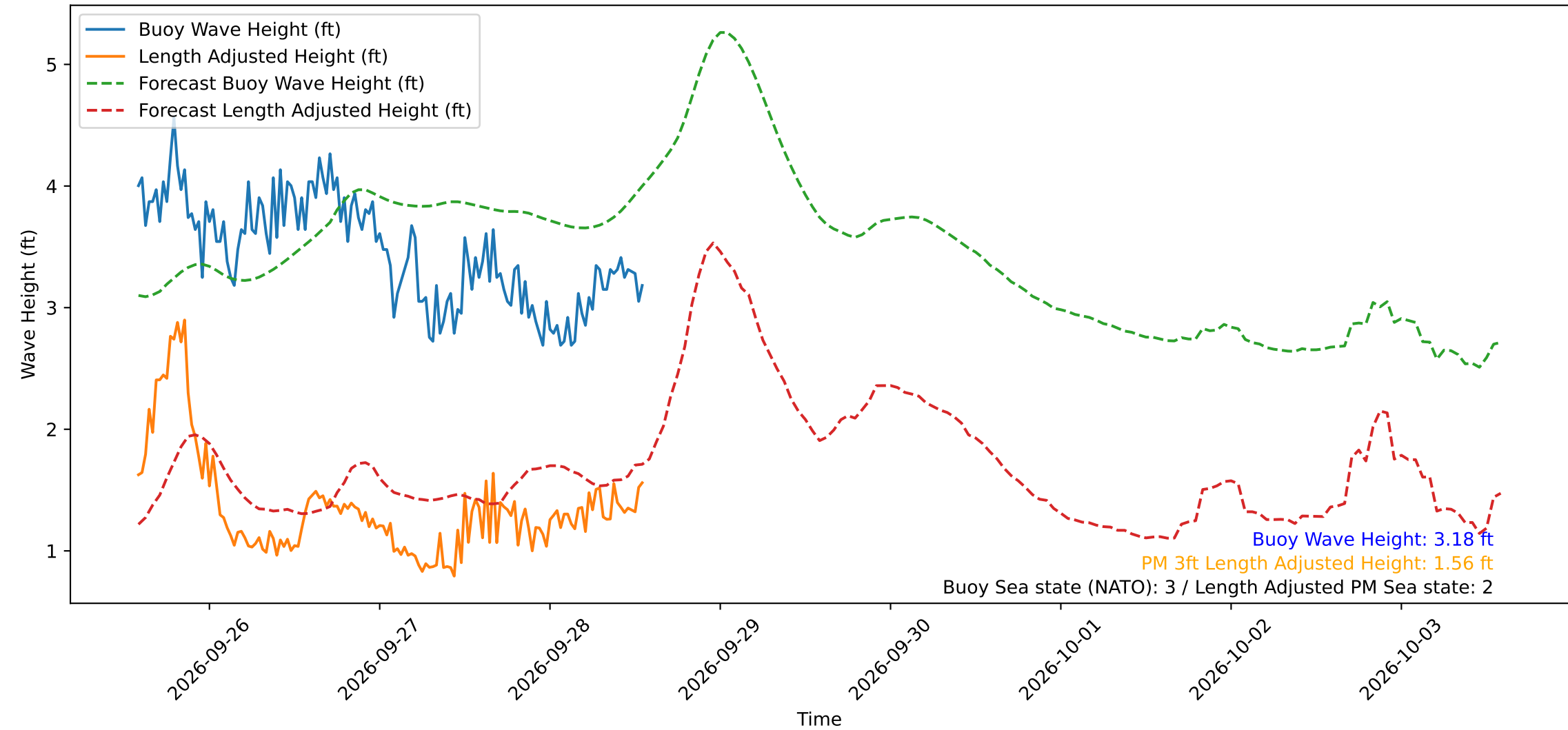
Wave Heights over Time for Green Beach at 2026-09-28 13:41:12
