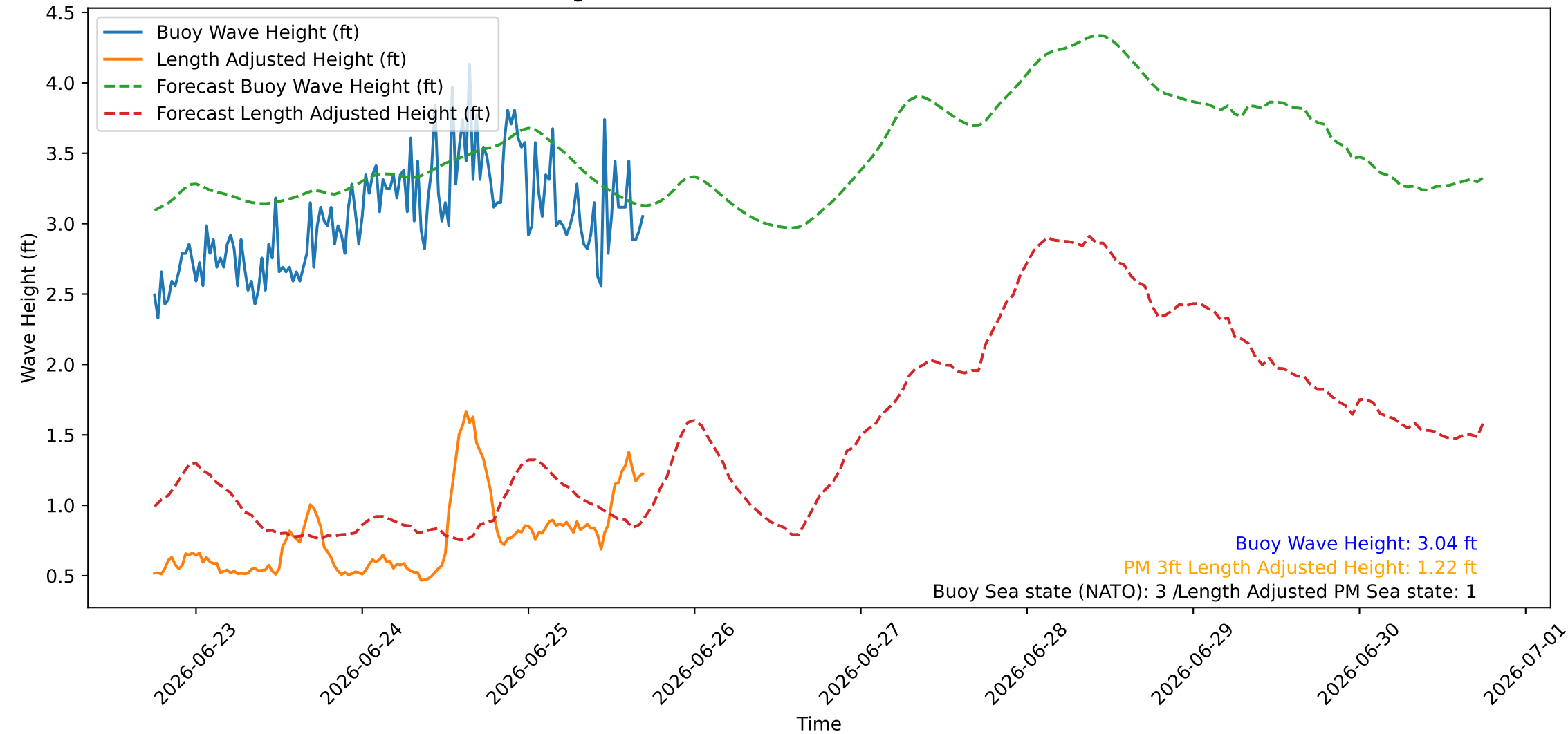
Wave Heights over Time for Red Beach at 2026-06-25 17:40:44
