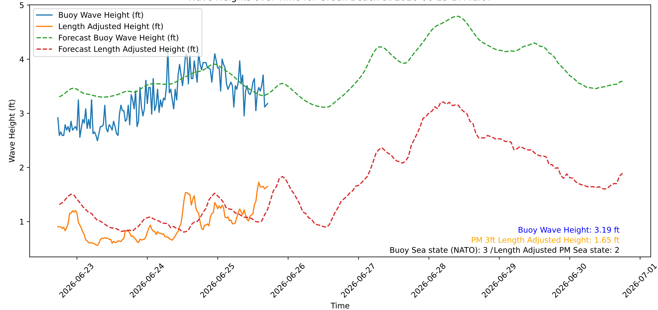
Wave Heights over Time for Green Beach at 2026-06-25 17:41:07
