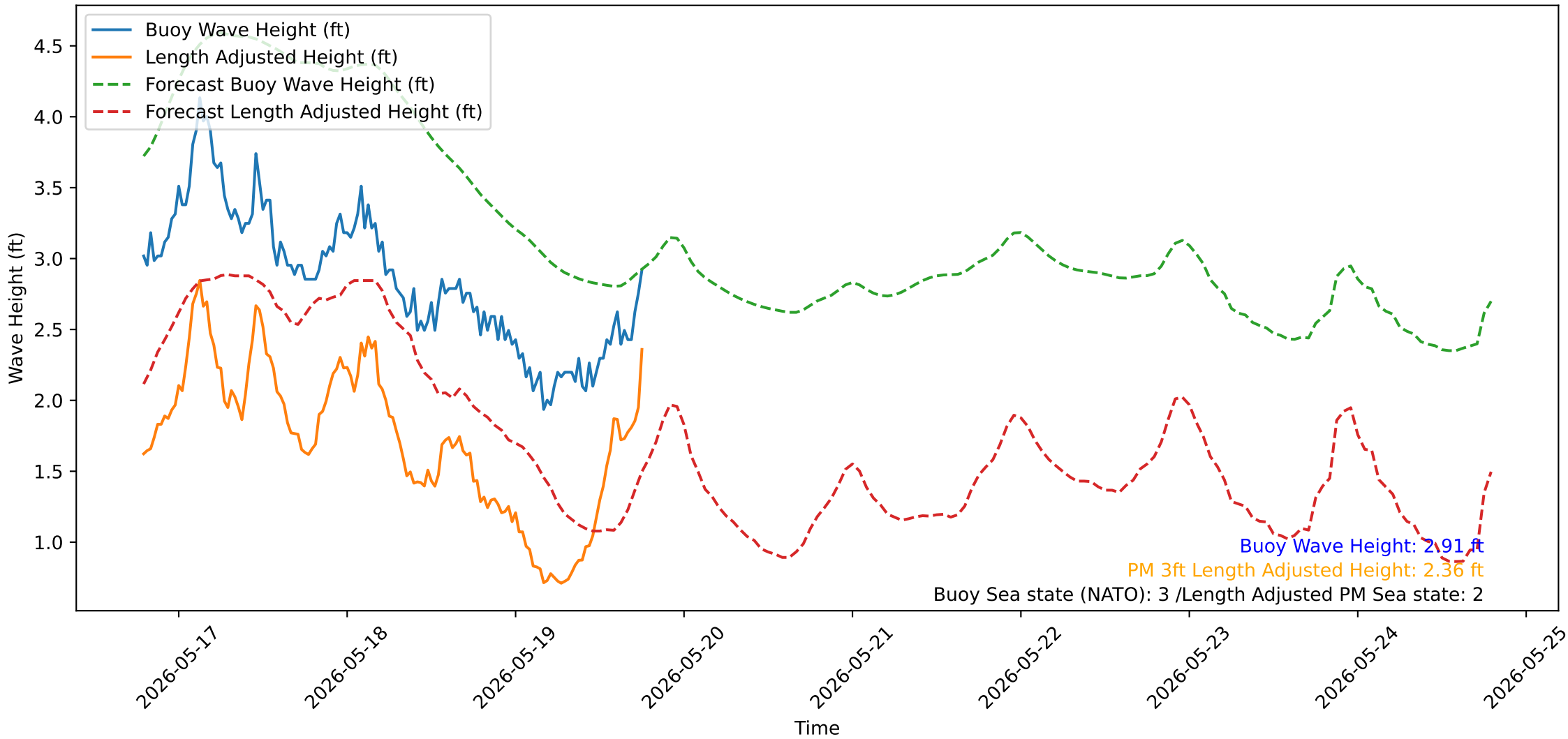
Wave Heights over Time for Red Beach at 2026-05-19 18:50:53
