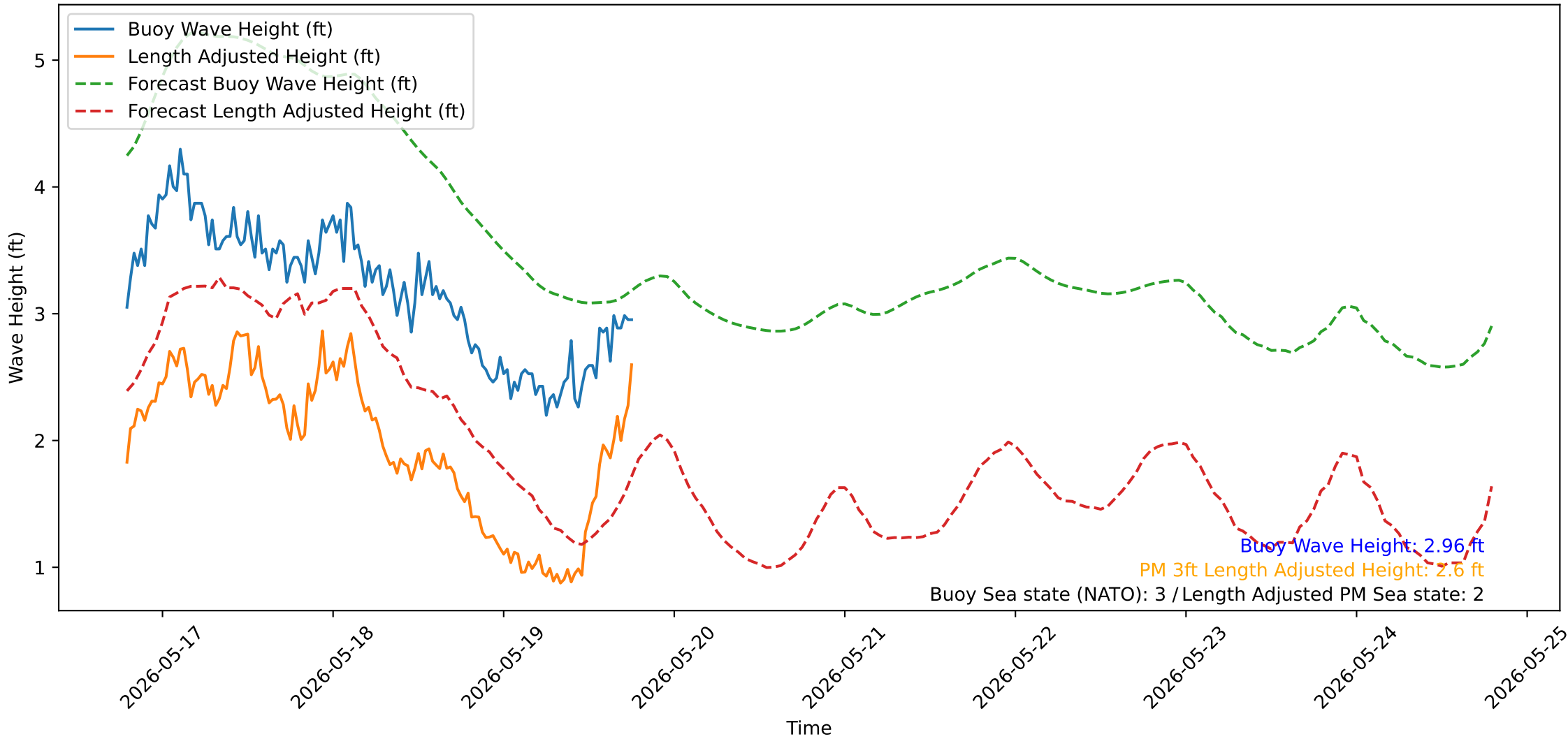
Wave Heights over Time for Oceanside Harbor at 2026-05-19 18:50:32
