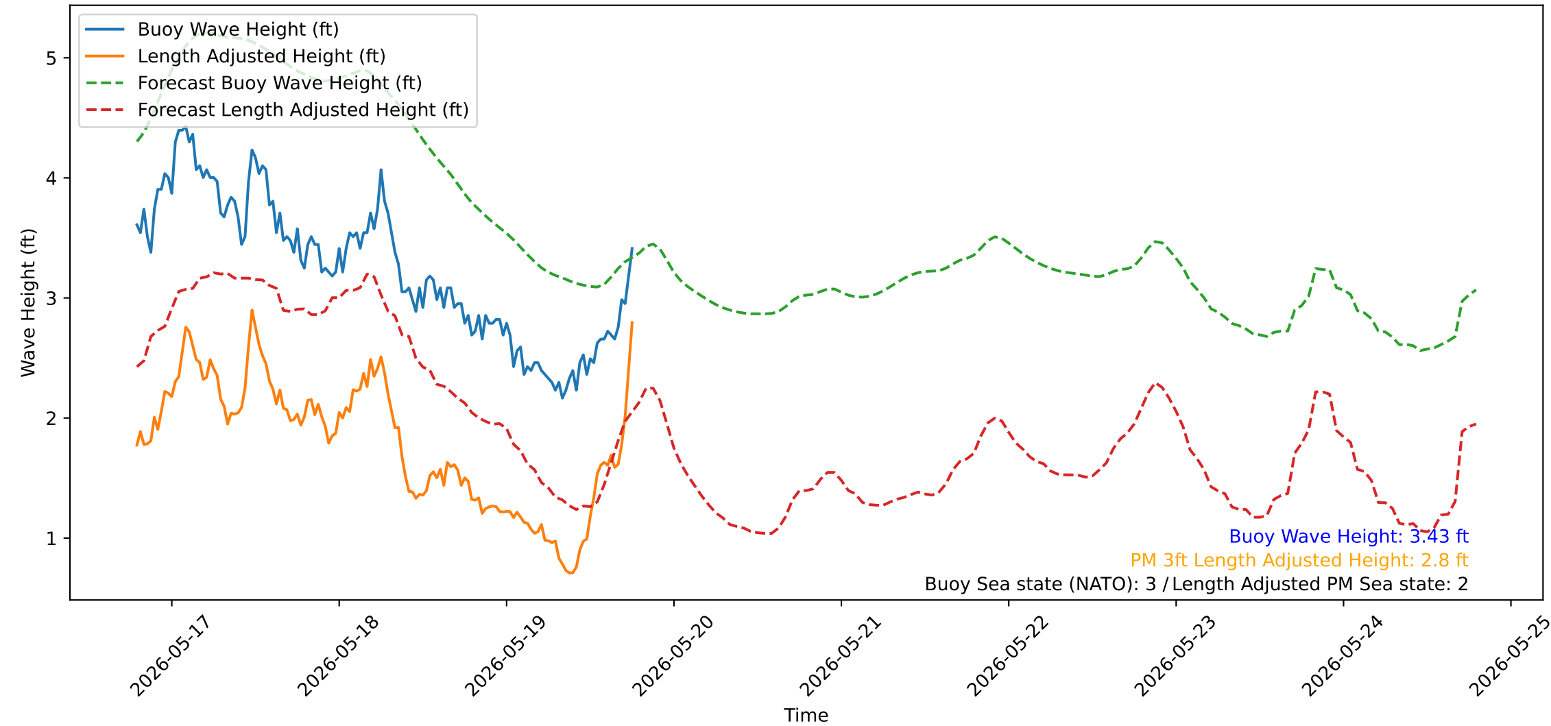
Wave Heights over Time for Green Beach at 2026-05-19 18:51:16
