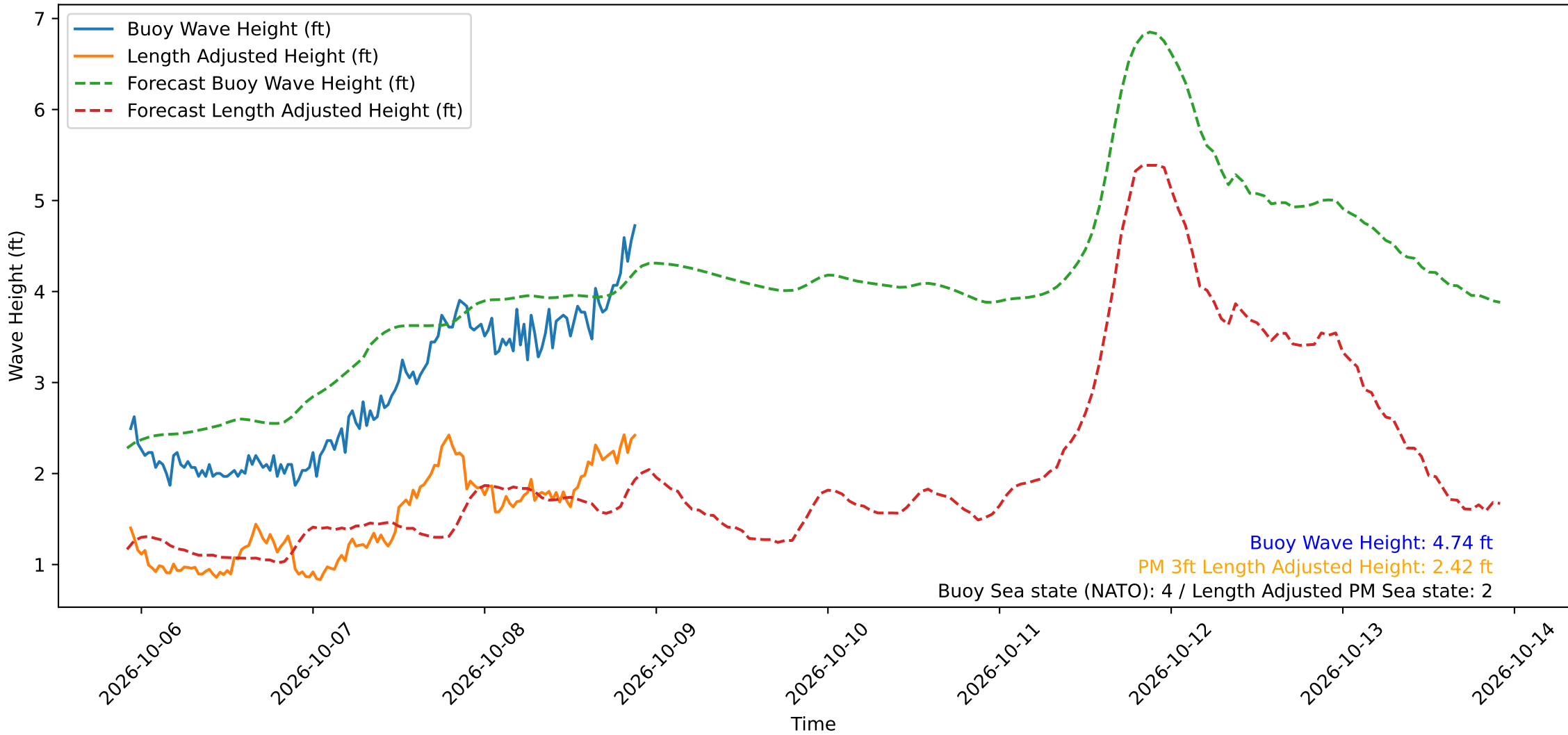
Wave Heights over Time for Red Beach at 2026-10-08 22:00:49
