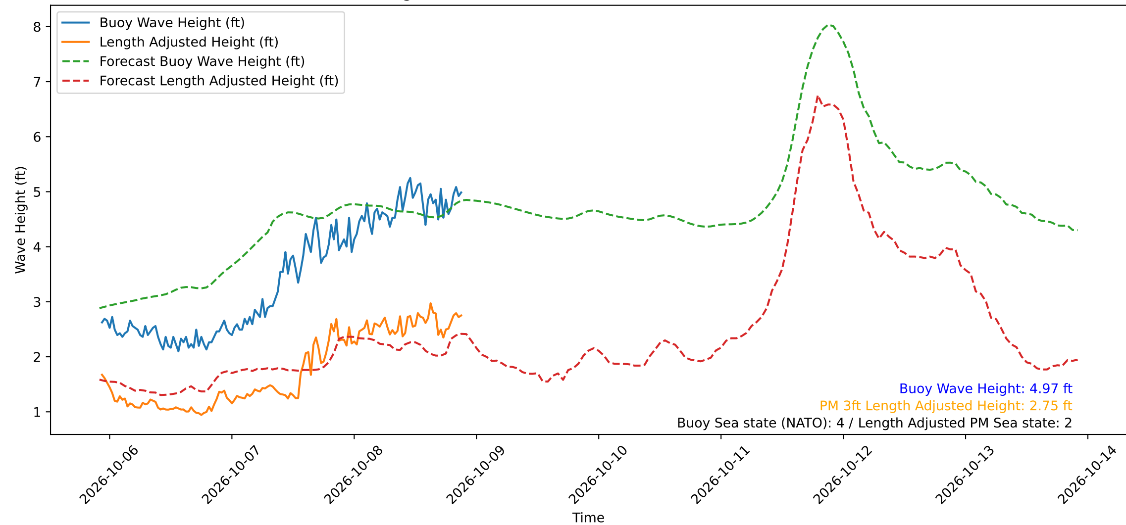
Wave Heights over Time for Green Beach at 2026-10-08 22:01:11
