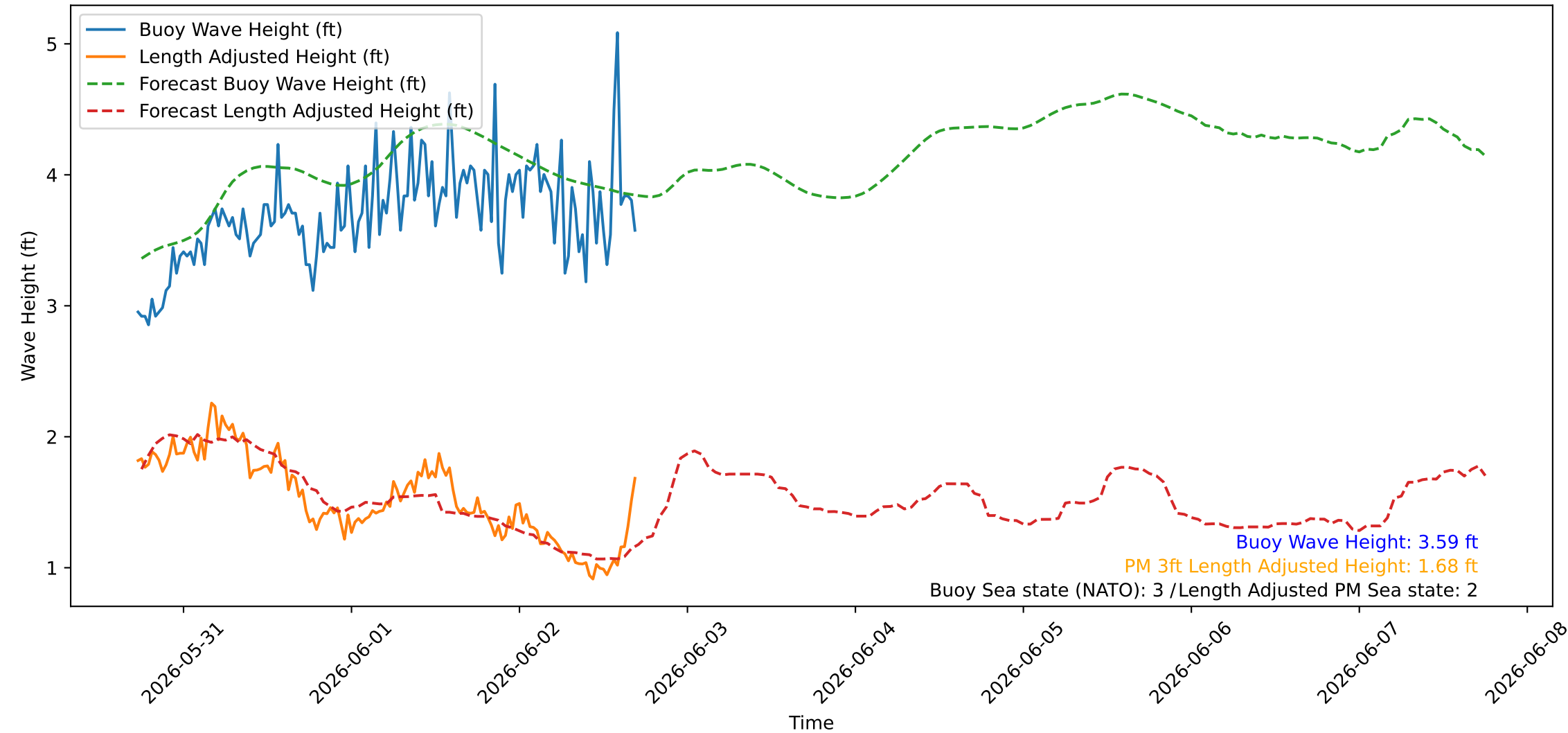
Wave Heights over Time for Oceanside Harbor at 2026-06-02 17:30:26
