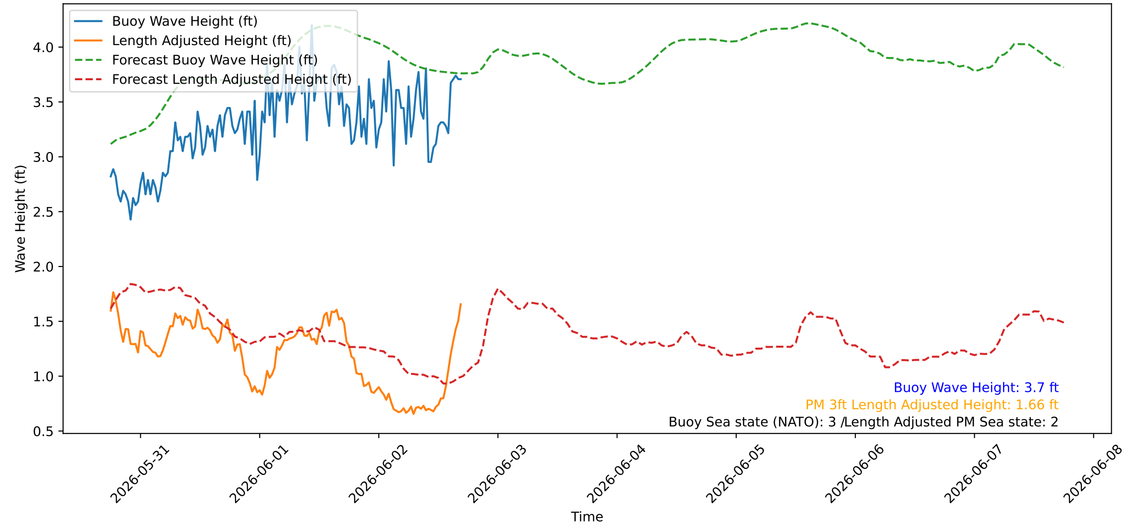
Wave Heights over Time for Red Beach at 2026-06-02 17:30:45
