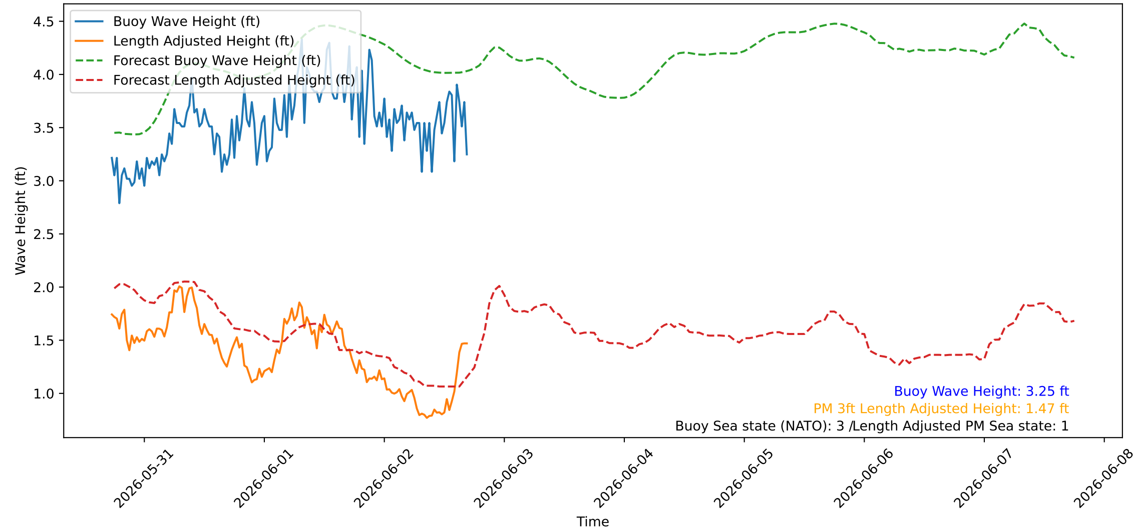
Wave Heights over Time for Green Beach at 2026-06-02 17:31:07
