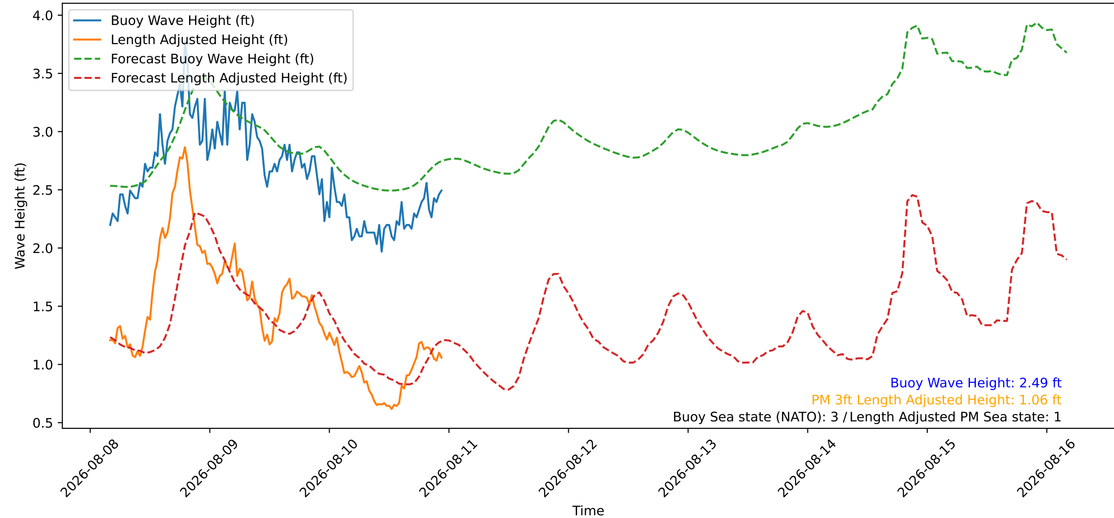
Wave Heights over Time for Green Beach at 2026-08-11 03:51:08
