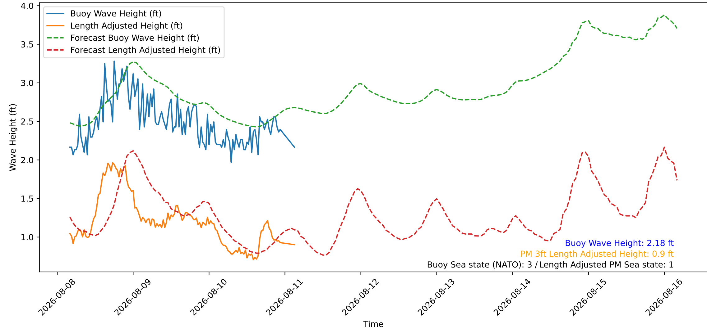
Wave Heights over Time for Oceanside Harbor at 2026-08-11 03:50:26
