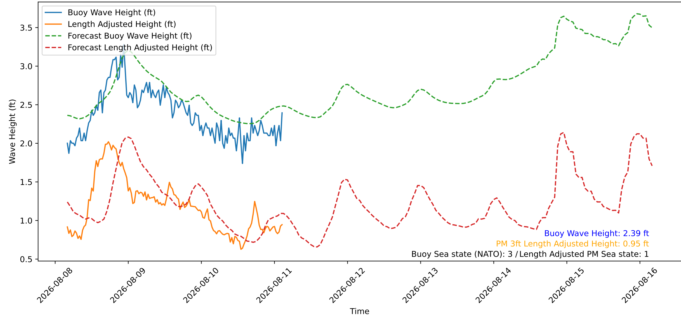
Wave Heights over Time for Red Beach at 2026-08-11 03:50:47
