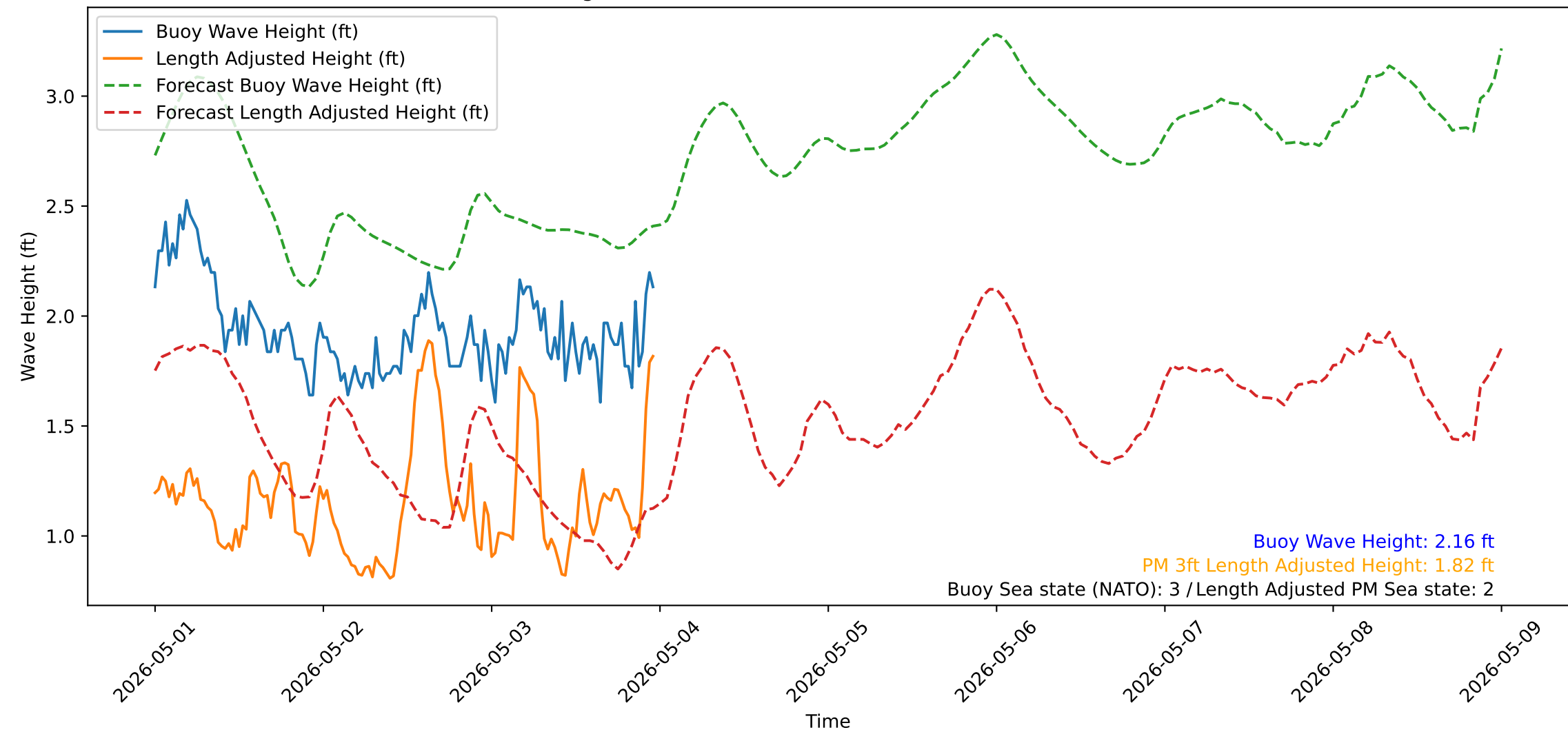
Wave Heights over Time for Red Beach at 2026-05-03 23:50:52
