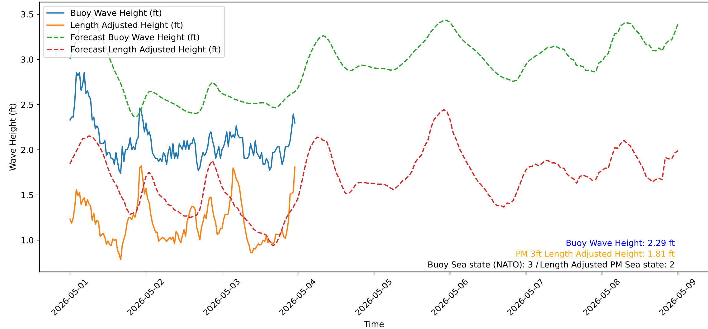
Wave Heights over Time for Green Beach at 2026-05-03 23:51:14
