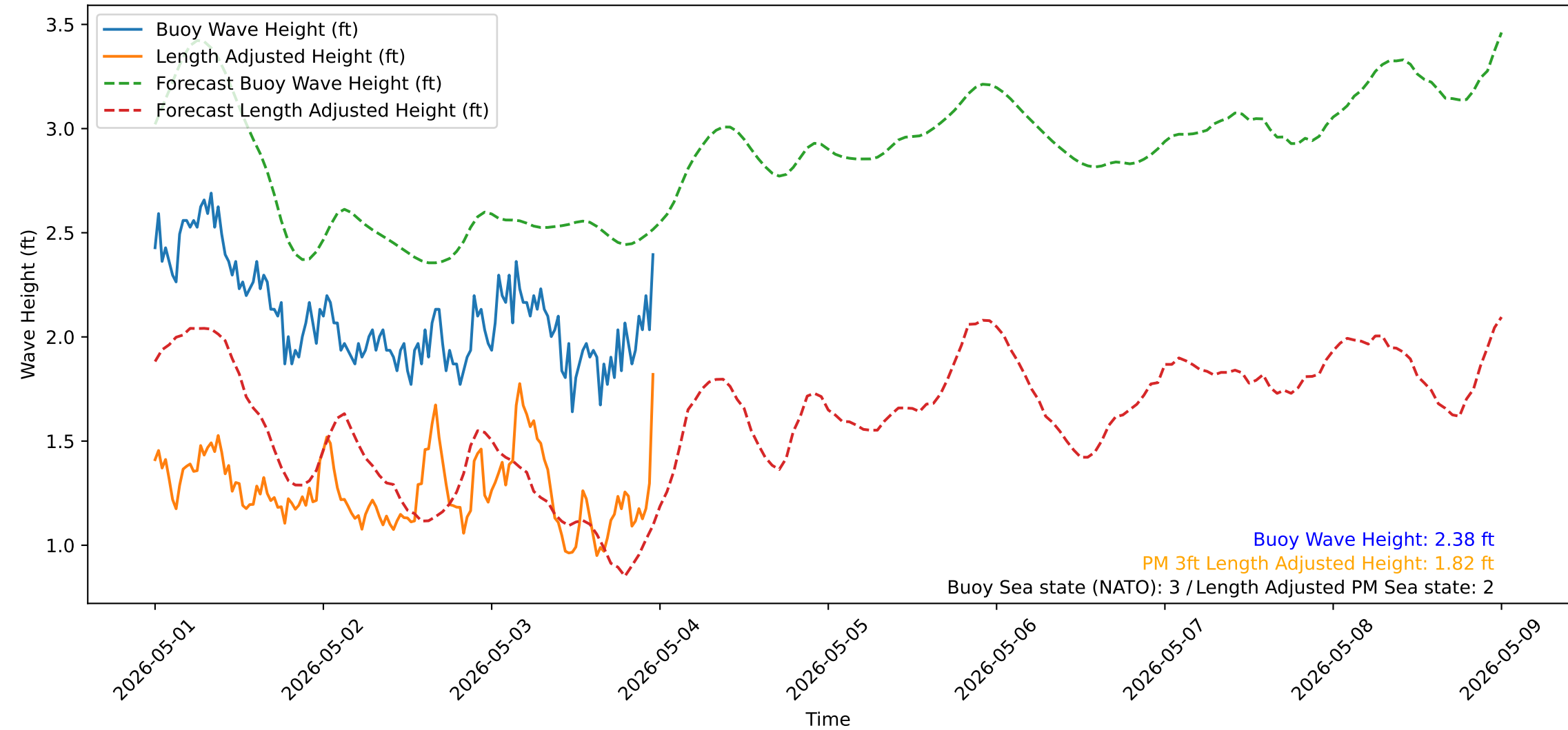
Wave Heights over Time for Oceanside Harbor at 2026-05-03 23:50:32
