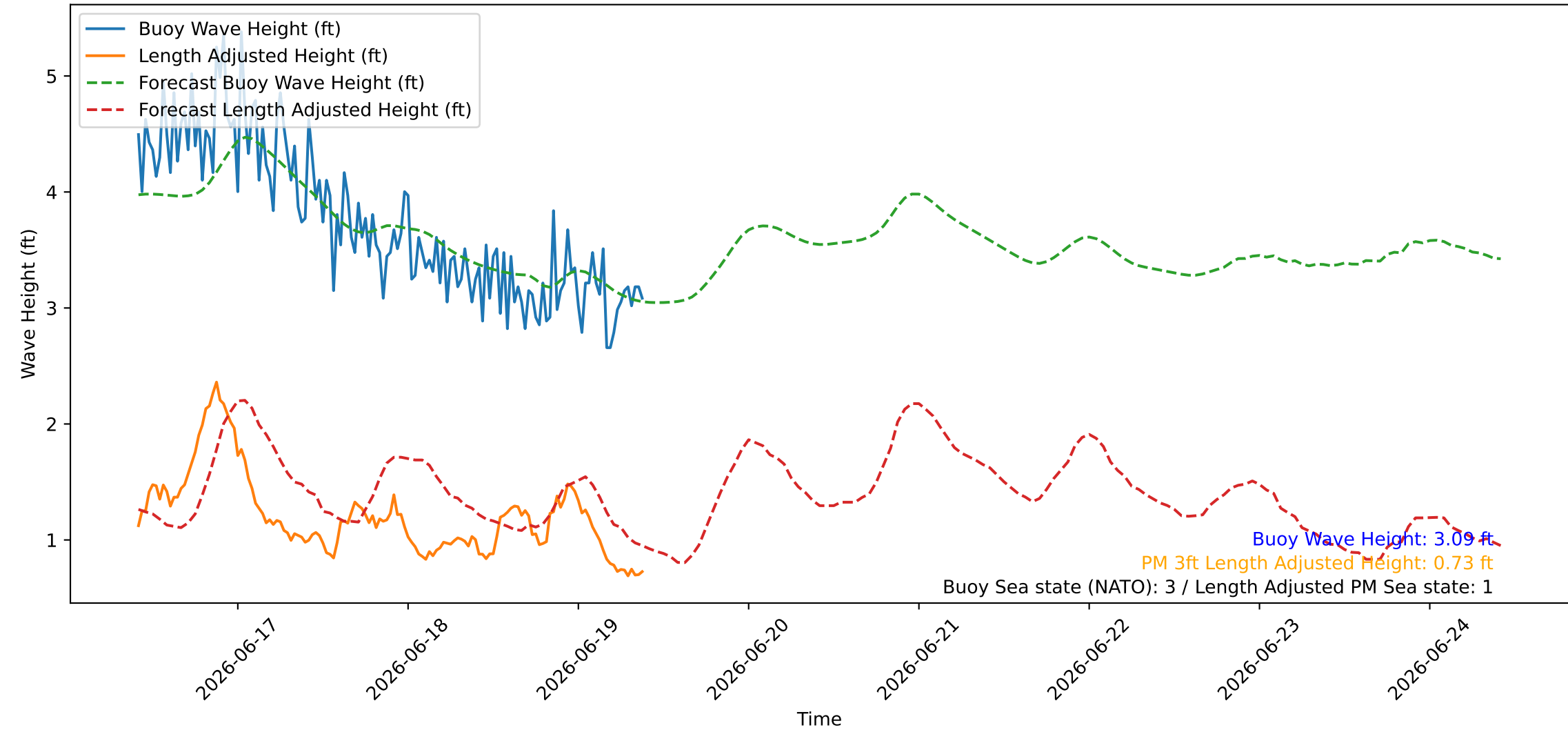
Wave Heights over Time for Red Beach at 2026-06-19 09:50:46
