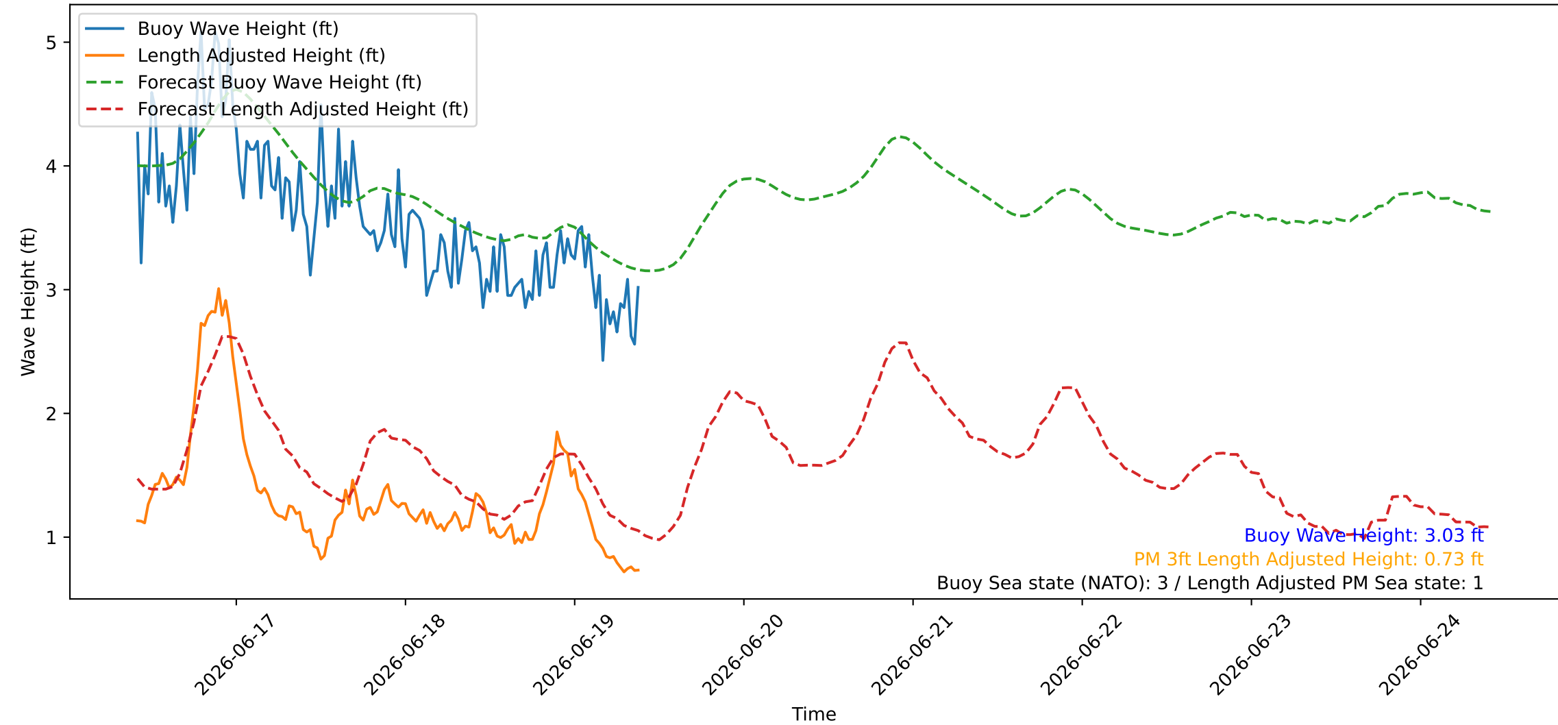
Wave Heights over Time for Green Beach at 2026-06-19 09:51:09
