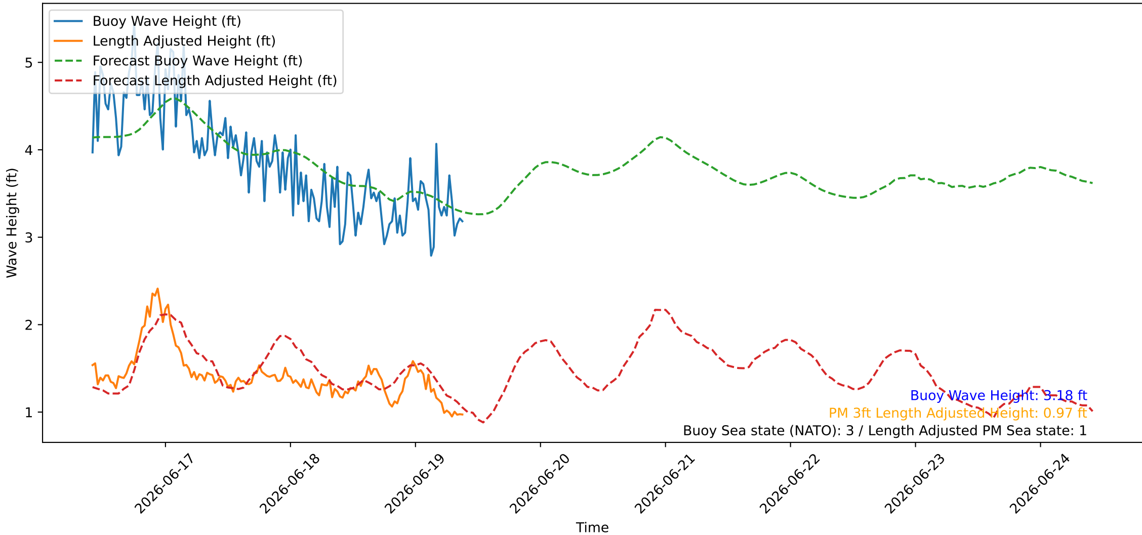
Wave Heights over Time for Oceanside Harbor at 2026-06-19 09:50:26
