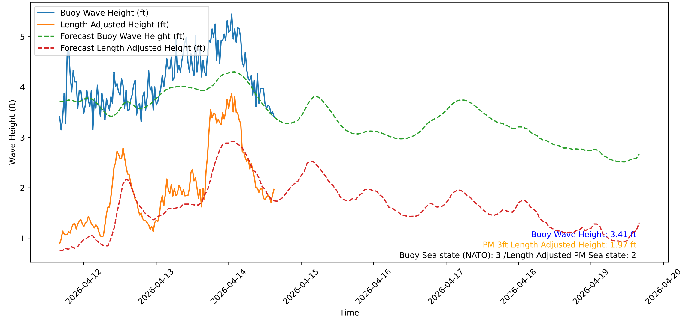
Wave Heights over Time for Oceanside Harbor at 2026-04-14 16:10:31
