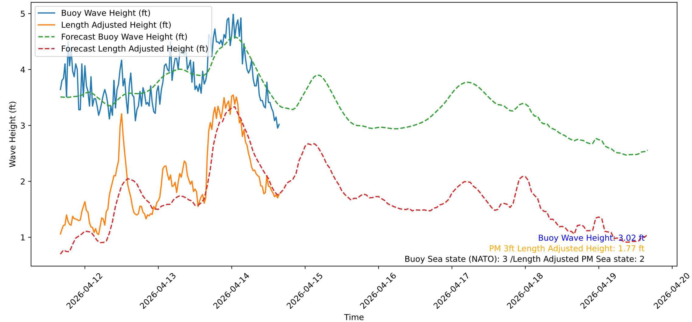
Wave Heights over Time for Green Beach at 2026-04-14 16:11:13
