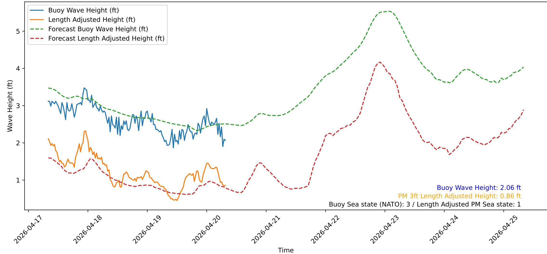
Wave Heights over Time for Green Beach at 2026-04-20 08:11:13
