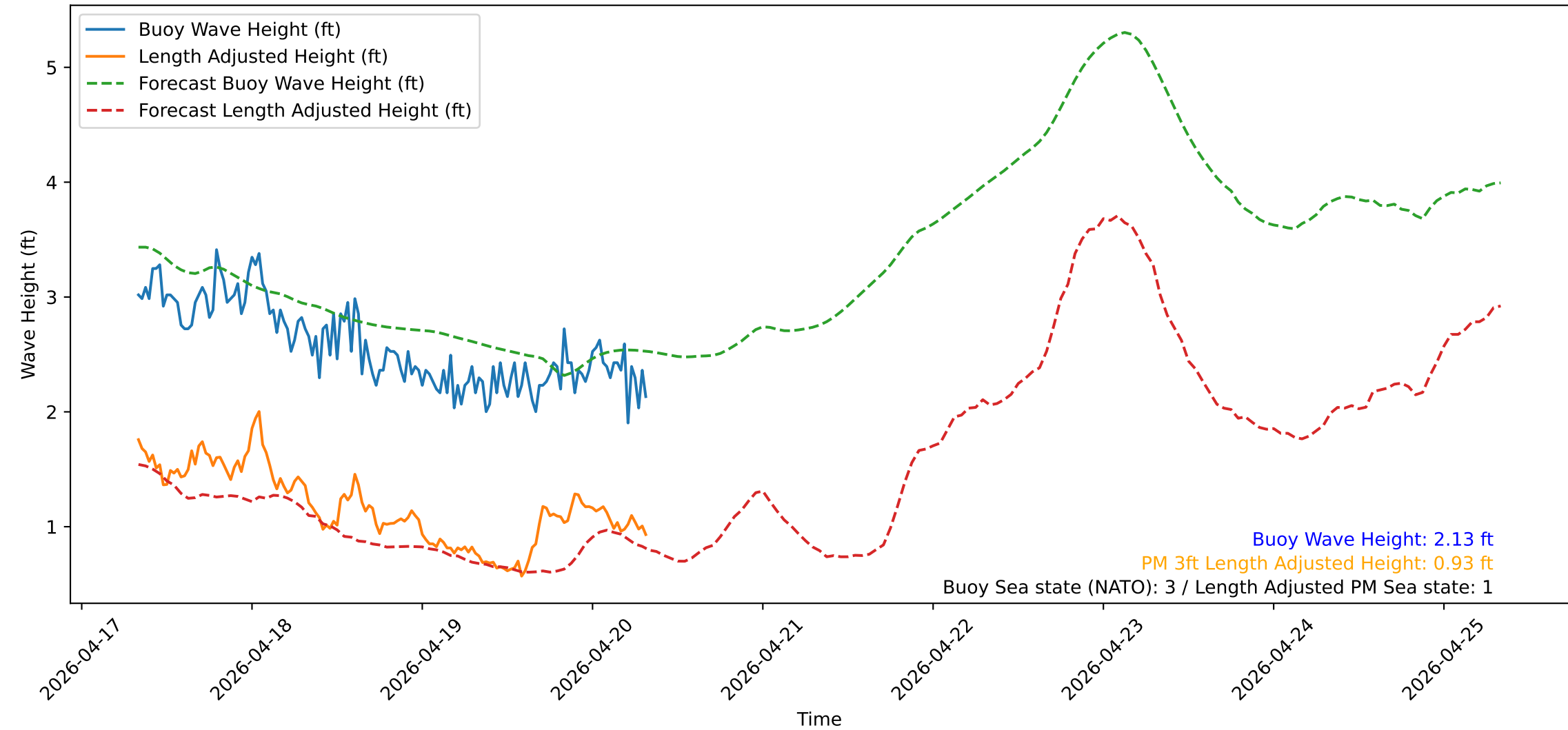
Wave Heights over Time for Oceanside Harbor at 2026-04-20 08:10:32
