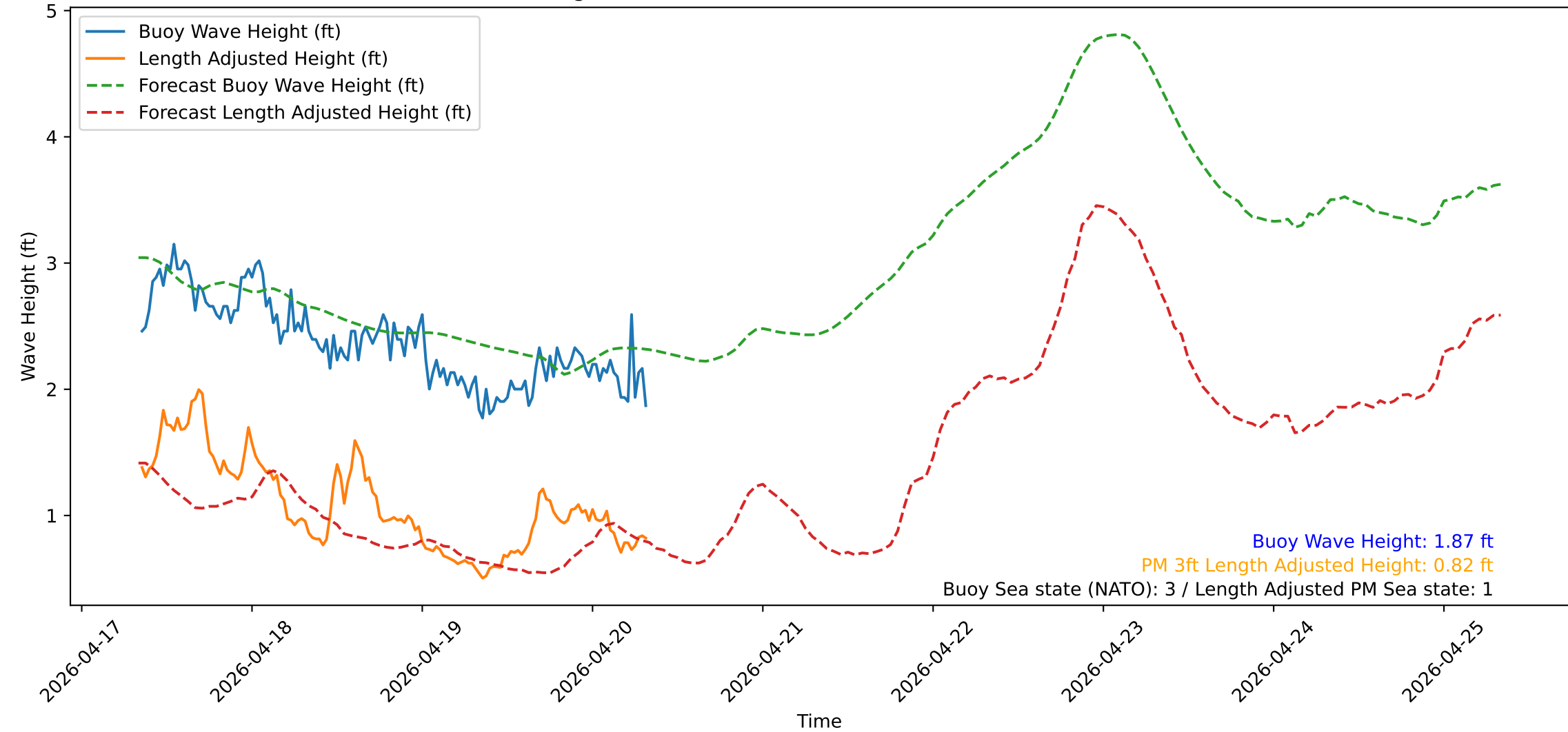
Wave Heights over Time for Red Beach at 2026-04-20 08:10:51
