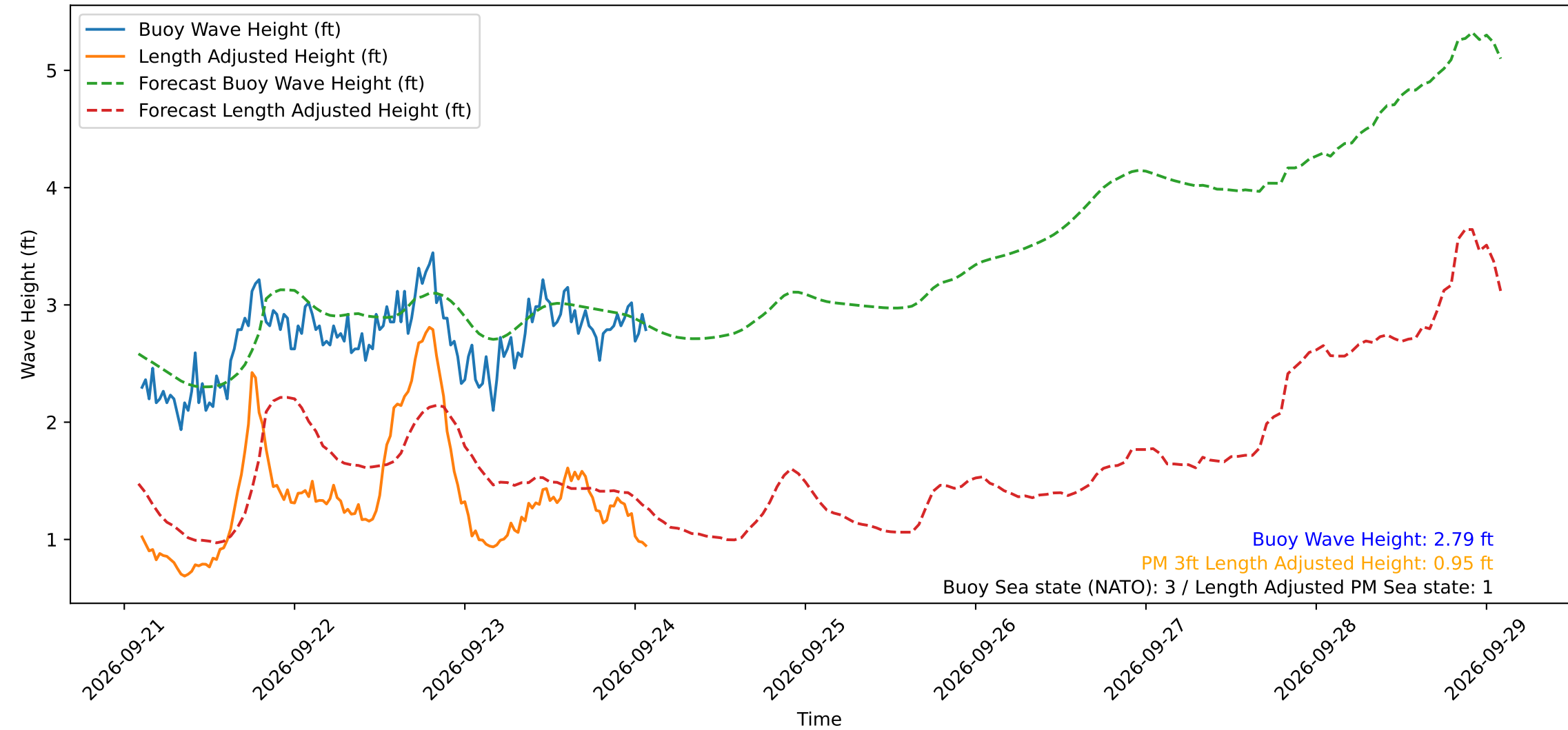
Wave Heights over Time for Green Beach at 2026-09-24 02:21:14
