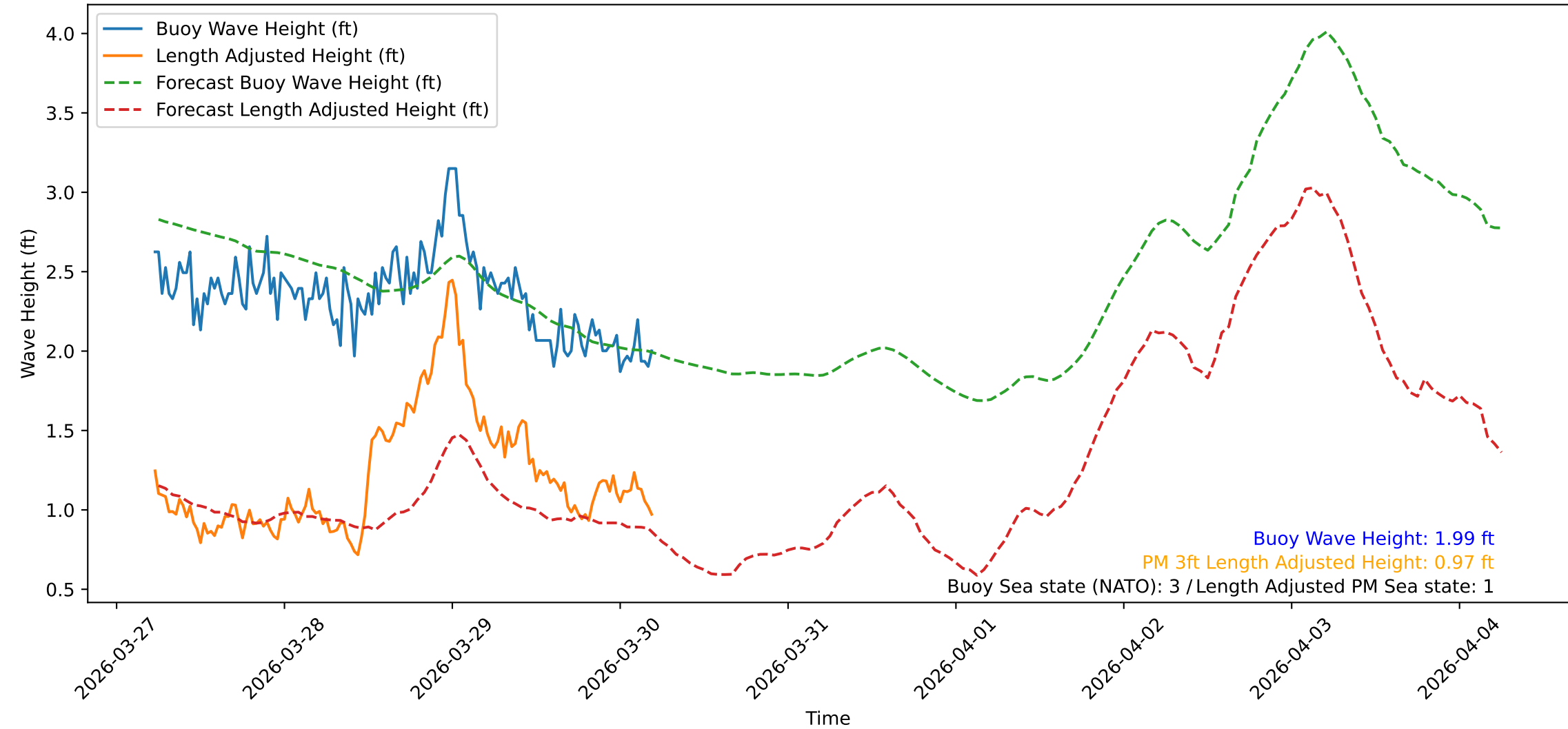
Wave Heights over Time for Oceanside Harbor at 2026-03-30 05:40:31
