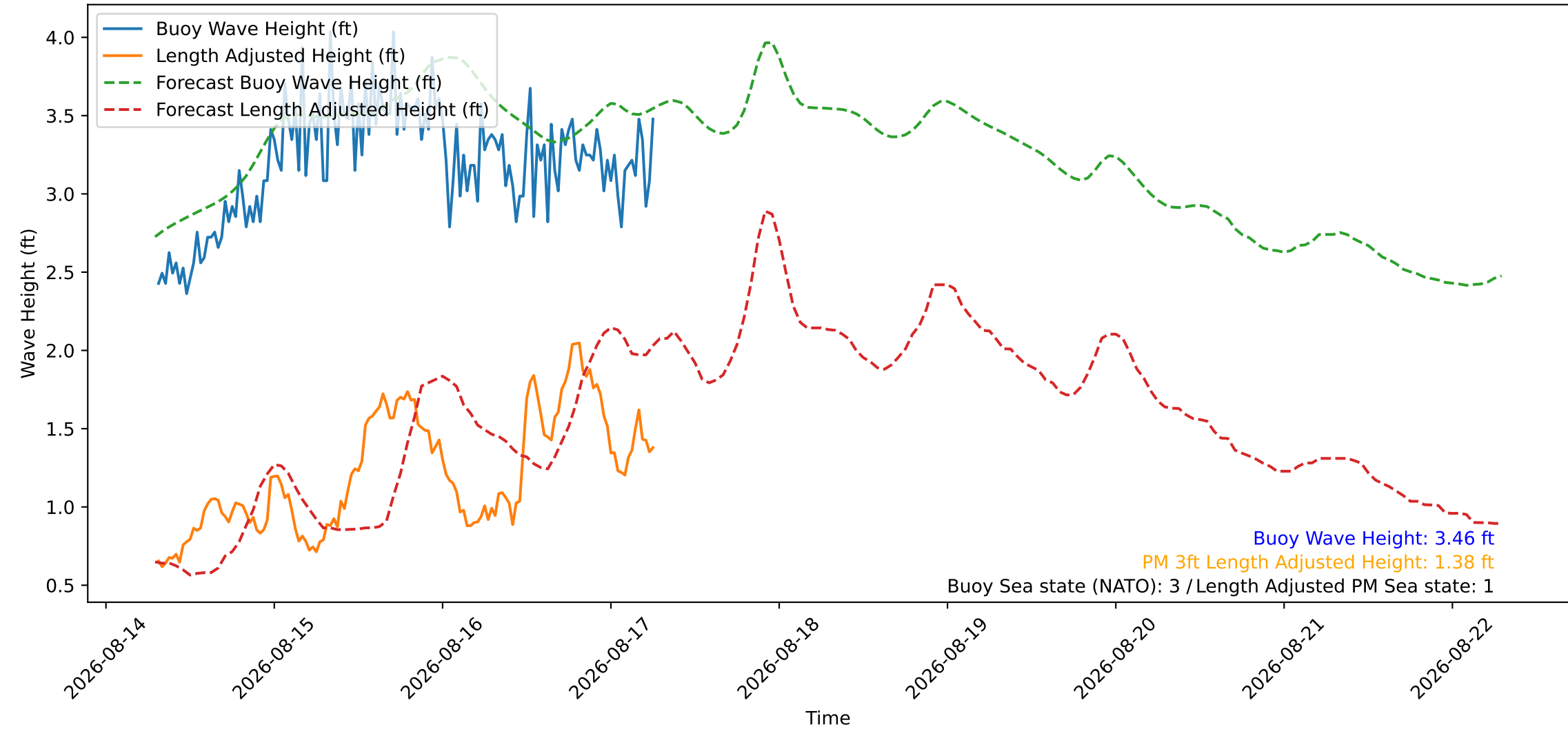
Wave Heights over Time for Red Beach at 2026-08-17 07:00:46
