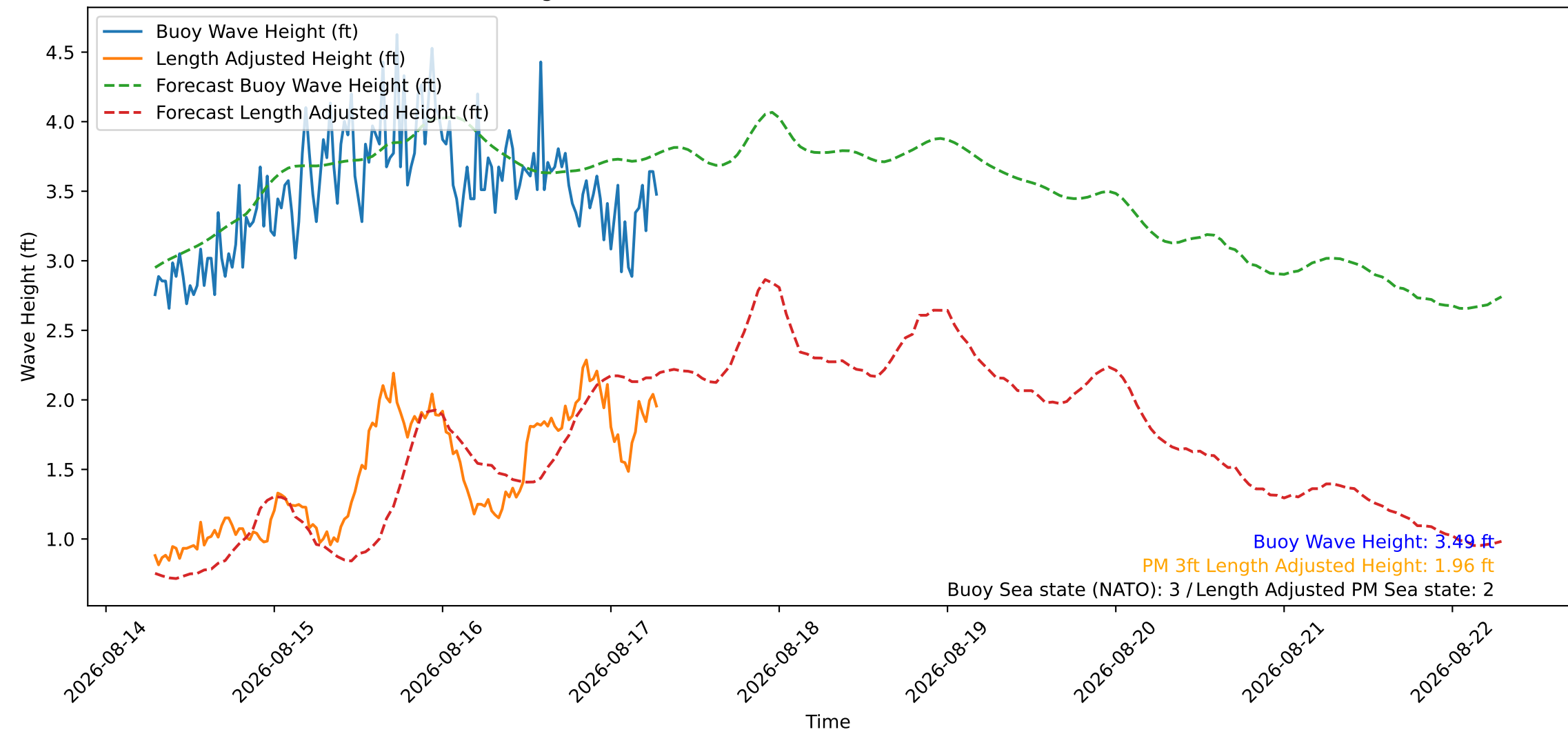
Wave Heights over Time for Oceanside Harbor at 2026-08-17 07:00:27
