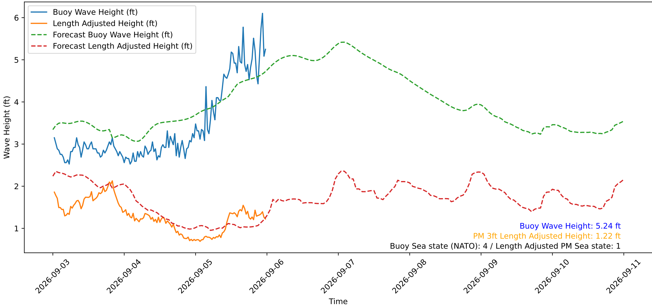
Wave Heights over Time for Red Beach at 2026-09-06 00:10:50
