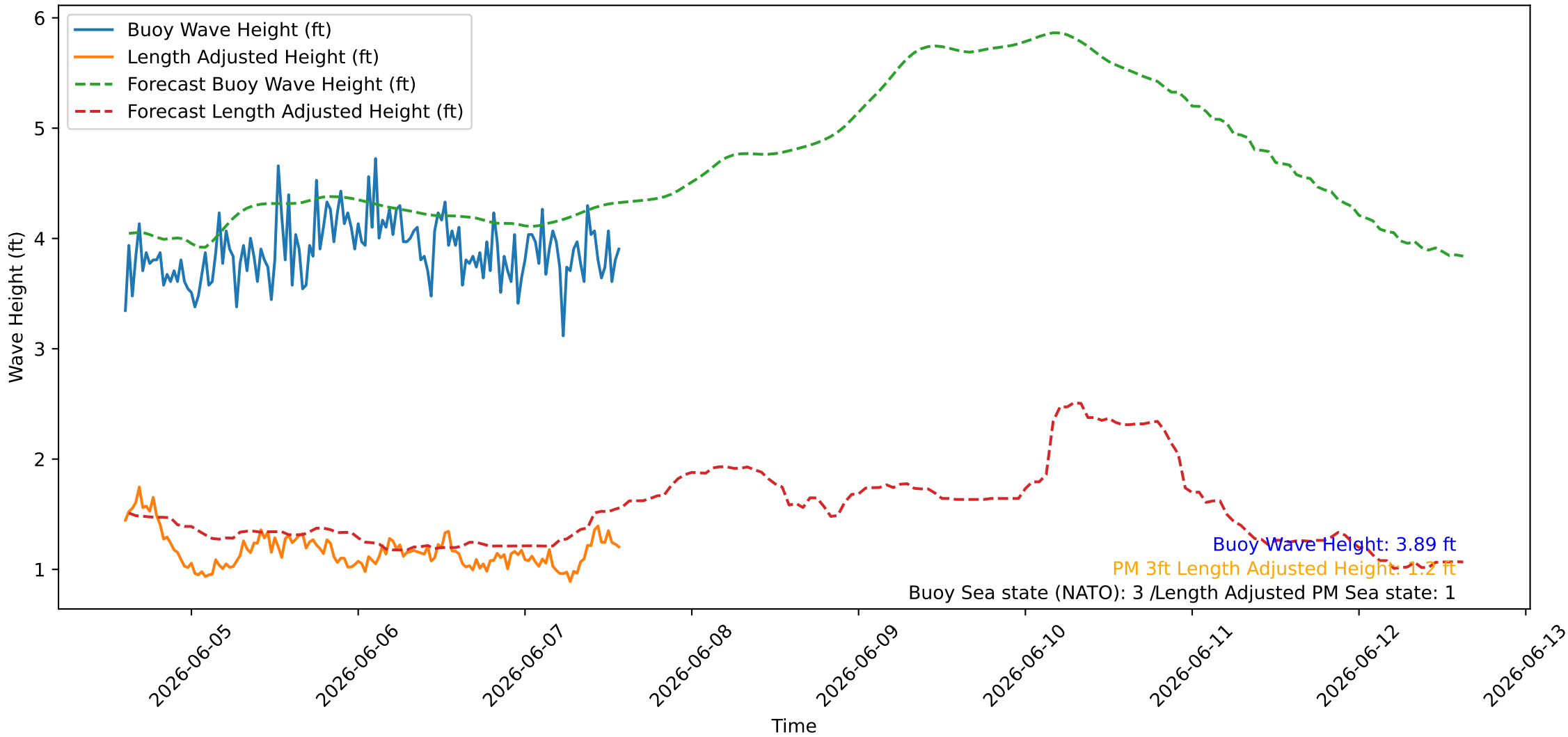
Wave Heights over Time for Green Beach at 2026-06-07 14:31:08
