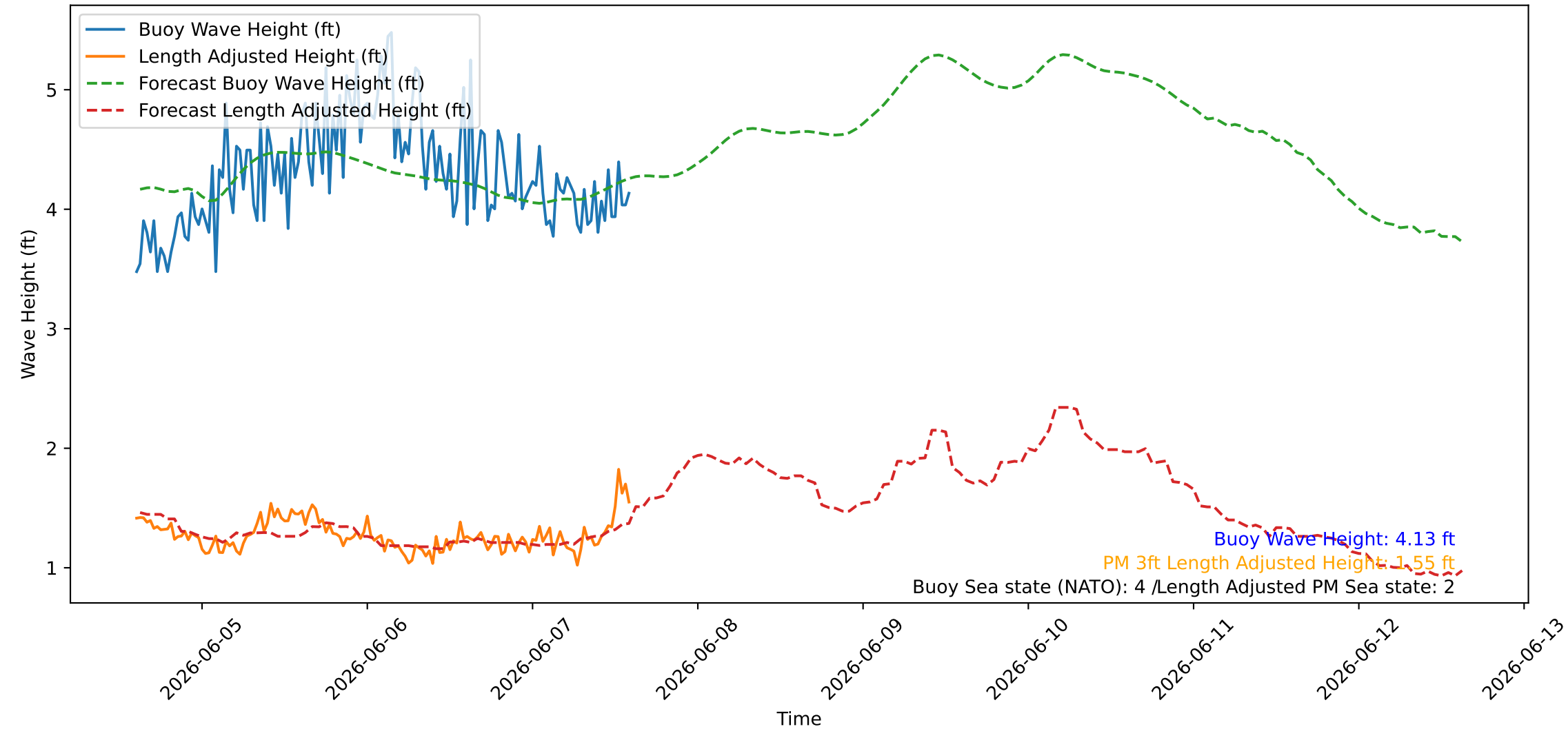
Wave Heights over Time for Oceanside Harbor at 2026-06-07 14:30:26
