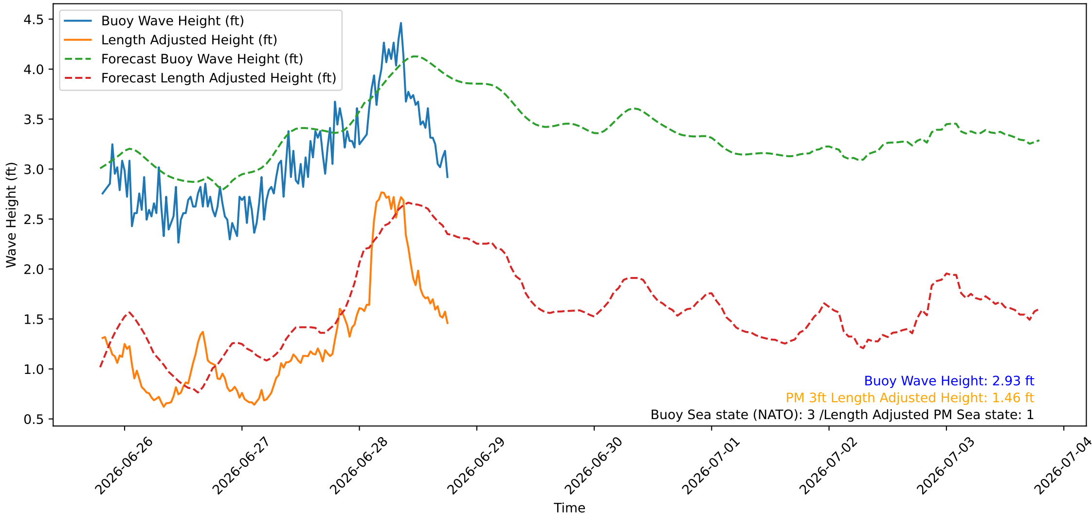
Wave Heights over Time for Red Beach at 2026-06-28 19:00:45
