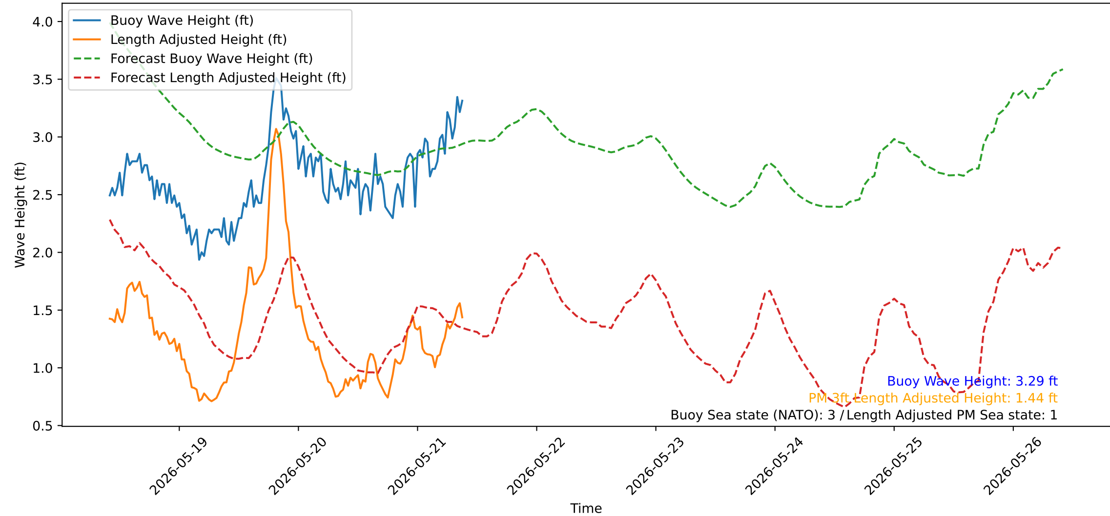
Wave Heights over Time for Red Beach at 2026-05-21 09:40:51
