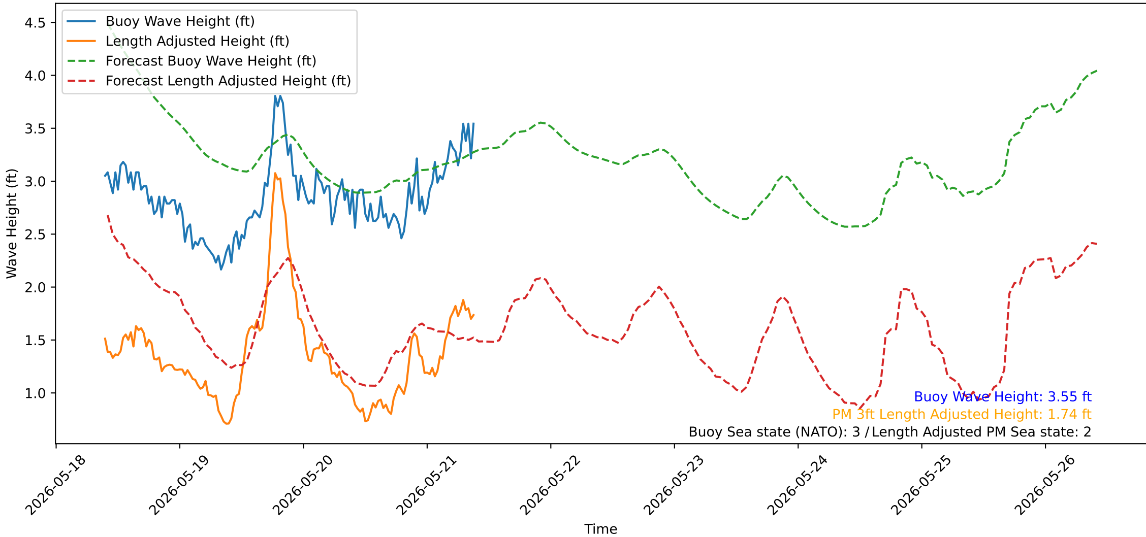
Wave Heights over Time for Green Beach at 2026-05-21 09:41:13
