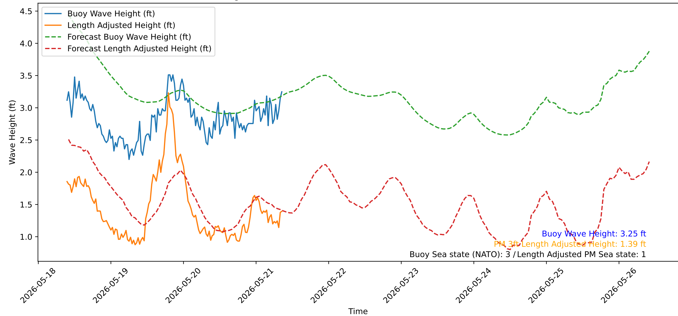
Wave Heights over Time for Oceanside Harbor at 2026-05-21 09:40:31
