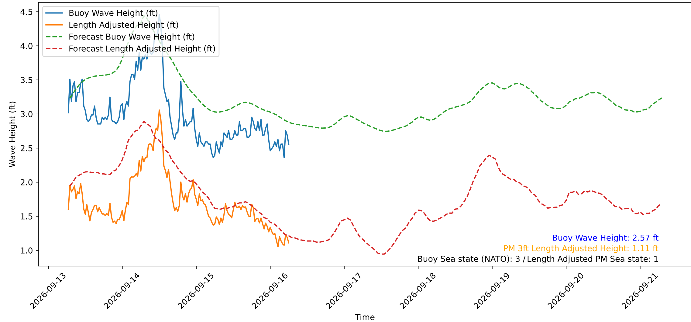
Wave Heights over Time for Oceanside Harbor at 2026-09-16 06:30:30
