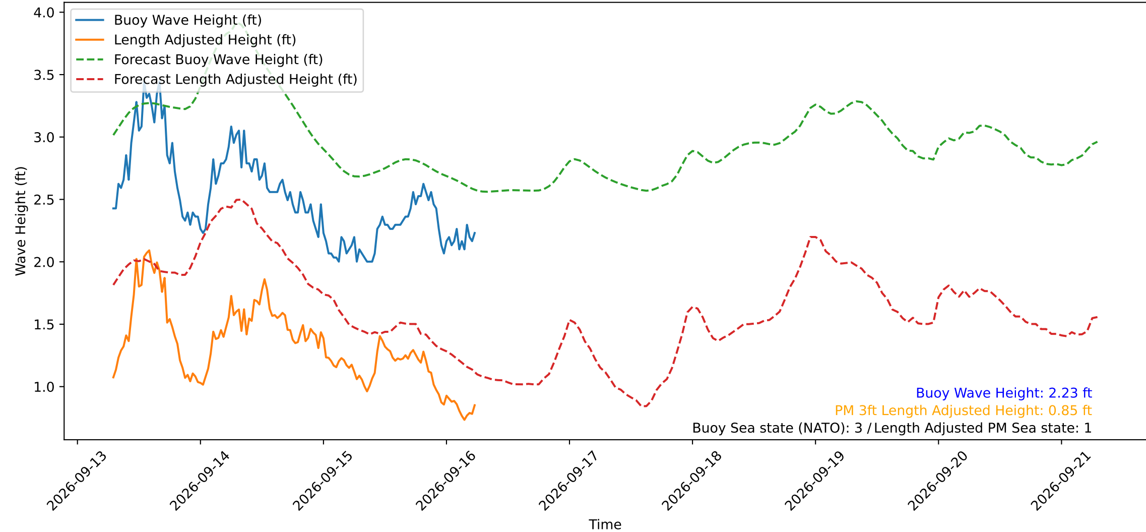
Wave Heights over Time for Red Beach at 2026-09-16 06:30:50
