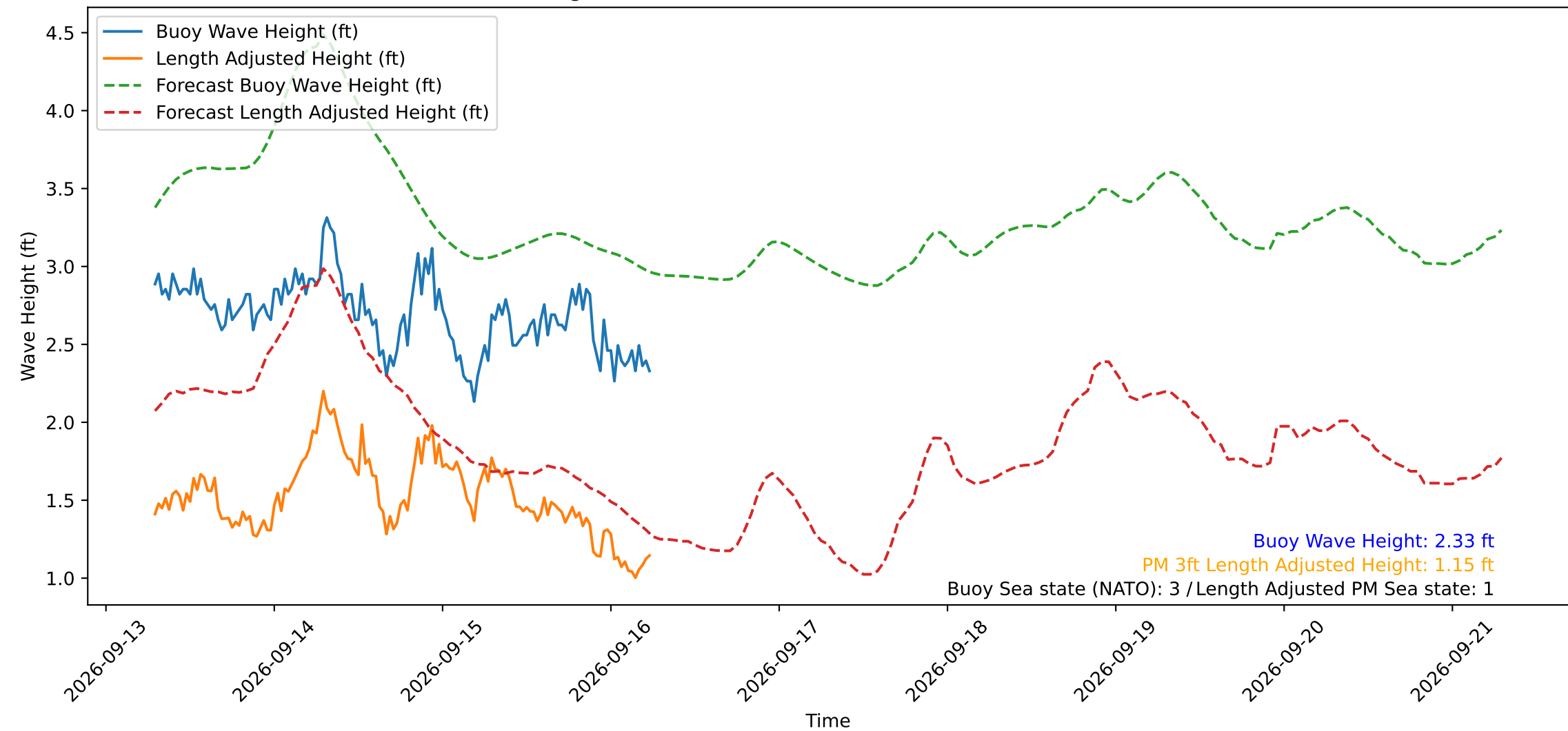
Wave Heights over Time for Green Beach at 2026-09-16 06:31:12
