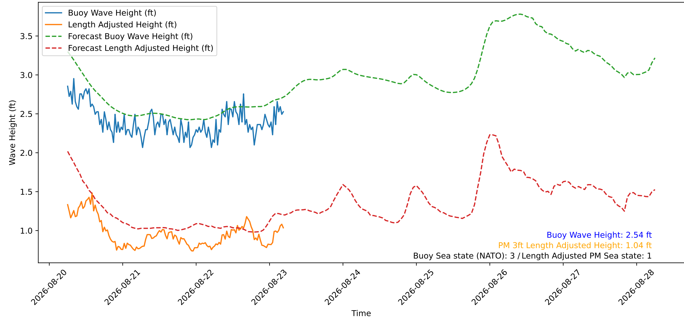
Wave Heights over Time for Red Beach at 2026-08-23 05:30:49
