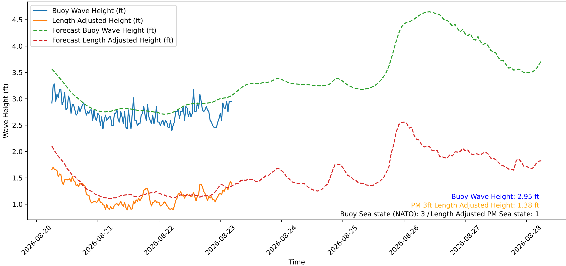
Wave Heights over Time for Green Beach at 2026-08-23 05:31:11
