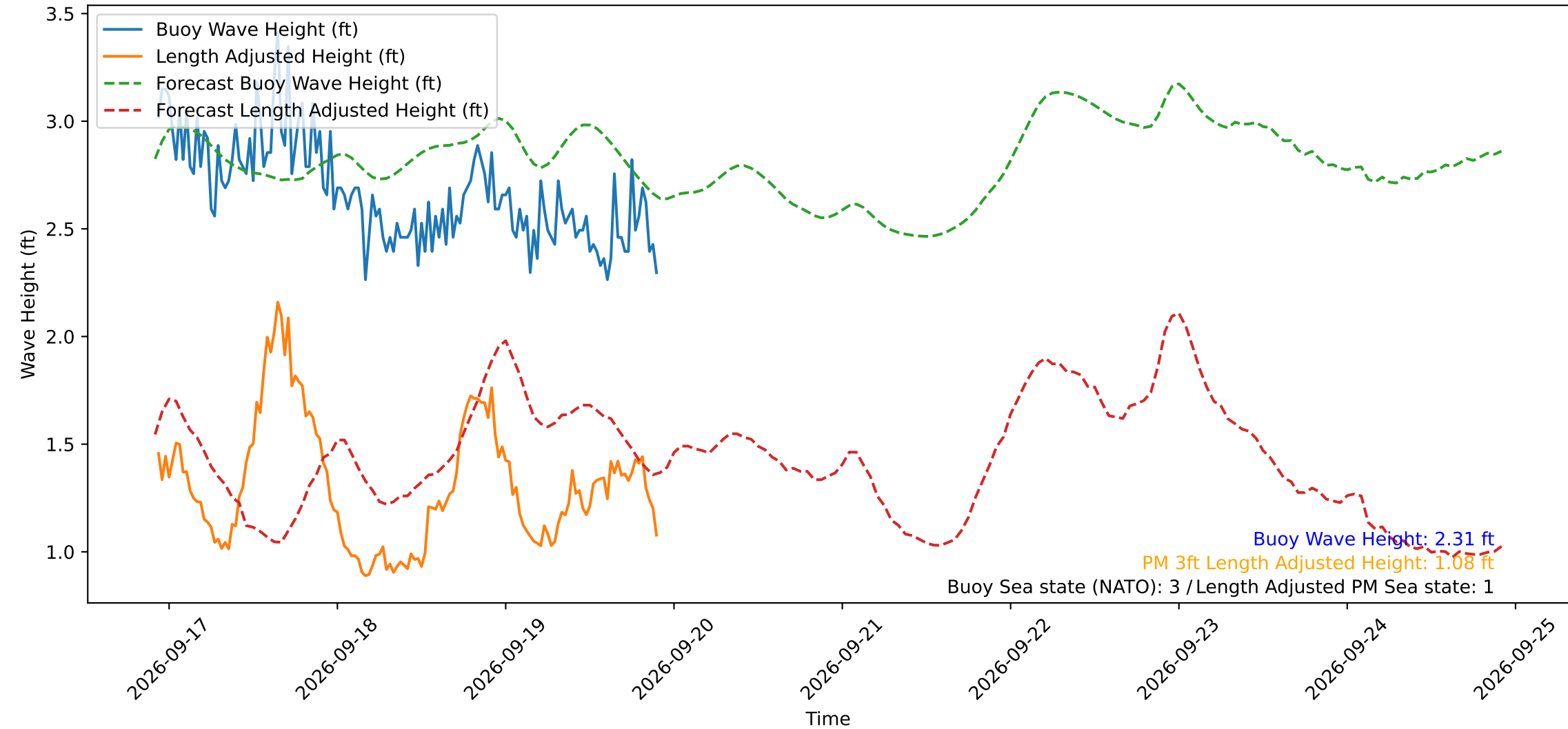
Wave Heights over Time for Red Beach at 2026-09-19 22:10:49
