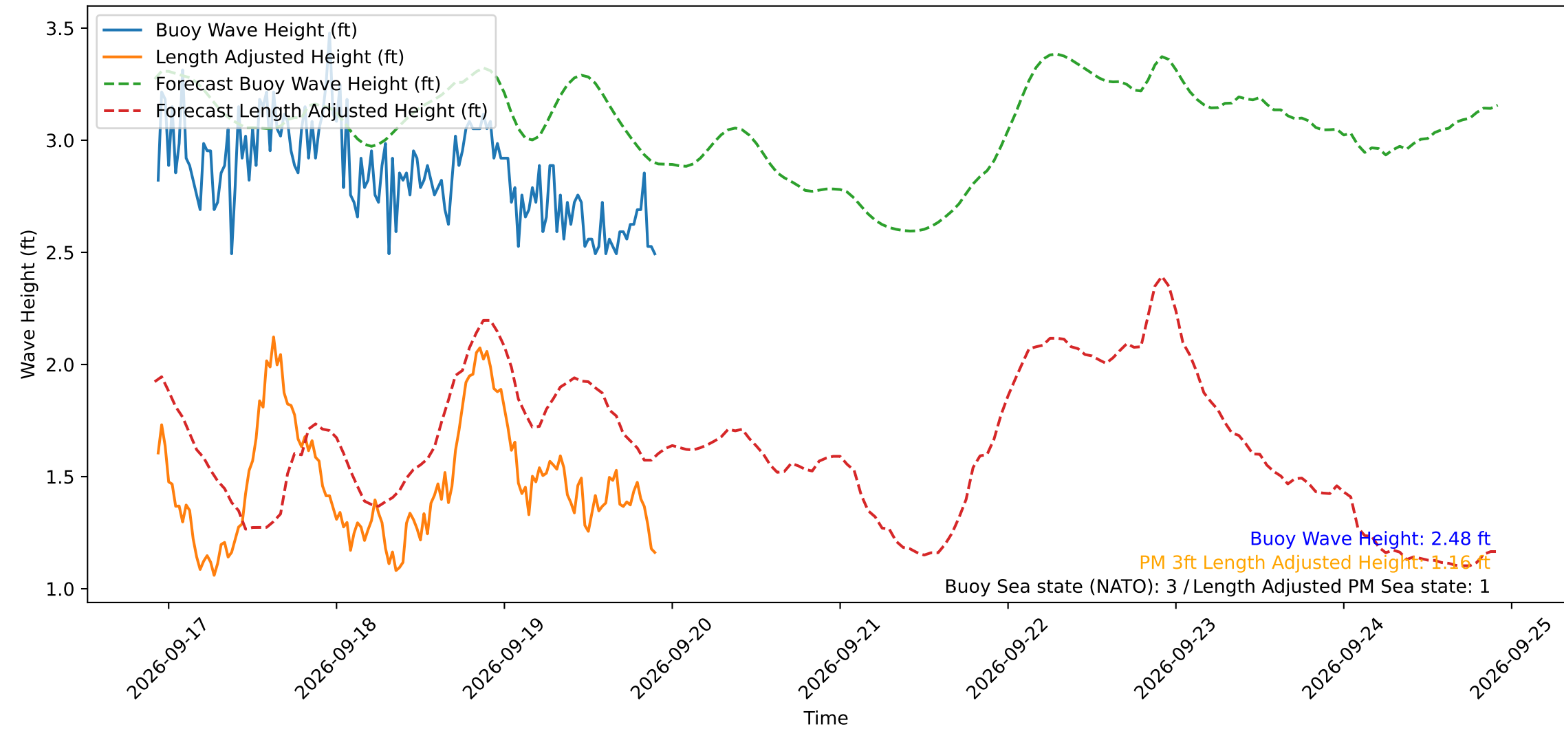
Wave Heights over Time for Green Beach at 2026-09-19 22:11:11
