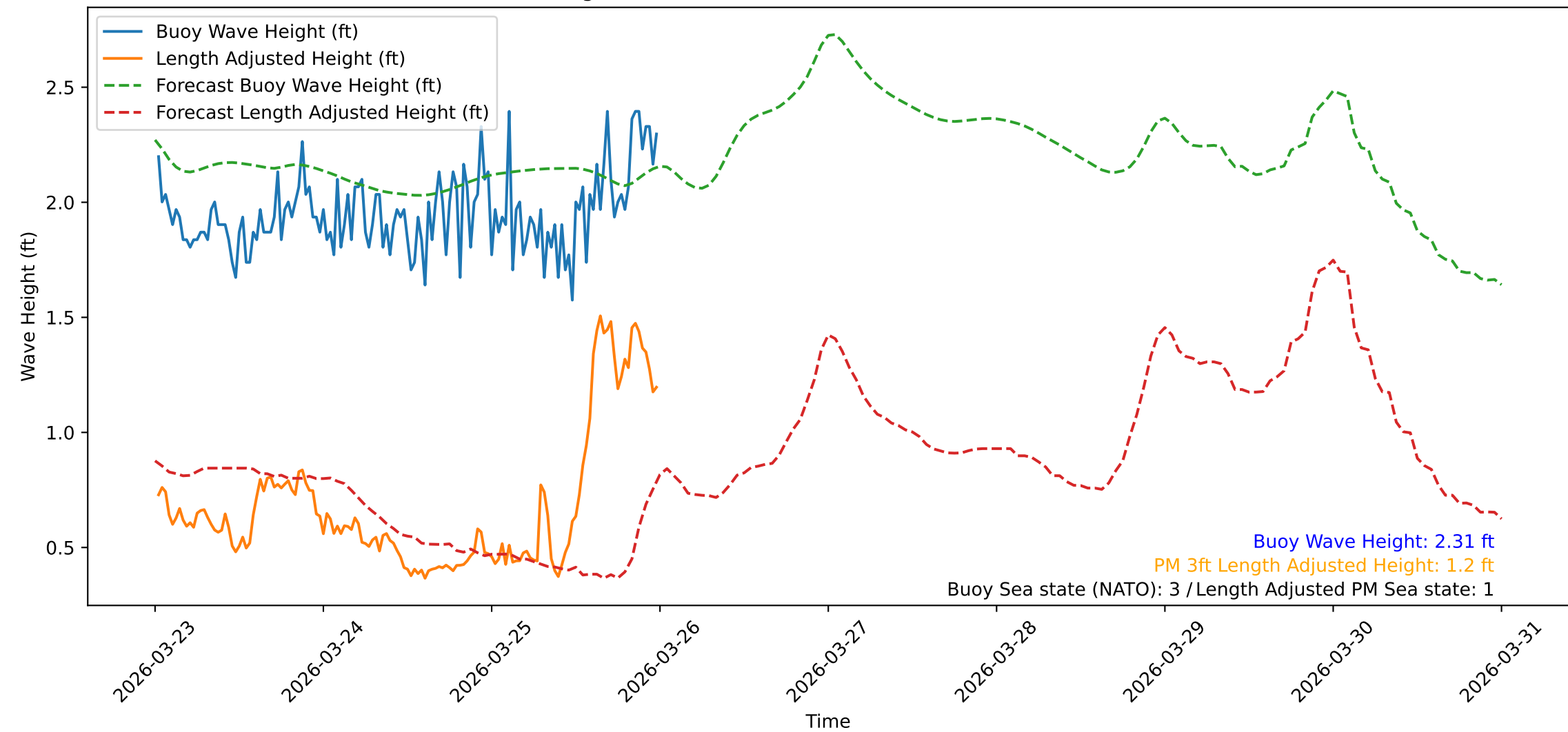
Wave Heights over Time for Red Beach at 2026-03-26 00:20:48
