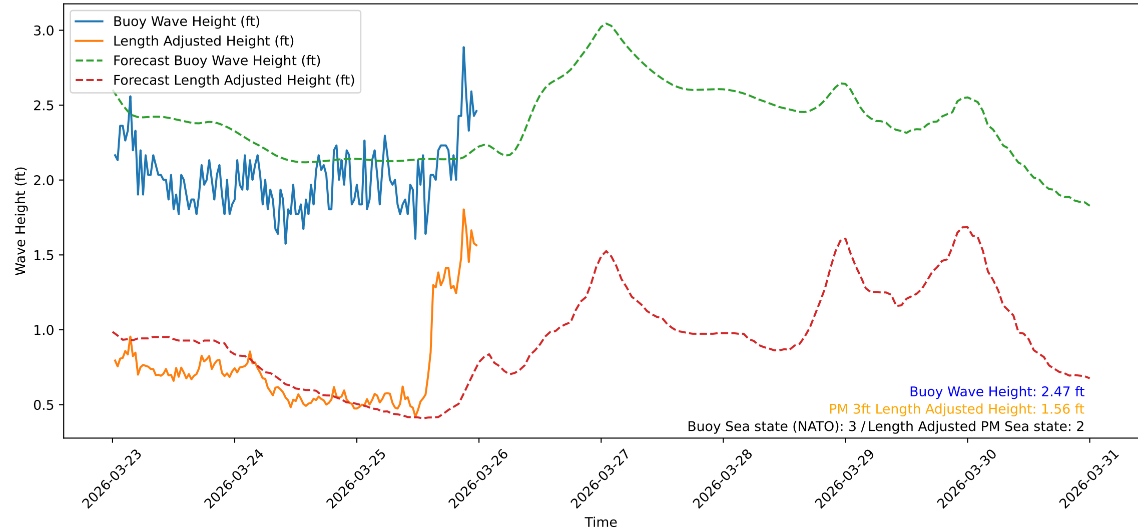
Wave Heights over Time for Oceanside Harbor at 2026-03-26 00:20:31
