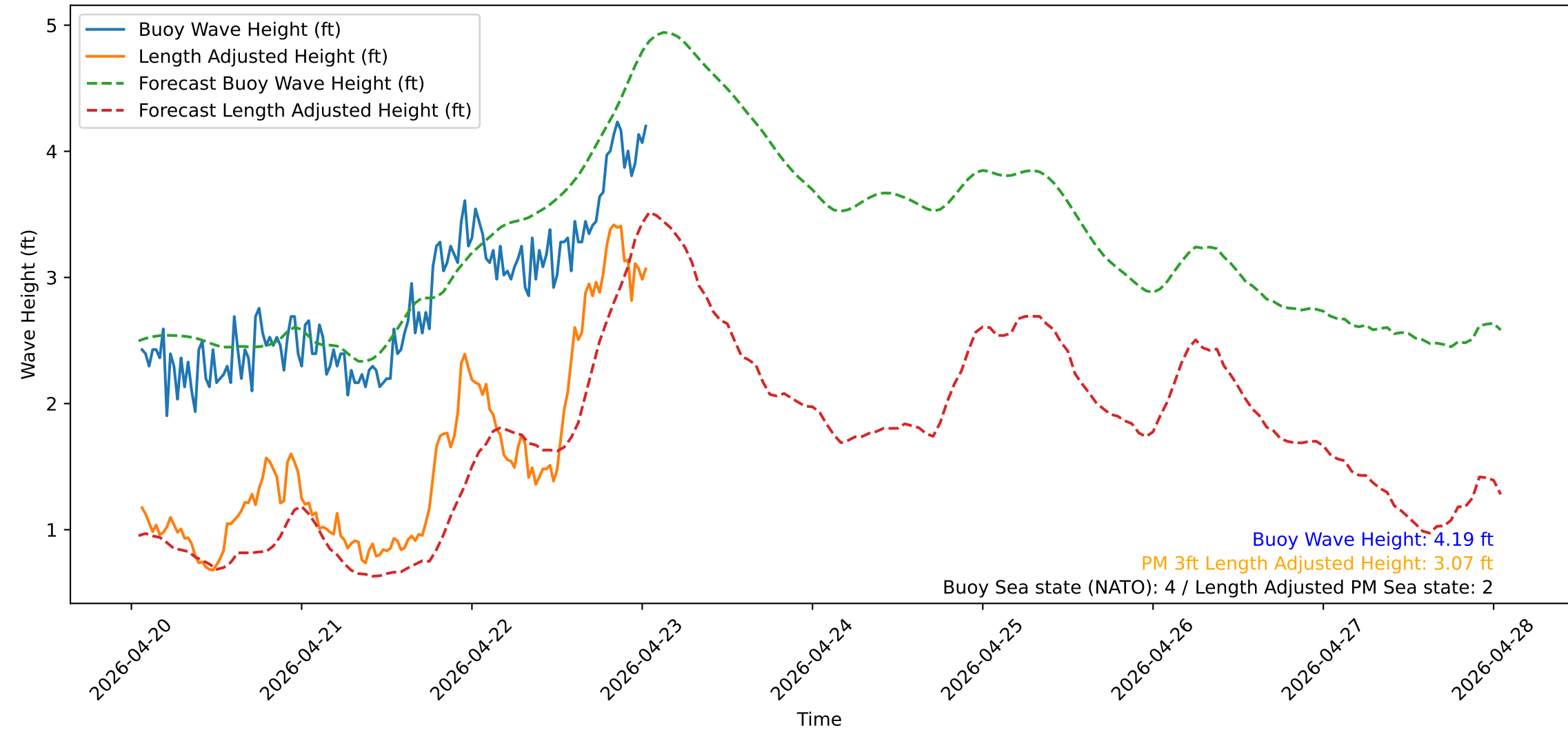
Wave Heights over Time for Oceanside Harbor at 2026-04-23 01:20:31
