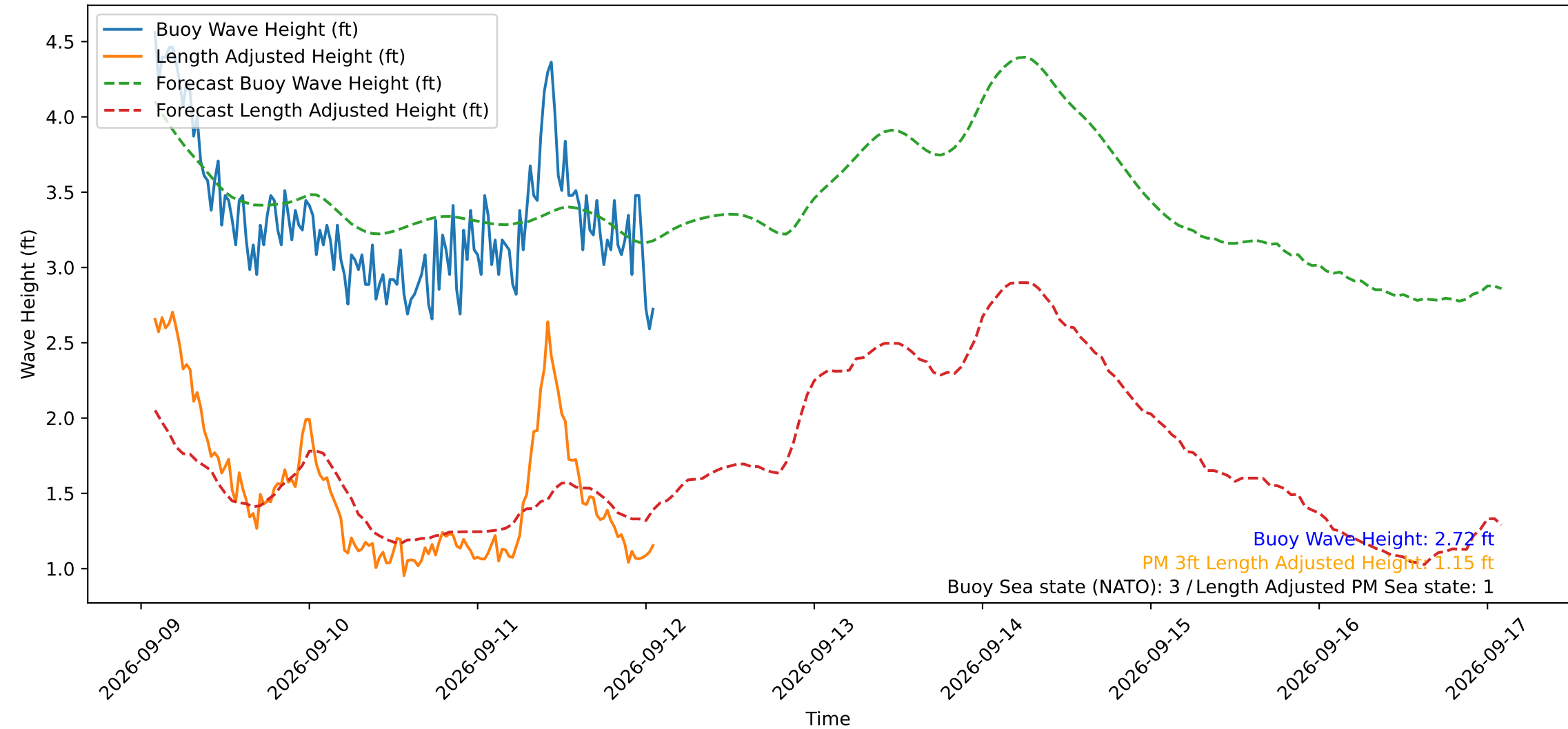
Wave Heights over Time for Oceanside Harbor at 2026-09-12 01:50:30
