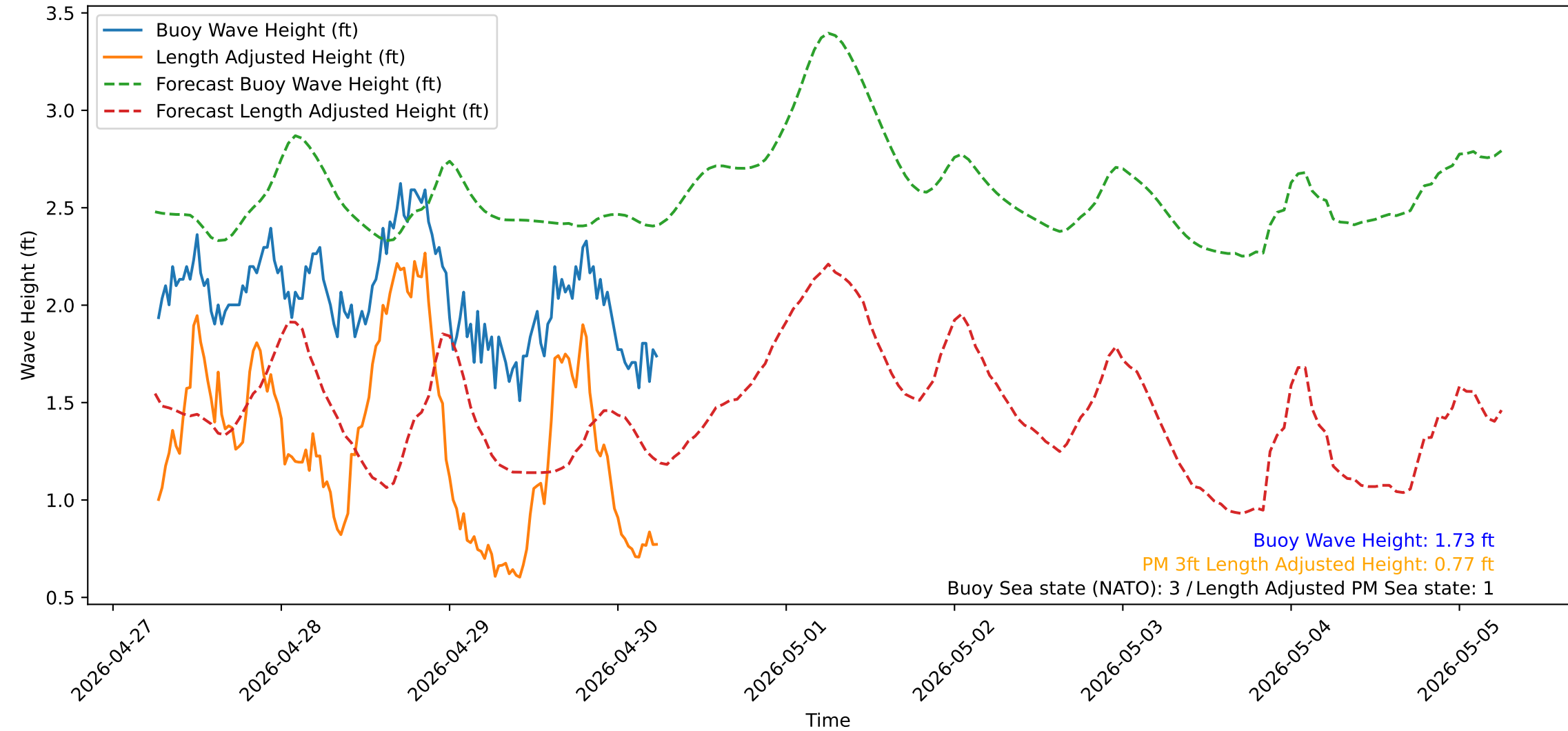
Wave Heights over Time for Red Beach at 2026-04-30 06:10:51
