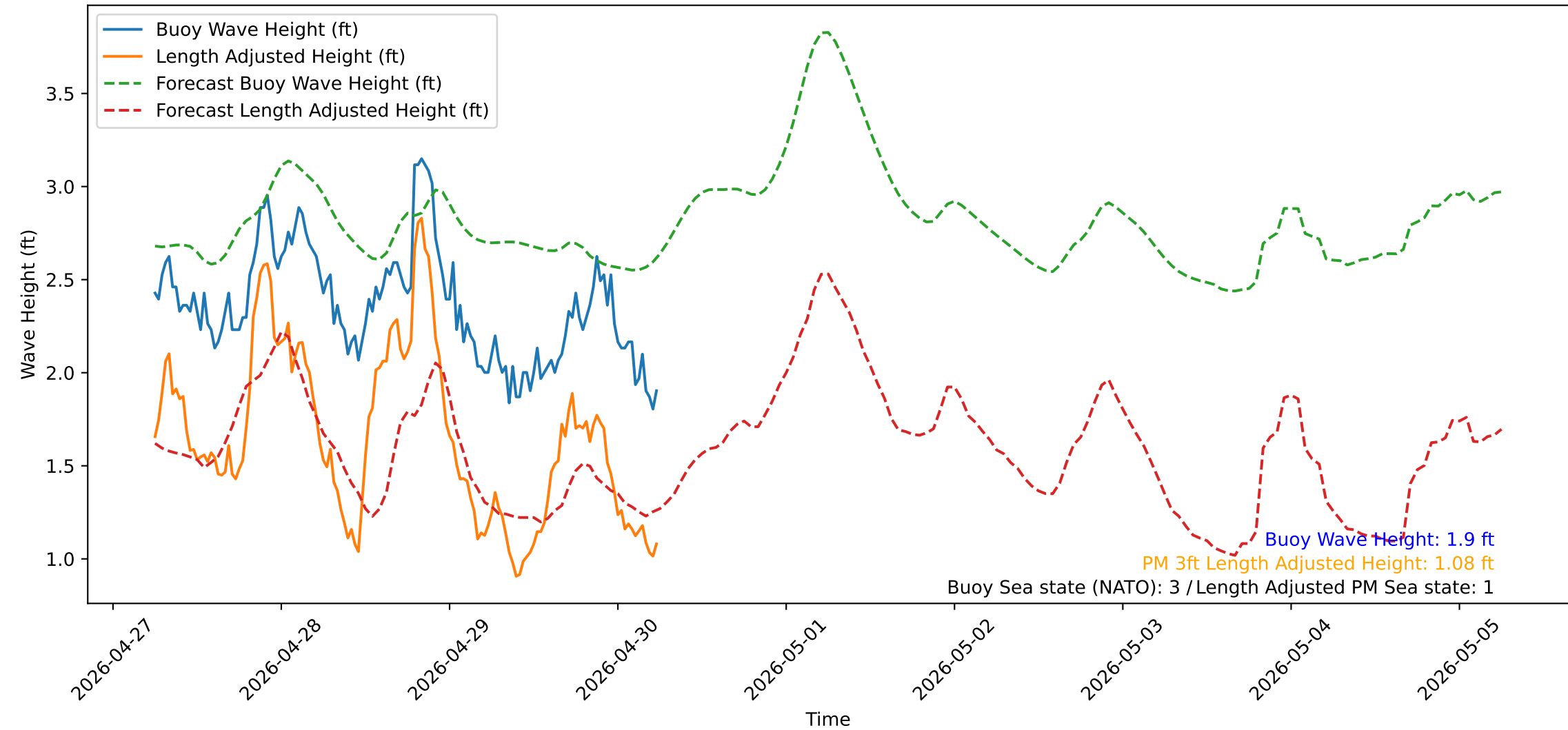
Wave Heights over Time for Green Beach at 2026-04-30 06:11:13
