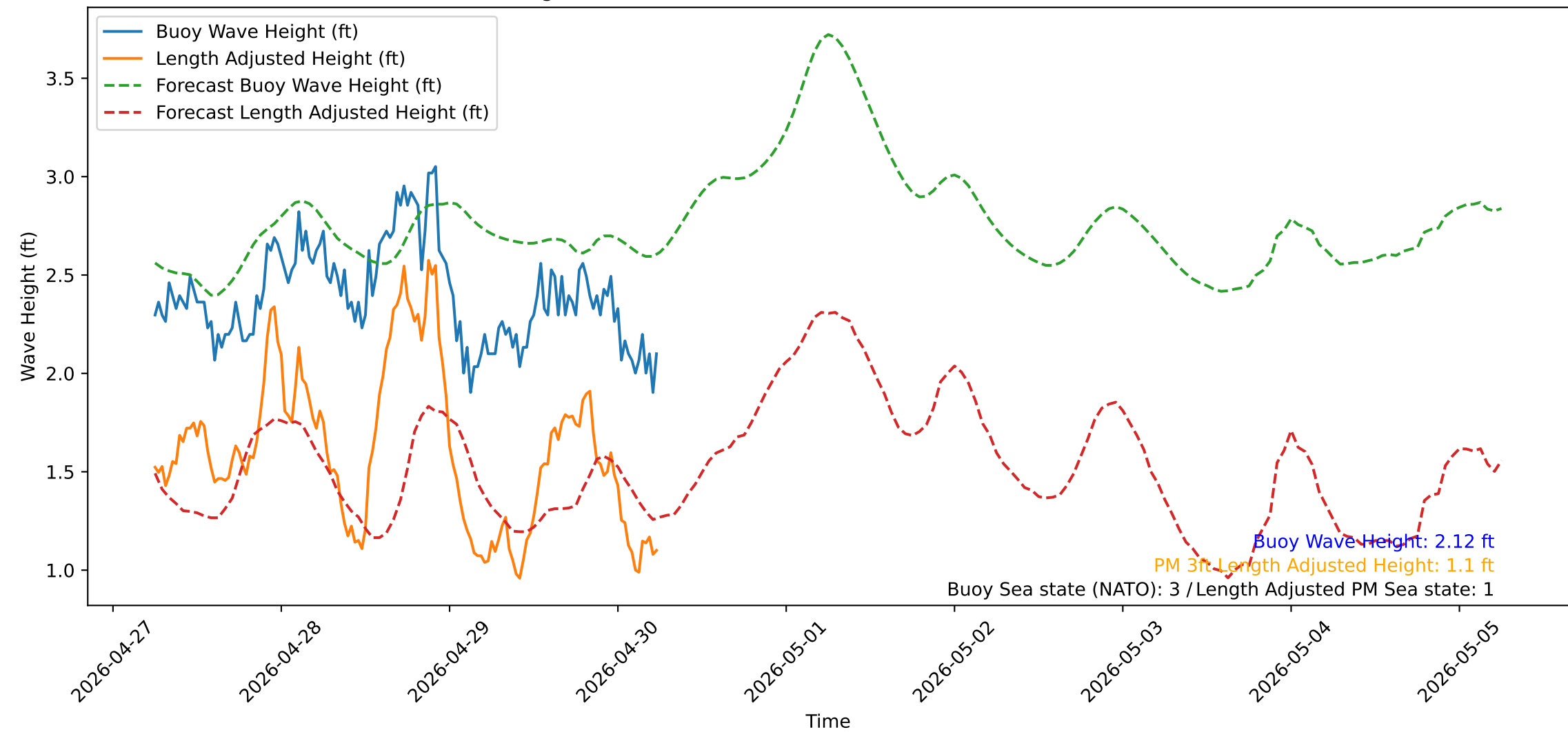
Wave Heights over Time for Oceanside Harbor at 2026-04-30 06:10:31
