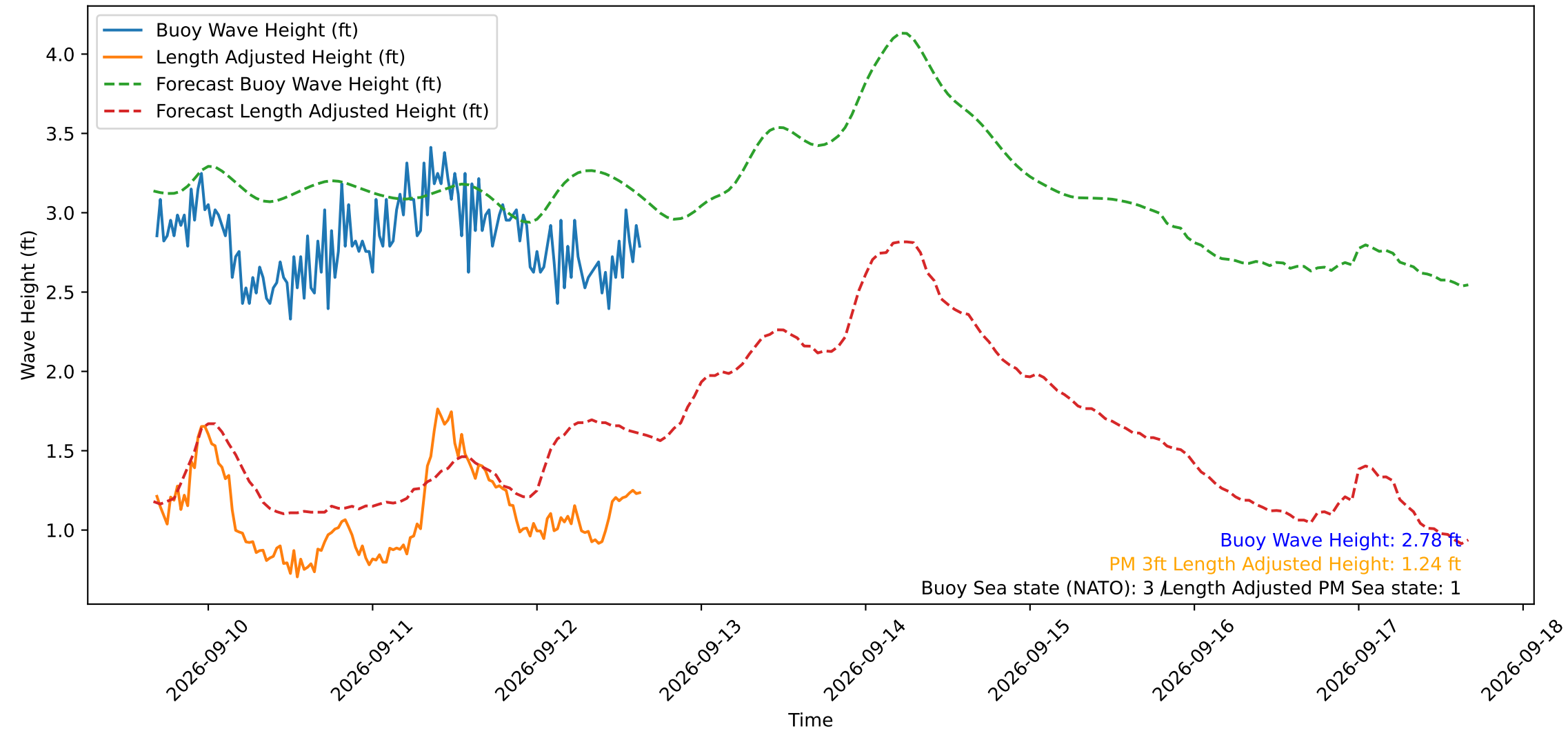
Wave Heights over Time for Red Beach at 2026-09-12 16:00:49
