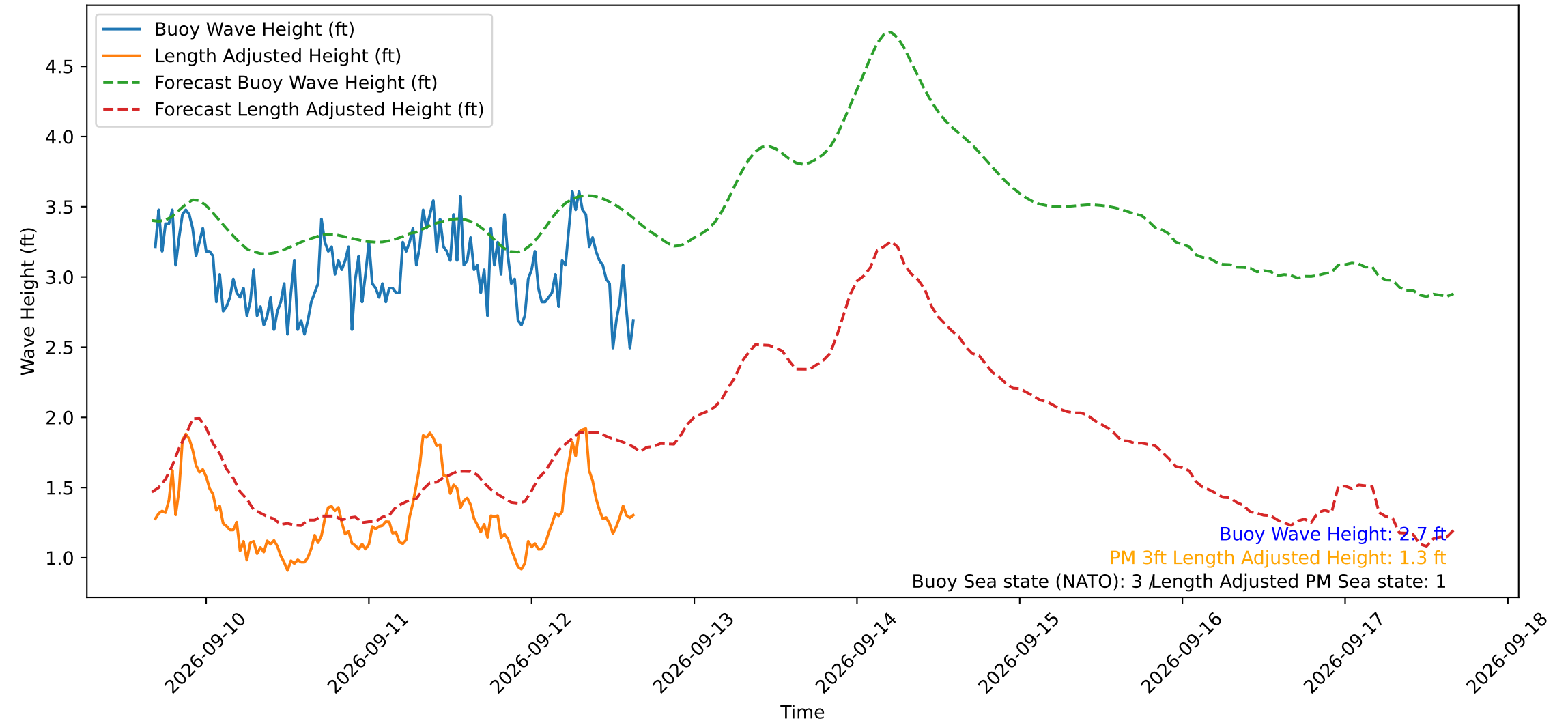
Wave Heights over Time for Green Beach at 2026-09-12 16:01:11
