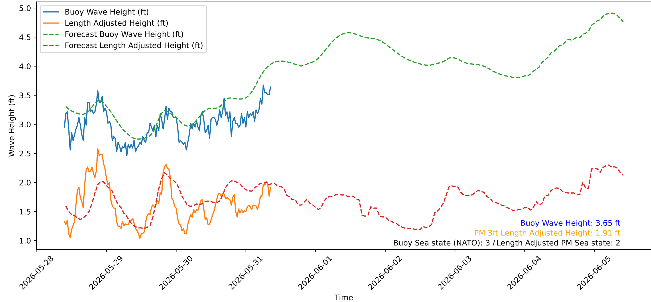
Wave Heights over Time for Green Beach at 2026-05-31 09:31:07
