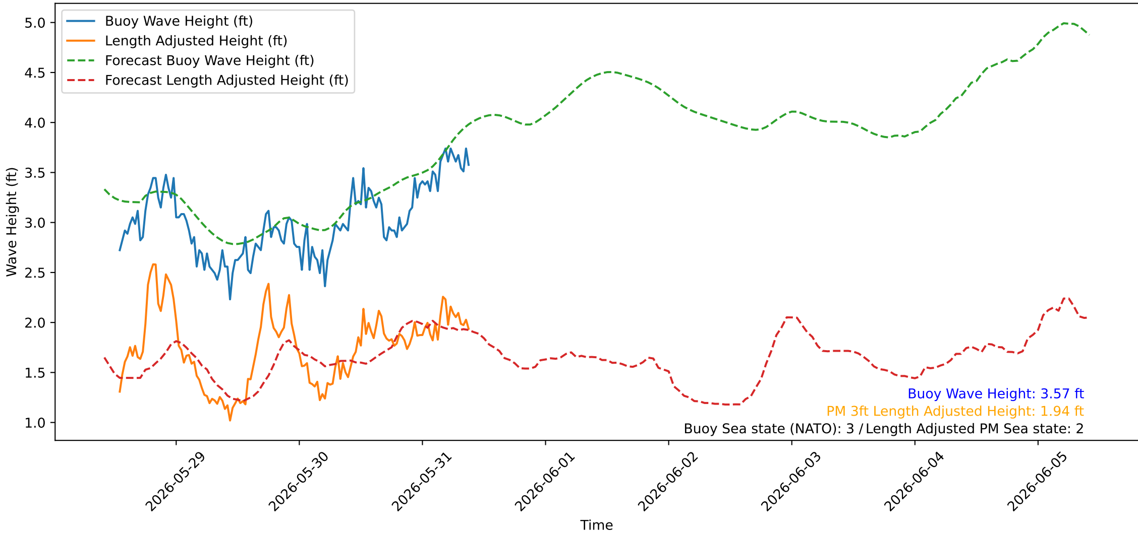
Wave Heights over Time for Oceanside Harbor at 2026-05-31 09:30:26
