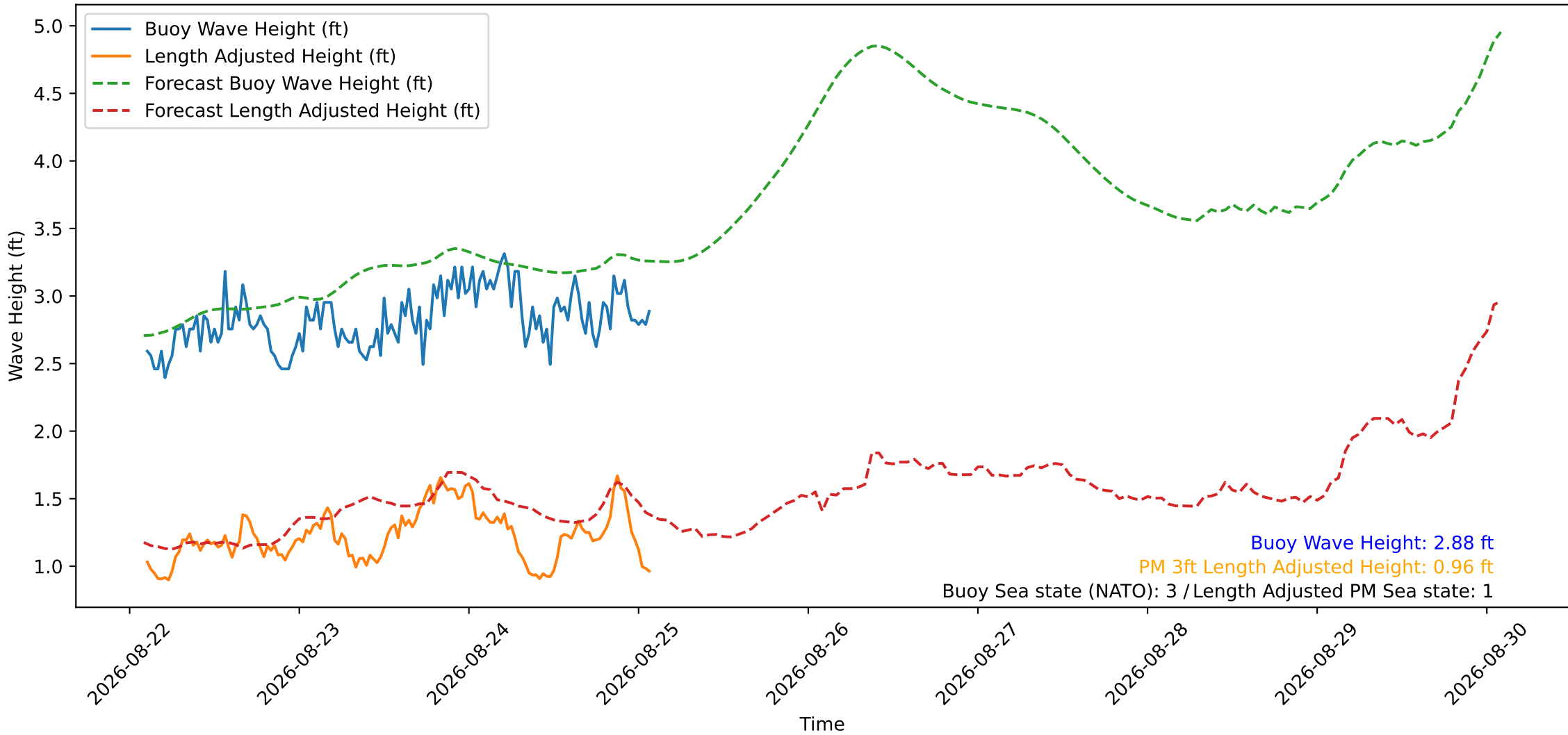
Wave Heights over Time for Green Beach at 2026-08-25 02:21:15
