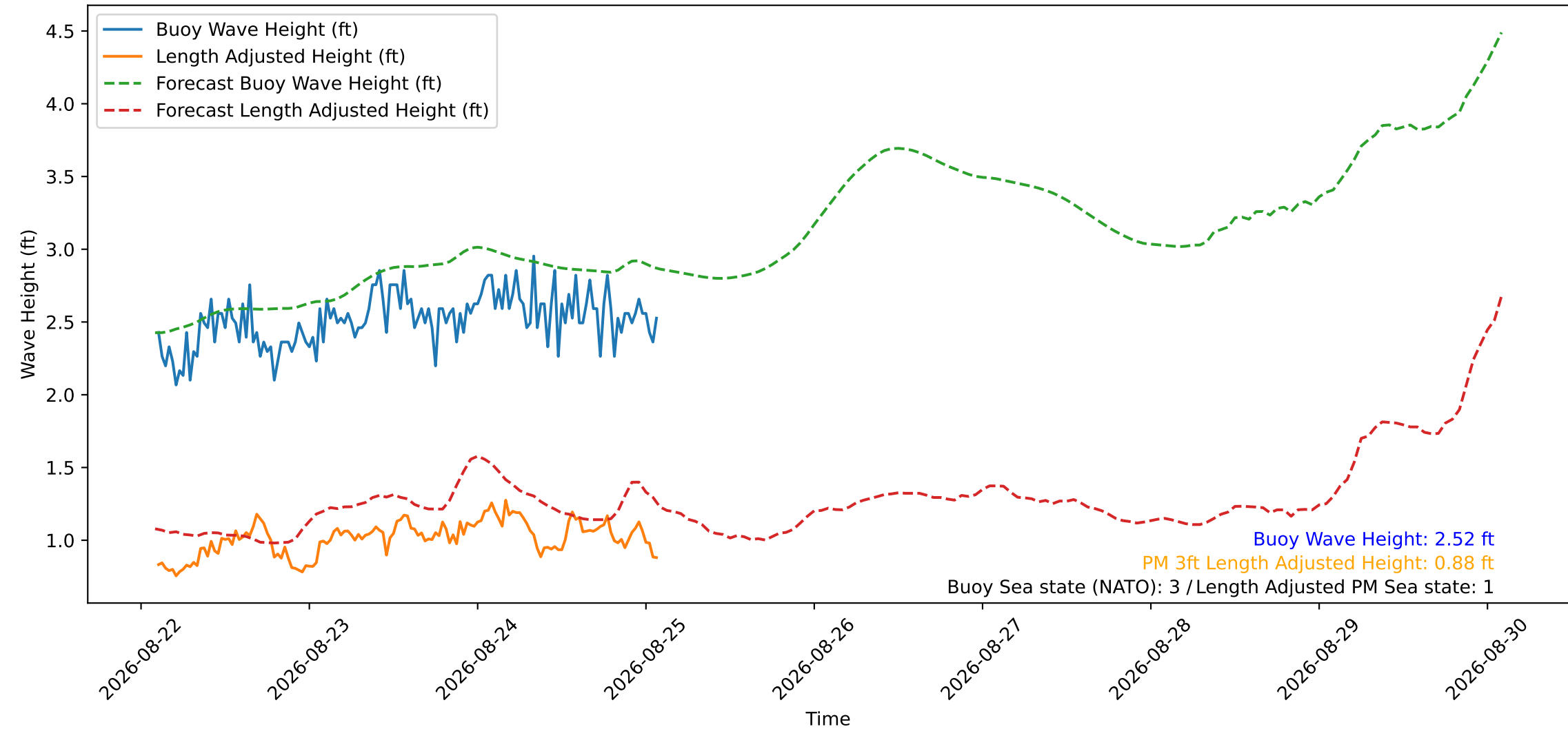
Wave Heights over Time for Red Beach at 2026-08-25 02:20:51
