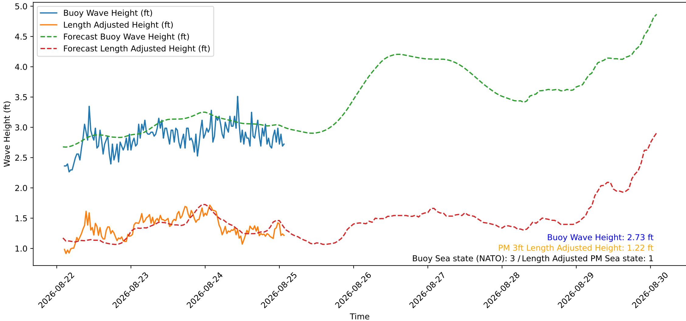
Wave Heights over Time for Oceanside Harbor at 2026-08-25 02:20:30
