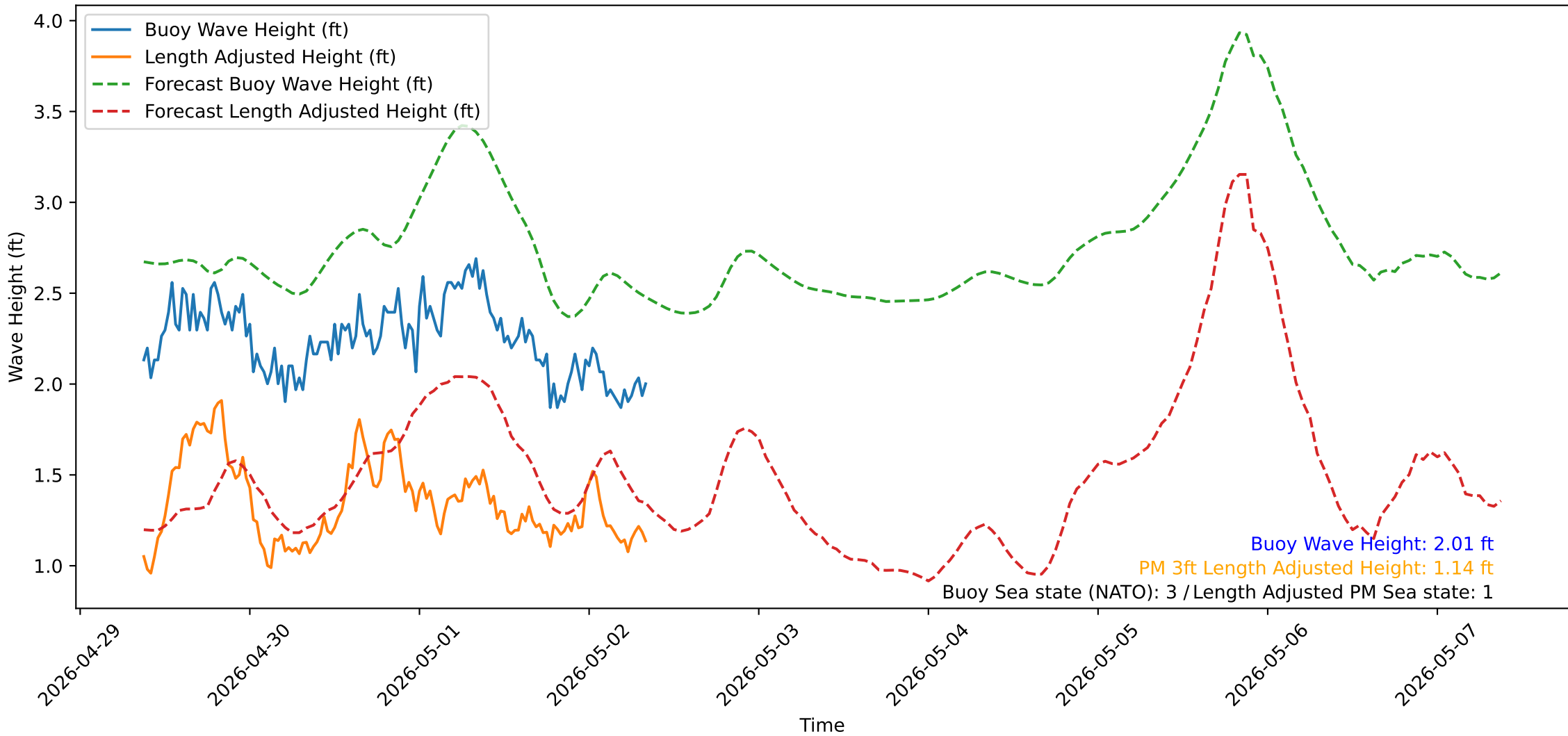
Wave Heights over Time for Oceanside Harbor at 2026-05-02 08:50:32
