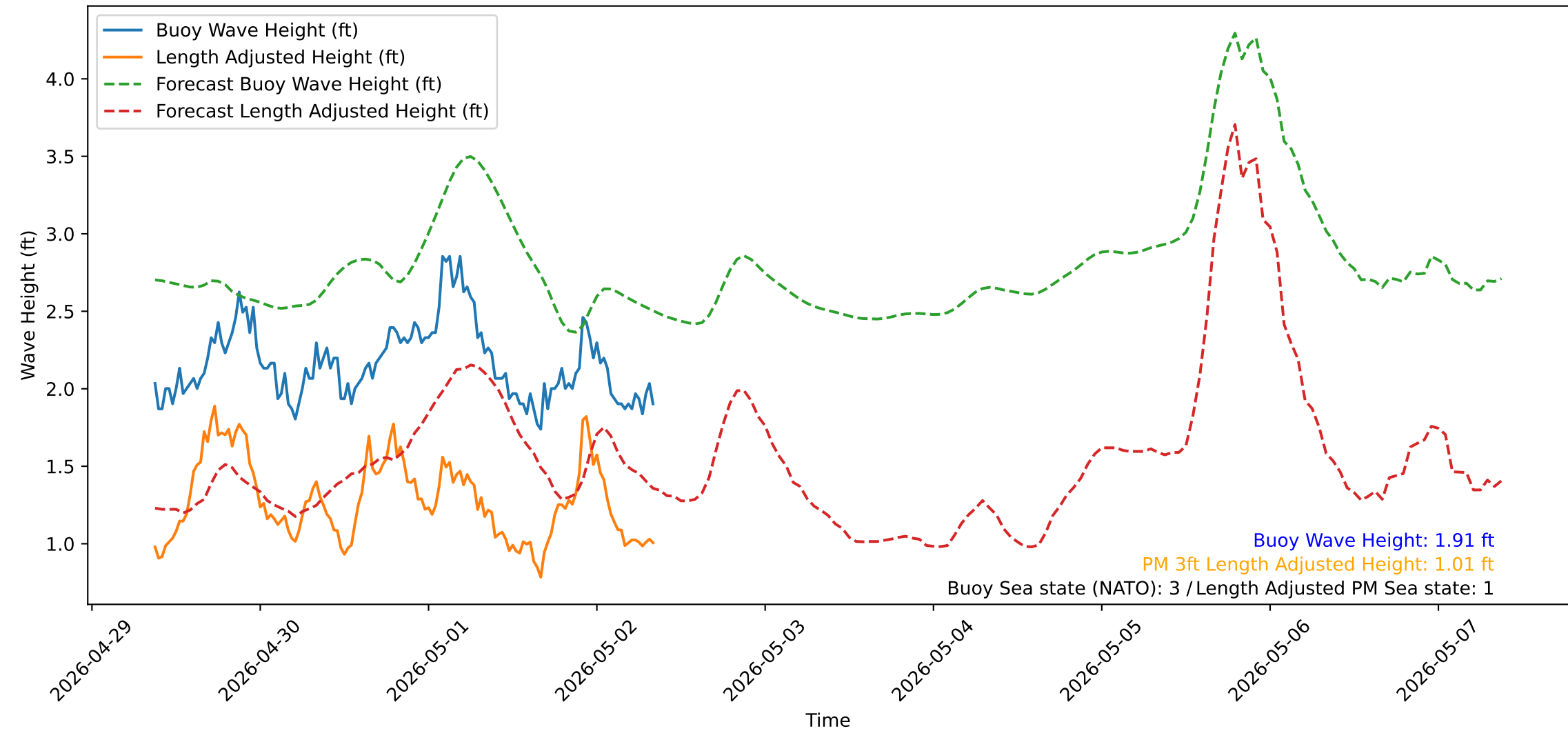
Wave Heights over Time for Green Beach at 2026-05-02 08:51:15
