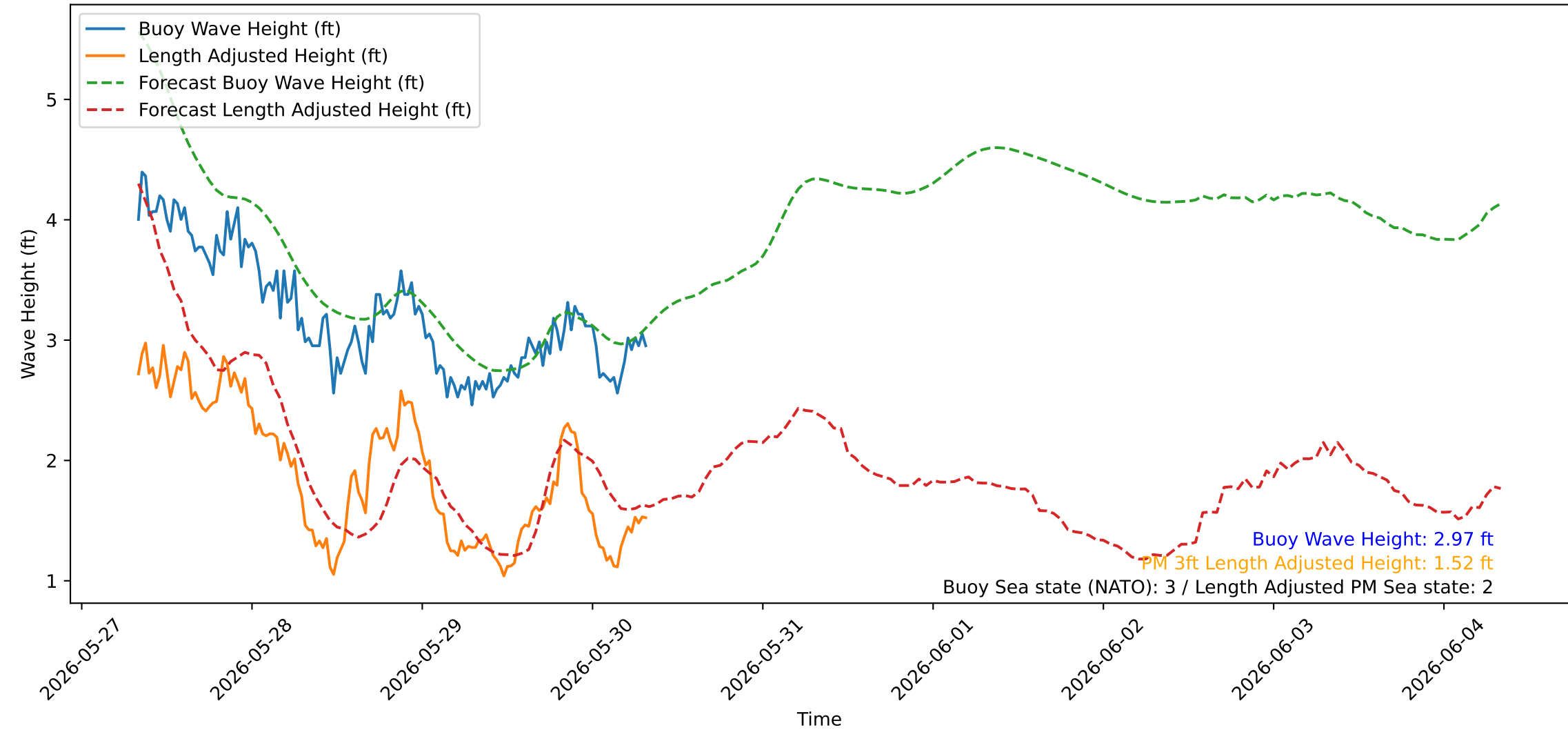
Wave Heights over Time for Green Beach at 2026-05-30 08:11:05
