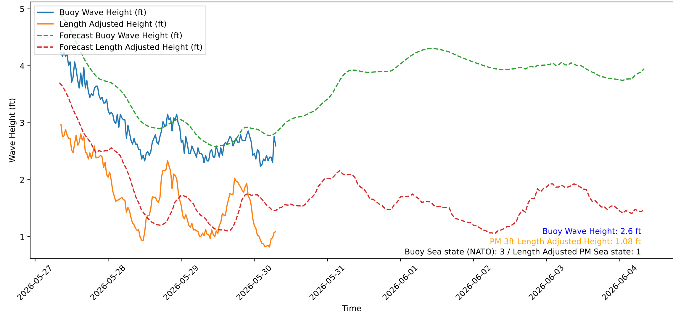
Wave Heights over Time for Red Beach at 2026-05-30 08:10:42
