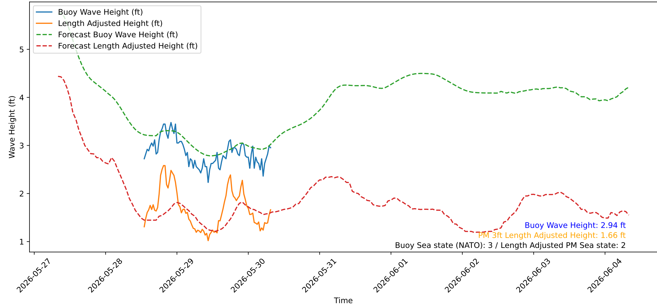
Wave Heights over Time for Oceanside Harbor at 2026-05-30 08:10:23
