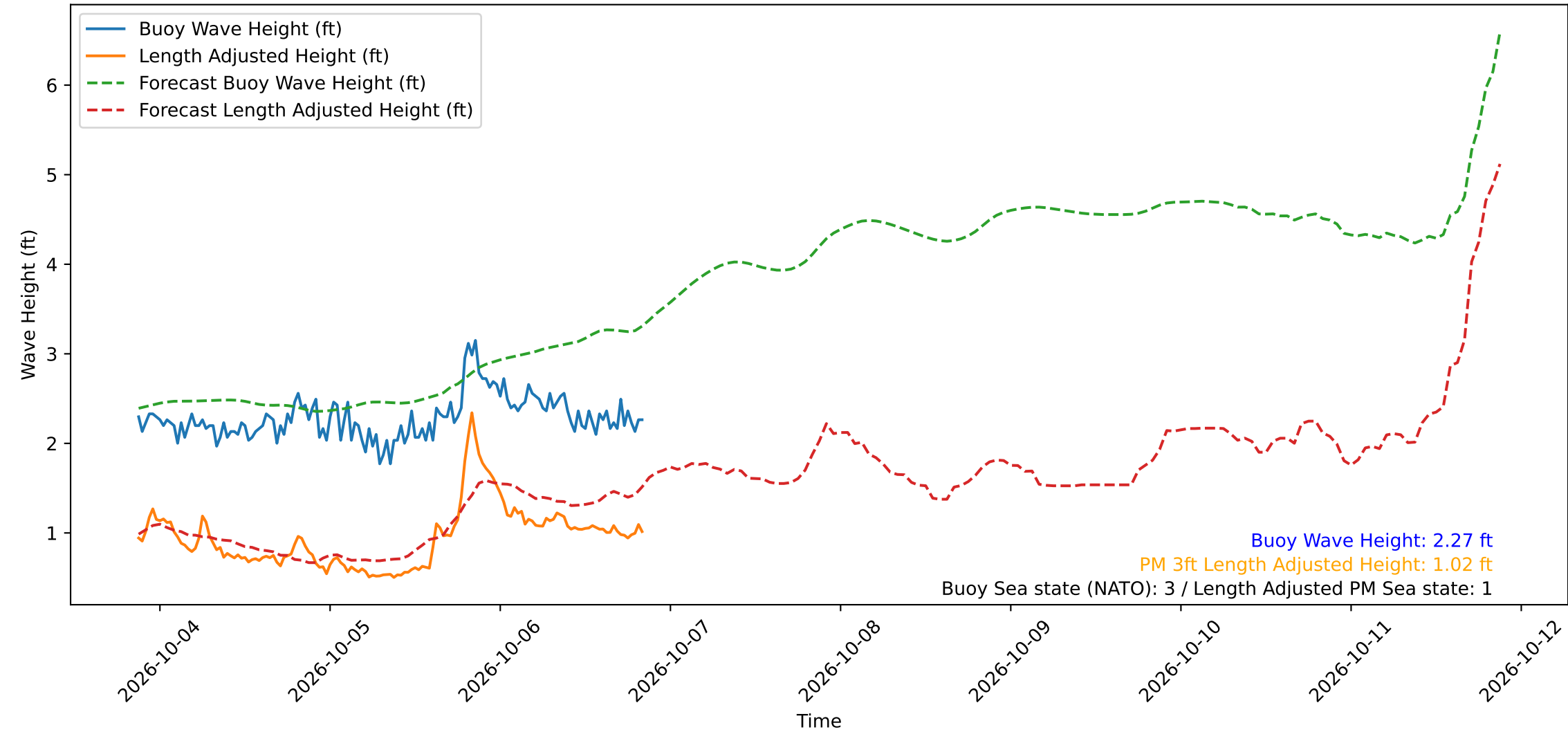
Wave Heights over Time for Green Beach at 2026-10-06 20:41:12
