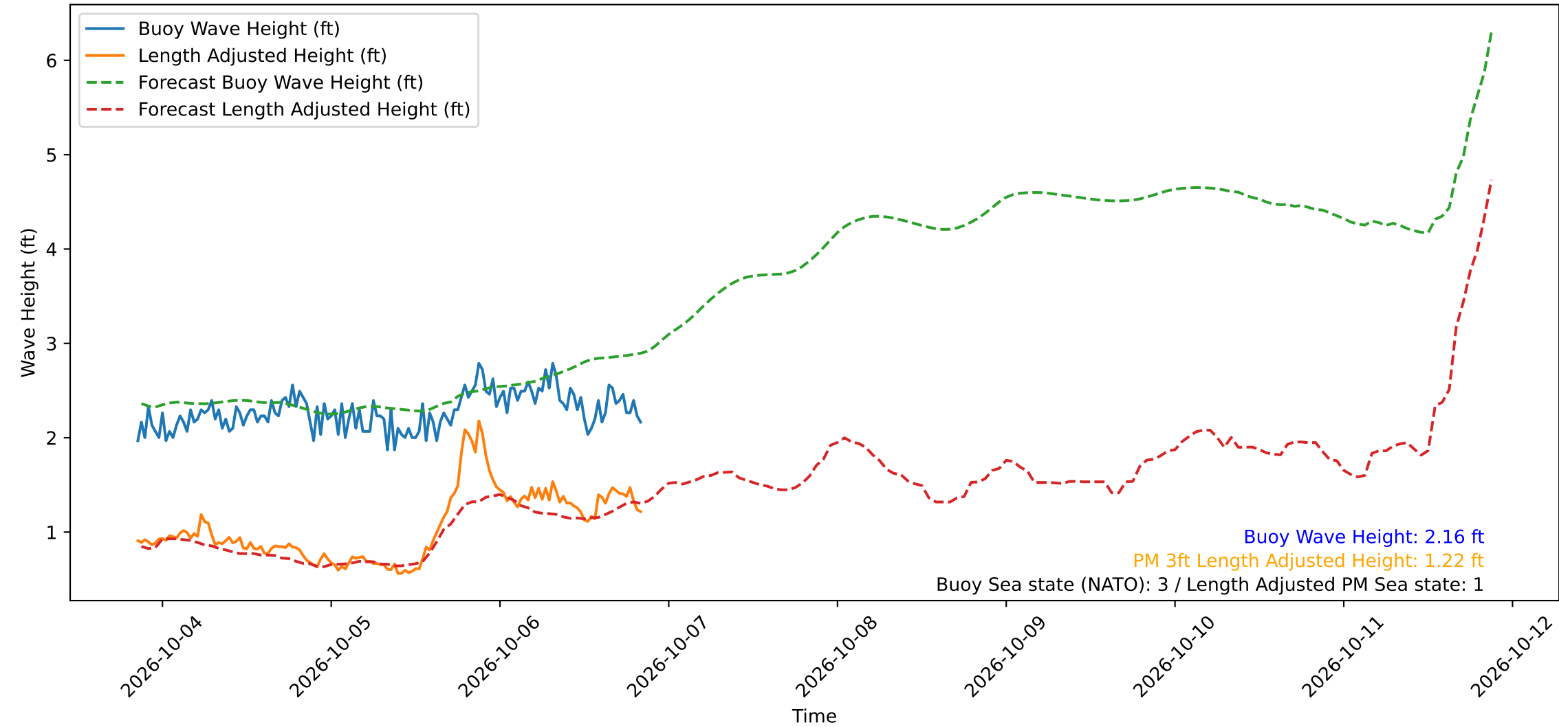
Wave Heights over Time for Oceanside Harbor at 2026-10-06 20:40:30
