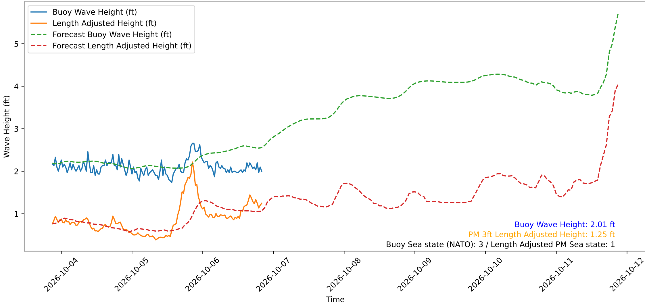
Wave Heights over Time for Red Beach at 2026-10-06 20:40:50
