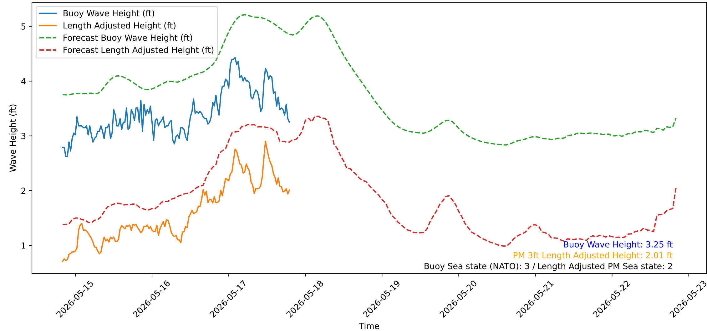
Wave Heights over Time for Green Beach at 2026-05-17 20:01:12
