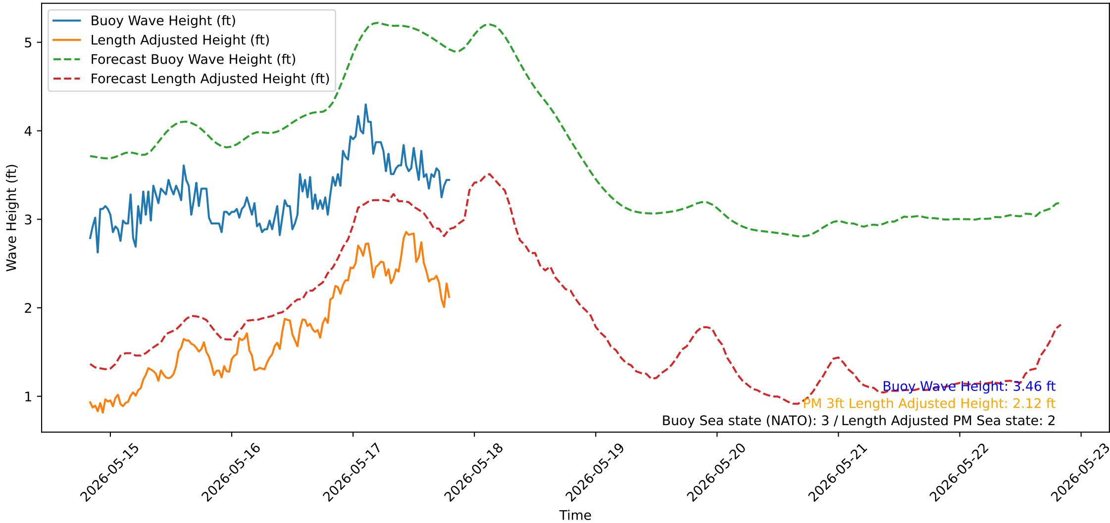
Wave Heights over Time for Oceanside Harbor at 2026-05-17 20:00:31
